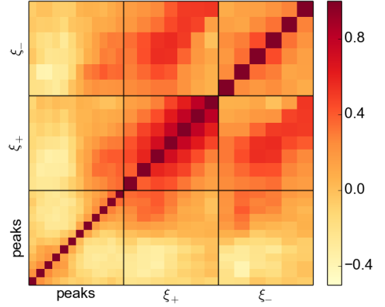
Figure 11. Joint correlation matrix for peaks in the range 0 \leq S/N \leq 4 , \xi_+ , and \xi_- . Each square represents the correlation of one estimator.
