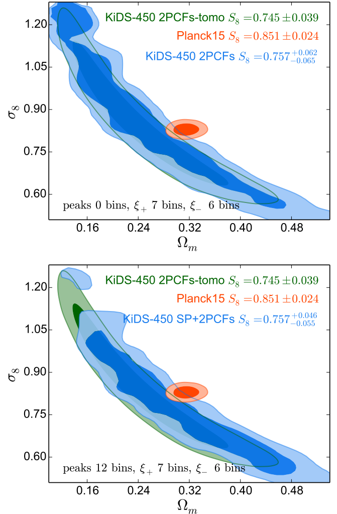
Figure 12. Cosmological constraints on (\Omega_m, \sigma_8) from peaks and 2PCFs. 1\sigma and 2\sigma confidence regions are displayed in dark and light areas respectively. Green contours correspond to KiDS-450 tomographic 2PCFs constraints marginalized over systematics ( Hildebrandt et al. 2017 ), blue to the KiDS-450 2PCFs constraints ( top ), and to the joint peaks in the range 0 \leq S/N \leq 4 and 2PCFs constraints ( bottom ), and red to Planck "TT+lowP" ( Planck Collaboration et al. 2016 ). The top right legend shows the S_8 best value and 68% errors for each study.
