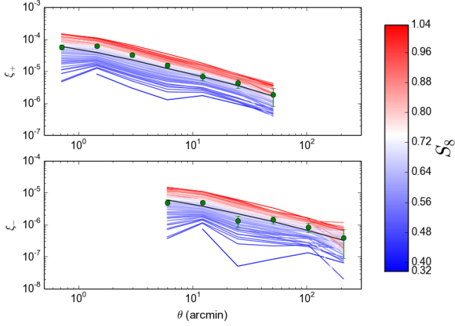
Figure 10. Shear two point correlation functions: \xi_+ (top) and \xi_- (bottom). Green dots represent KiDS data with error bars from the dispersion in the fiducial cosmologies, black line the mean of the fiducial cosmologies, and colored lines the various simulations with S_8 increasing from blue to red.
