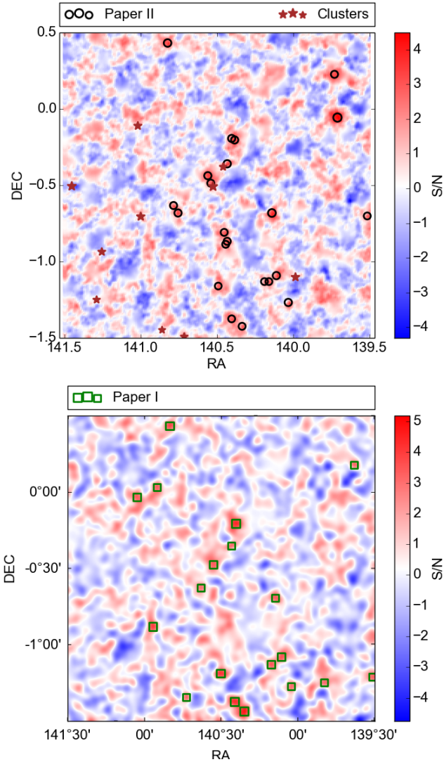
Figure 3. Top: Aperture mass map of a 2 \times 2 square degree field in the KiDS-450 footprint. The S/N of each pixel is color-coded from blue to red, red corresponding to high- M_{\text{ap}} pixels. Black circles represent peaks in this map with S/N \geq 3 , and brown stars indicate galaxy clusters from Radovich et al. (2017) with redshift z \leq 0.5 and detection level \sigma \geq 7 . Bottom: Mass map of the same field computed from the direct shear inversion in Paper I. Green squares correspond to peaks with S/N \geq 3 as detected in Paper I.
