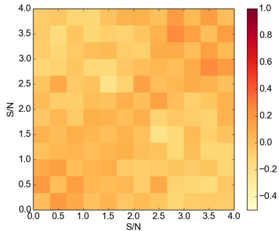
Figure B1. Difference between the fiducial correlation matrix of Fig. 6 and the refined correlation matrix for peaks in the range 0 \leq S/N \leq 4 .
