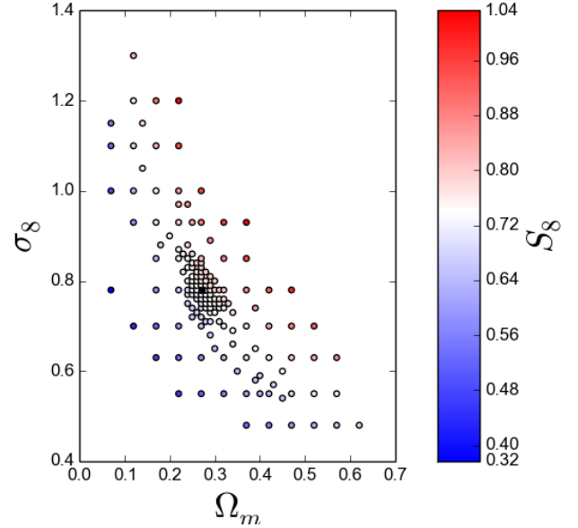
Figure 1. Sampling of the (\Omega_m, \sigma_8) plane. Each dot represents an N-body simulation out of which 5 galaxy catalogs are made. Colors show S_8 = \sigma_8 \sqrt{\Omega_m/0.3} values. The central black dot corresponds to our fiducial cosmology \pi_0 = (0.27, 0.78) , which has 35 N-body simulations and therefore 175 pseudo-independent catalogs.
