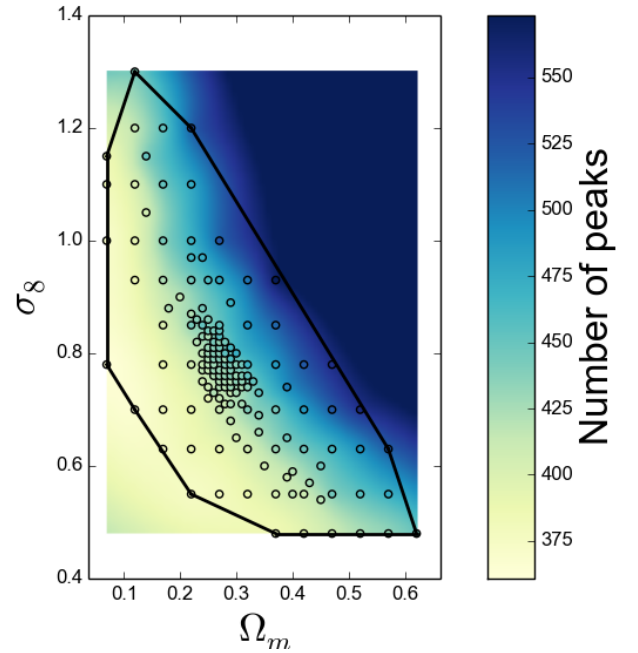
Figure 5. Interpolation of the number of peaks in the bin 3.33 \leq S/N \leq 3.66 . Dots correspond to measured values and the background area to interpolated ones. The black polygon represents the convex hull within which we trust the interpolation. See text for details.
