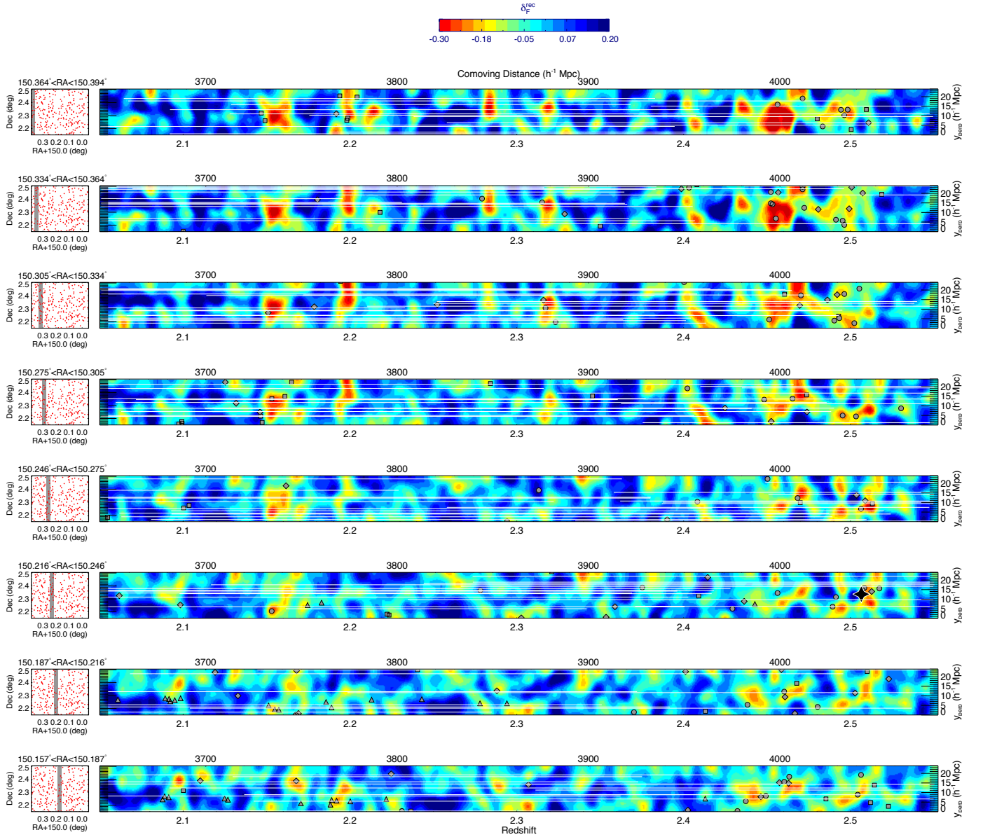
Figure 9. Wiener-filtered tomographic reconstructions of the Ly \alpha forest absorption field, \delta_{F^{\text{ec}}}^{\text{ec}} , at 2.05 < z_{\alpha} < 2.55 from the current CLAMATO data (color map), shown after smoothing with an isotropic R = 2 h^{-1} Mpc Gaussian kernel. Each color panel shows the absorption projected over a 2 h^{-1} Mpc R.A. slice, the position of which is denoted by the shaded region in the subpanels to the left that also show the sightline positions on the sky as red dots. The color convention for the absorption is such that red denotes overdensities while blue denotes underdensities. White horizontal lines denote the sightline coverage, while symbols mark the location of known foreground galaxy redshifts: downwards triangles from MOSDEF, upwards triangles from ZFIRE, squares from VUDS, diamonds from zCOSMOS-Deep, and circles from CLAMATO. The large black stars indicate the reported central positions of the galaxy overdensities at z = [2.10, 2.44, 2.47, 2.51] . This sequence is continued in Figure 10.
