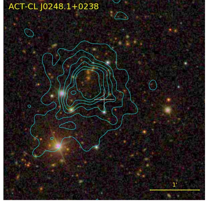
Figure 30. SDSS gri image of the massive cluster ACT-CL J0248.1+0238 ( z = 0.556 ), with contours showing the extended X-ray emission detected by Chandra (arbitrary levels; smoothed at 5'' scale). The cluster is morphologically disturbed, and has a high X-ray temperature ( T = 8.4^{+1.4}_{-1.0} \text{ keV} ). The image is 4' on a side, with North at the top and East at the left. The white cross marks the SZ cluster position.
