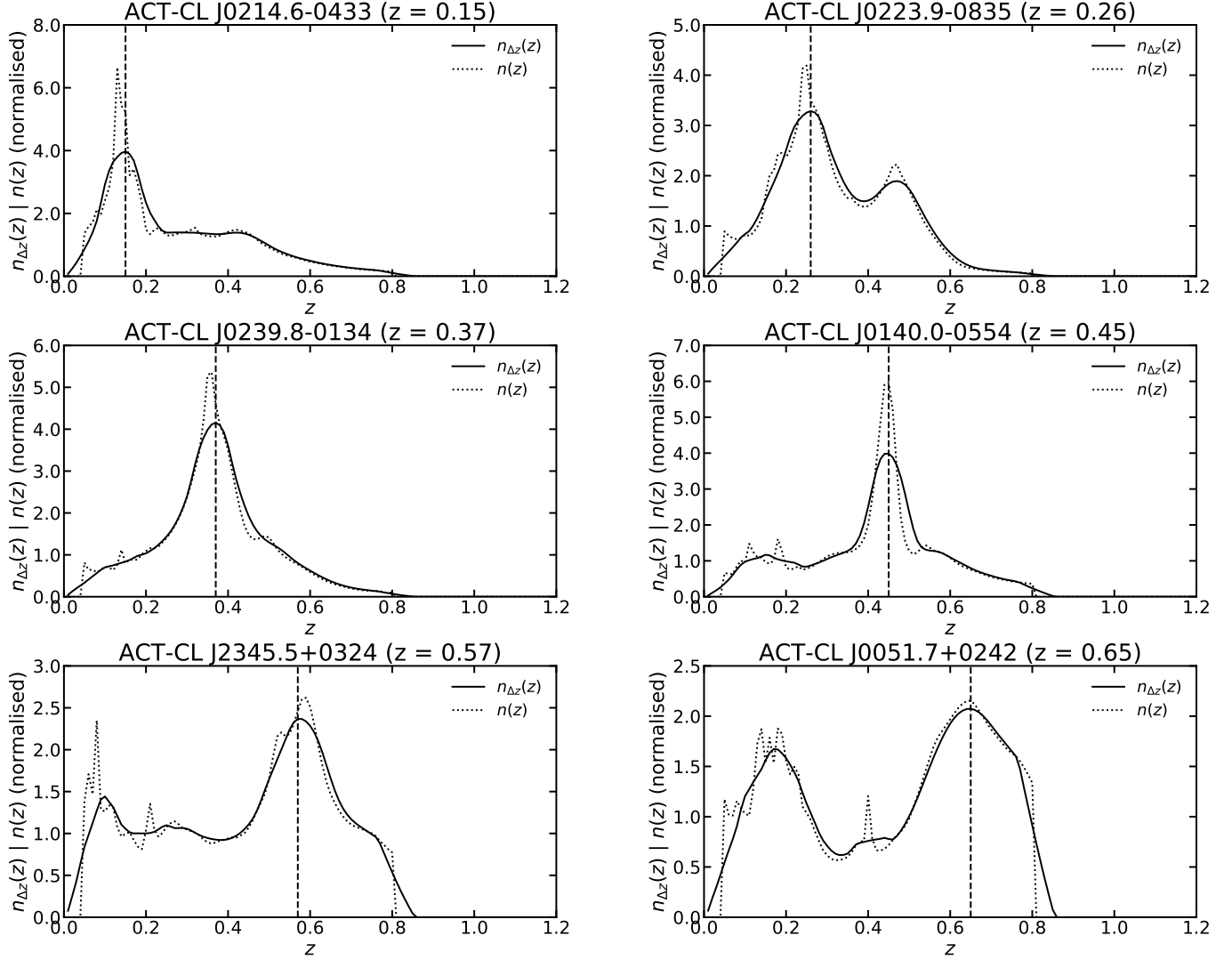
Figure 12. Examples of normalized n(z) and n_{\Delta z}(z) distributions for several clusters at different redshifts (based on SDSS photometry), measured within 1 Mpc projected radial distance. In some cases, multiple peaks are seen; we adopt the maximum of n_{\Delta z}(z) as the cluster photometric redshift (shown as the vertical dashed line). Optical images corresponding to each of the clusters shown here can be found in Fig. 13.
