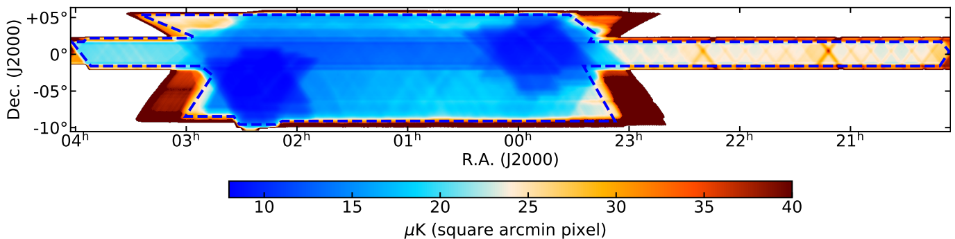
Figure 2. The white noise level ( \mu\text{K} per square arcmin pixel) across the inverse-variance weighted combination of the ACT equatorial and ACTPol maps (E-D56). The variation in the noise level in this map reflects the scan strategy. The cluster search was conducted within the area bounded by the blue dashed line. The deepest regions are the D5 and D6 fields (Naess et al. 2014; Louis et al. 2017), located at approximately 23^{\text{h}}30^{\text{m}} and 02^{\text{h}}30^{\text{m}} respectively.
