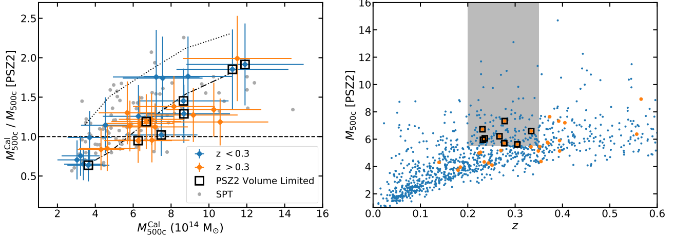
Figure 26. Left panel: Comparison of the ratio of PSZ2 masses (Planck Collaboration et al. 2016a) to the ACTPol UPP-based masses, re-scaled using the richness-based weak-lensing mass calibration ( M_{500c}^{\text{Cal}} ; Section 6.1). Clearly there is a mass-dependent trend, with ACTPol mass estimates being progressively larger than PSZ2 with mass, which persists when the sample is split by redshift. The Bleem et al. (2015) SPT catalog, cross-matched with PSZ2 using a 10' matching radius, follows a similar trend (gray points). The dotted (dot-dashed) line shows the limit obtained by assigning masses at the 2\sigma ( 5\sigma ) PSZ2 detection threshold to clusters that were detected by ACTPol but not PSZ2, averaged in M_{500c} bins (see the text). Right panel: The distribution of the whole PSZ2 catalog in the mass, redshift plane (small blue points). Clusters that are detected by both ACTPol and Planck are shown as the larger yellow points. The shaded area shows a volume-limited sample defined by 0.2 < z < 0.35 and M_{500c} [\text{PSZ2}] > 5.5 \times 10^{14} M_{\odot} . The 8 clusters in this region, detected by both ACT and Planck , are highlighted in both panels by black squares. The lower redshift limit accounts for the fact that z < 0.2 clusters are underrepresented in the ACTPol sample (see Fig. 10).
