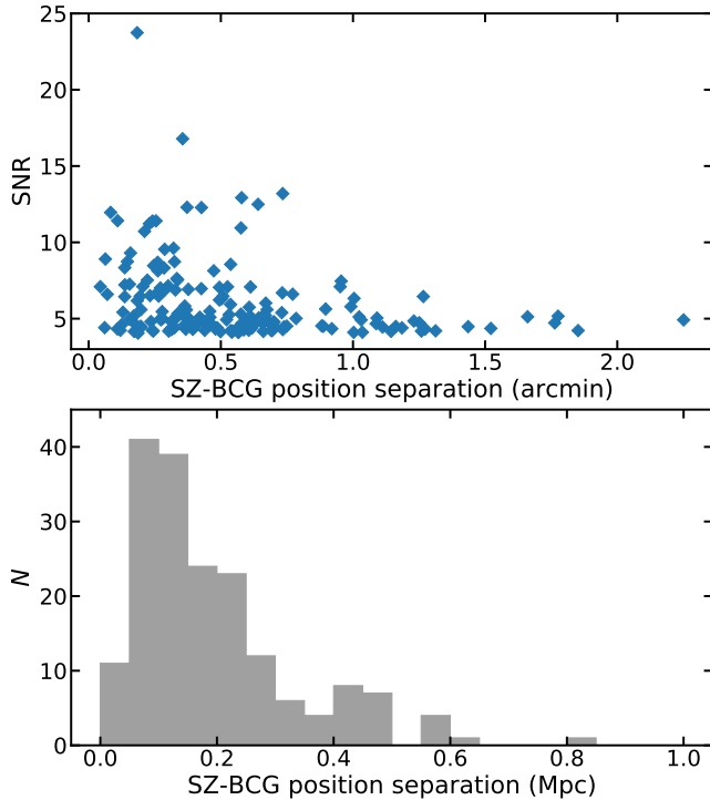
Figure 21. The separation between BCG positions and the position at which each cluster was detected via the SZ. The top panel shows this in terms of arcminutes as a function of SNR, while the bottom panel shows the distribution in terms of projected radial distance. The typical offset is < 150 kpc.
