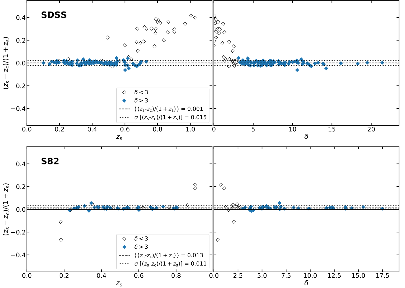
Figure 15. Accuracy of photometric redshift recovery by zCluster, using SDSS (top) and S82 (bottom) data. Each data point represents a cluster in the E-D56 field with a spectroscopic redshift ( z_s ). The difference between the zCluster photometric redshift ( z_c ) and the cluster spectroscopic redshift is plotted on the vertical axis. Clusters with low density contrast ( \delta < 3 ; equation 4), as measured at the photometric redshift, are shown as open diamonds. In the top panels, most of these objects are clusters with z_s > 0.5 , which is beyond the typical reach of SDSS photometry. As a result, their assigned photometric redshifts are spurious, but are flagged by the \delta < 3 cut. For clusters with \delta > 3 , z_c is unbiased when using SDSS photometry, and has small scatter. However, as shown in the bottom panel, the photometric redshifts are underestimated by \Delta z/(1+z) = 0.013 , when using S82 photometry.
