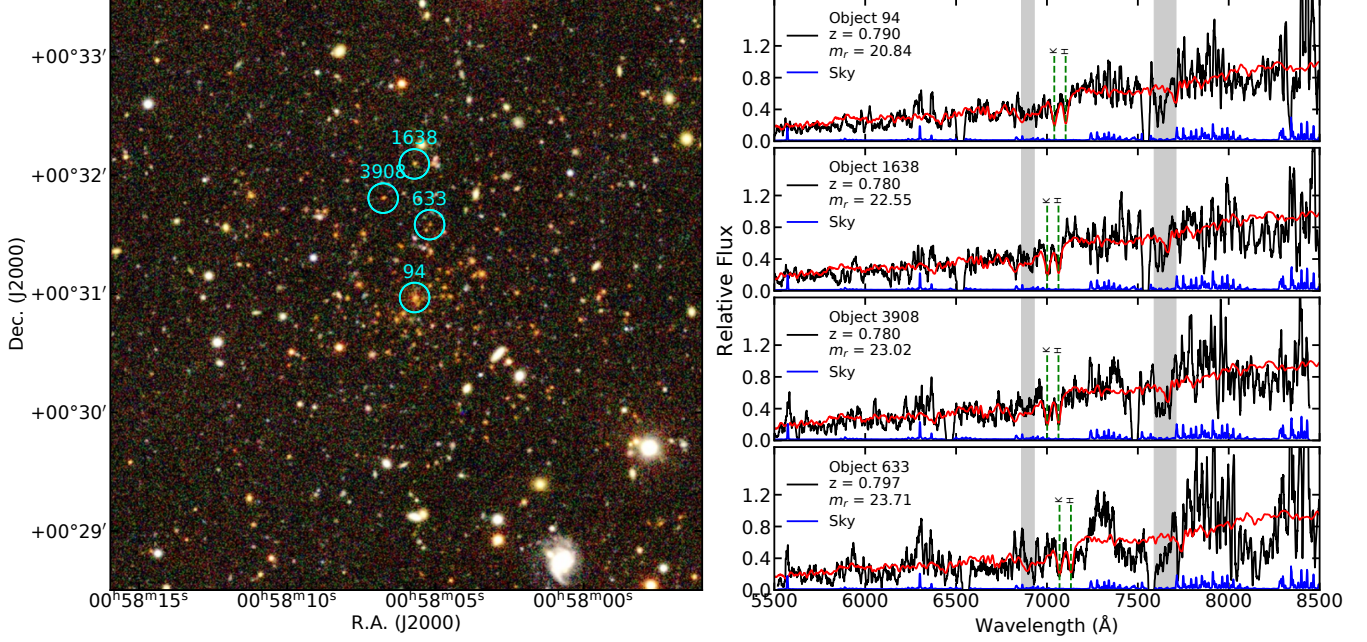
Figure 17. The z = 0.79 cluster ACT-CL J0058.1 + 0031. Secure spectroscopic redshifts have been obtained for 7 member galaxies in this cluster. The left hand panel shows a 5' \times 5' false color S82 optical image ( g, r, i ). SALT spectra for the four galaxies highlighted by the cyan circles are shown in the right hand panel. Here, the black lines are the SALT RSS spectra (smoothed with a 15 pixel boxcar), while red lines show the best match redshifted SDSS spectral template in each case. The blue line is the sky spectrum, and the gray bands indicate regions strongly affected by absorption features in the atmosphere.
