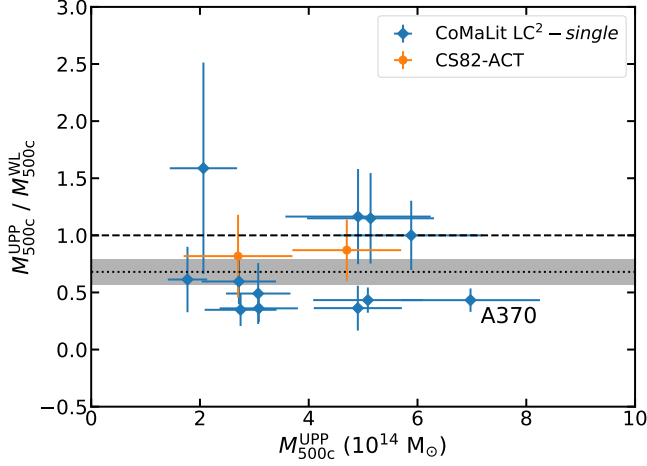
Figure 23. Comparison of weak-lensing masses from the CoMaLit database (Sereno 2015, blue) and the stacked weak-lensing analysis of Battaglia et al. (CS82-ACT; 2016, orange) with ACTPol SZ masses based on the UPP and A10 mass-scaling relation. The CS82-ACT masses plotted here are from NFW profile fits to the stacked weak-lensing signal. Here we used the LC^2 -single catalog from CoMaLit, which consists of objects modeled using a single halo. The dotted line and shaded area indicates the richness-based weak-lensing mass calibration factor and its uncertainty ( 0.68 \pm 0.11 ), obtained independently from these data by applying the Simet et al. (2017) scaling relation to ACTPol clusters cross matched with the redMaPPer catalog (see Section 6.1).
