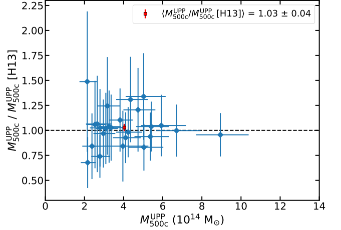
Figure 8. End-to-end test of M_{500c} recovery, comparing clusters cross-matched with H13 ( 2.5' matching radius) with M_{500c} values inferred from SZ decrement measurements made on D56 maps containing only ACTPol data, filtered at the \theta_{500c} = 2.4' scale (this work). The data sets used for this test have independent detector noise. The red square marks the unweighted mean ratio ( \pm standard error) between the two sets of measurements. This test assumes that clusters are described by both the UPP and the A10 mass-scaling relation.
