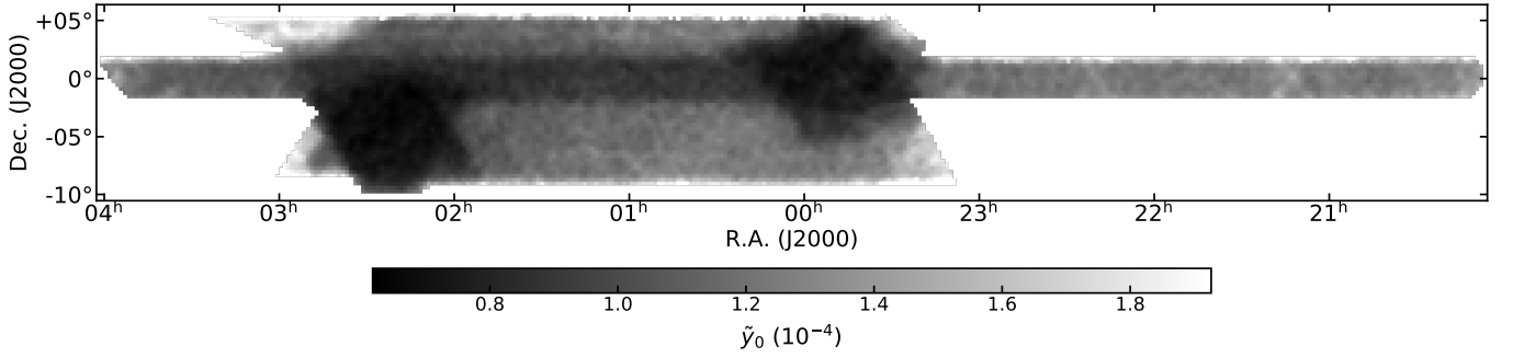
Figure 9. Map of the \tilde{y}_0 -limit corresponding to \text{SNR}_{2.4} = 5 across the ACTPol E-D56 field. In addition to capturing the variation in the white noise level caused by the ACT scan strategy, noise on 20' scales from the CMB and Galactic dust emission is also visible.
