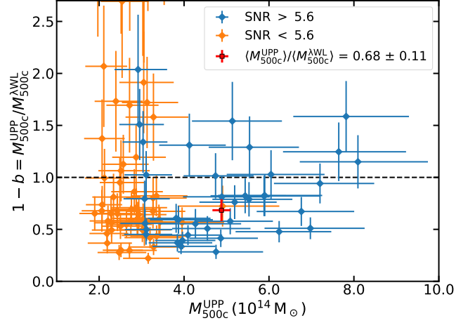
Figure 24. Comparison of richness-based weak-lensing masses ( M_{500c}^{\lambda WL} ), derived from applying the Simet et al. (2017) scaling relation to ACTPol clusters in common with redMaPPer, with ACTPol UPP/A10 SZ masses. The red square marks the ratio \langle M_{500c}^{UPP} \rangle / \langle M_{500c}^{\lambda WL} \rangle = 0.68 \pm 0.11 for the SNR > 5.6 subsample, which is complete at z < 0.6 . The effect of a Malmquist-type bias in the SZ selection can be seen on the clusters with SNR < 5.6 , many of which have SNR close to the detection threshold.
