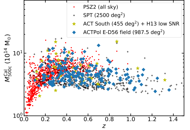
Figure 27. Comparison of the ACTPol E-D56 cluster sample in the (mass, redshift) plane with other blind SZ surveys: SPT (Bleem et al. 2015), and PSZ2 (Planck Collaboration et al. 2016a). Additional clusters from the southern ACT field (Marriage et al. 2011; 23 objects) and equatorial clusters that were masked/not detected in the E-D56 field with \text{SNR} > 4 (Table A4; 15 objects) are shown as yellow stars, using the masses and redshifts as listed in H13. Here, all the ACT SZ masses have been re-scaled according to a richness-based weak-lensing mass calibration (Section 6.1). The SPT and PSZ2 mass measurements are as reported in Bleem et al. (2015) and Planck Collaboration et al. (2016a) respectively (see Section 6.2).
