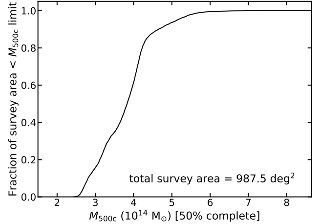
Figure 11. Fraction of the survey area as a function of M_{500c} 50% completeness limit, averaged over the redshift range 0.2 < z < 1 , as assessed from inserting UPP-model clusters into the E-D56 map, filtering at the \theta_{500c} = 2.4' scale, applying a cut of \text{SNR}_{2.4} > 5 , and assuming the A10 mass scaling relation.
