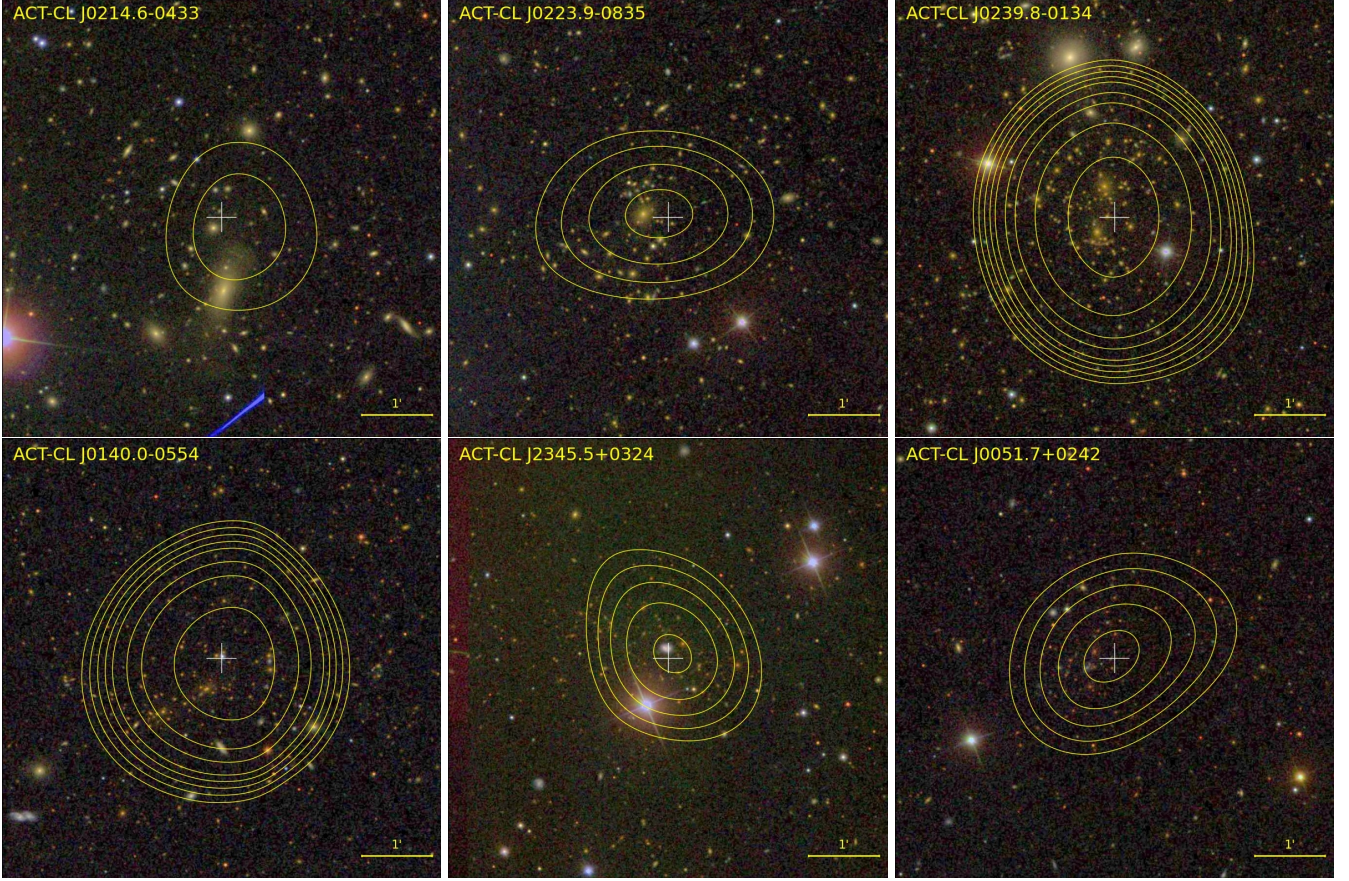
Figure 13. Example optical gri images of clusters confirmed in SDSS (these objects correspond to those shown in Fig. 12). Each image is 6' on a side, with North at the top and East at the left. The yellow contours (minimum 3\sigma , increasing in steps of 0.5\sigma up to \text{SNR} = 5 , and then by 1-2\sigma thereafter) indicate the (smoothed) 148 GHz decrement in the matched-filtered ACT map. The white cross indicates the ACT SZ cluster position. Note that ACT-CL J0051.7+0242 is a newly discovered cluster.
