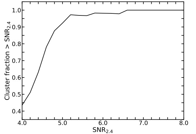
Figure 19. The cumulative fraction of candidates that are confirmed clusters as a function of \text{SNR}_{2.4} . For \text{SNR}_{2.4} > 5 , the fraction is less than 1 because of incomplete redshift follow-up; there is evidence from e.g., WISE imaging that these candidates are likely to be high-redshift ( z > 1 ) clusters. At \text{SNR}_{2.4} < 5 , the dominant effect is sample impurity (see Fig. 5).
