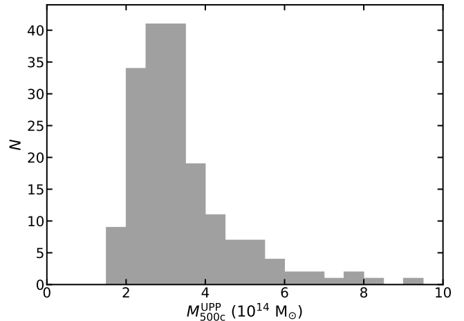
Figure 22. The mass distribution of the 182 clusters in E-D56 cluster catalog (median M_{500c}^{\text{UPP}} = 3.1 \times 10^{14} M_{\odot} ), estimated from the central Compton parameter \tilde{y}_0 measured at the 2.4' filter scale, assuming the A10 scaling relation.
