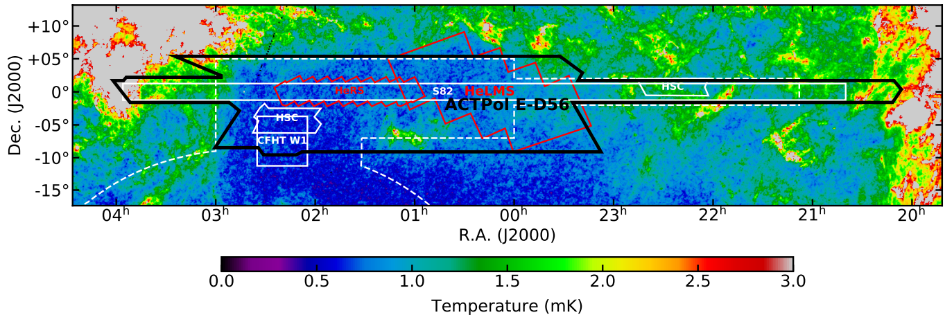
Figure 1. The location of the combined ACT equatorial and ACTPol D56 field (E-D56; covering area 987.5 \text{ deg}^2 after masking) overlaid on the Planck 353 GHz map, which is sensitive to thermal emission by dust. The locations of Herschel surveys (HeLMS [part of HerMES; Oliver et al. 2012], HeRS [Viero et al. 2014]) and deep optical surveys (CFHTLS W1, HSC [ongoing, current coverage marked; Aihara et al. 2017a], SDSS S82 [Annis et al. 2014]) are also shown. The expected final footprint of the Dark Energy Survey (DES; Diehl et al. 2016) is shown as the dashed white line. Almost the entire E-D56 field is covered by the SDSS legacy survey.
