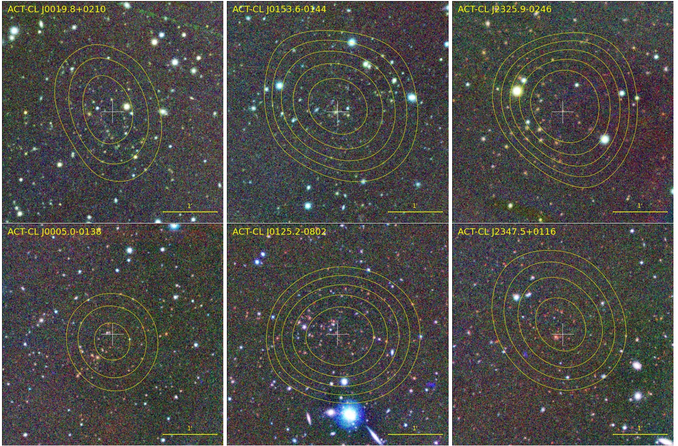
Figure 16. Images of newly discovered z > 0.7 clusters, confirmed with imaging from the ARC 3.5m and SOAR telescopes. Each image is 4' on a side, with North at the top and East at the left. The top row shows SOAR riz images, while the bottom row shows SOAR+ARC 3.5m riK s images, with the K s -band channel coming from the latter. The yellow contours (minimum 3\sigma , increasing in steps of 0.5\sigma ) indicate the (smoothed) 148 GHz decrement in the matched-filtered ACT map. The white cross indicates the ACT SZ cluster position.
