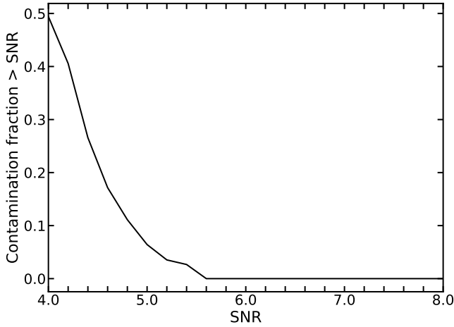
Figure 5. Estimated contamination fraction, i.e., false positive detection rate, versus SNR optimized over all filter scales. This is estimated by running the cluster finder over inverted maps, as described in Section 2.2.
