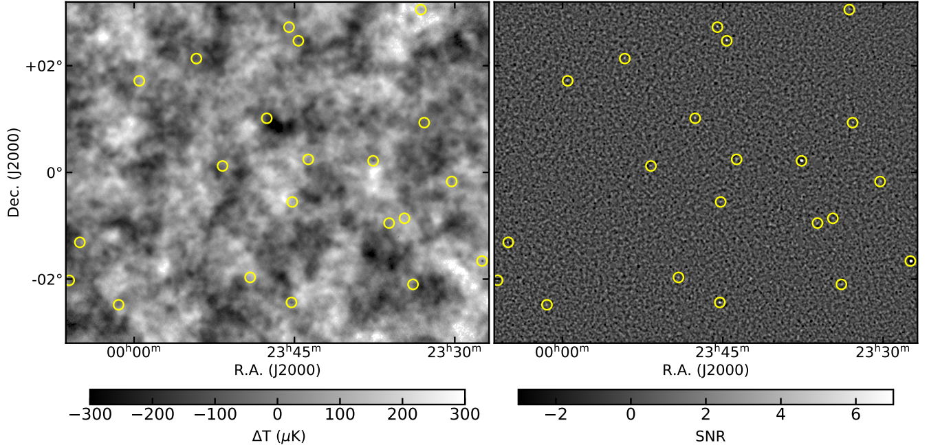
Figure 4. Zoom-in on a 79 \text{ deg}^2 section of the E-D56 map, to show the comparison between the unfiltered (left) and filtered (right) maps. The filtered map is the result of convolution with the real-space matched filter kernel (described in Section 2.2) with \theta_{500c} = 2.4' , corresponding to an UPP-model cluster with M_{500c} = 2 \times 10^{14} M_{\odot} at z = 0.4 . The positions of detected clusters are highlighted with yellow circles. The highest SNR cluster detected, ACT-CL J2327.4-0204 ( z = 0.70 ; \text{SNR} = 23.7 ), is clearly visible near the lower right edge of both maps (in the unfiltered map, it appears as a decrement).
