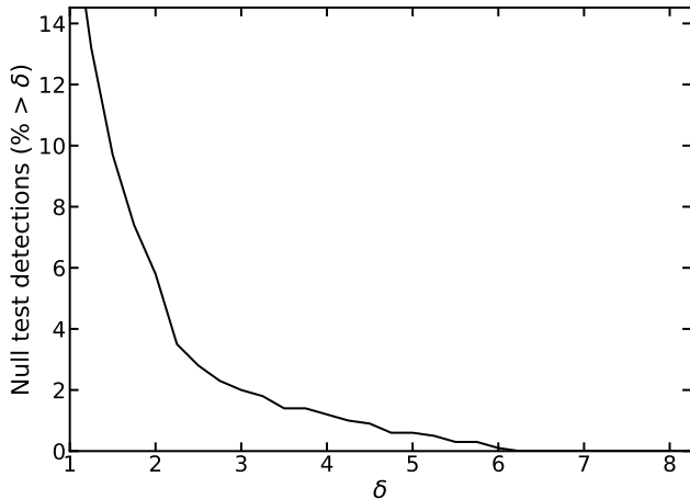
Figure 14. The cumulative fraction of false detections (expressed as a percentage) at random positions in the SDSS zCluster null test (see Section 3.3). For \delta > 3 , this shows that the false detection rate is 2%; this falls to 0.6% per cent for \delta > 5 .
