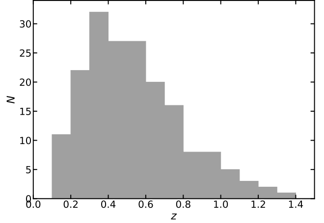
Figure 18. The redshift distribution of the 182 clusters in E-D56 cluster catalog. The median redshift is 0.49. The lack of clusters at low redshift ( z < 0.2 ) is largely a selection effect, due to the angular size of such clusters being similar to CMB anisotropies (see Section 2.4).
