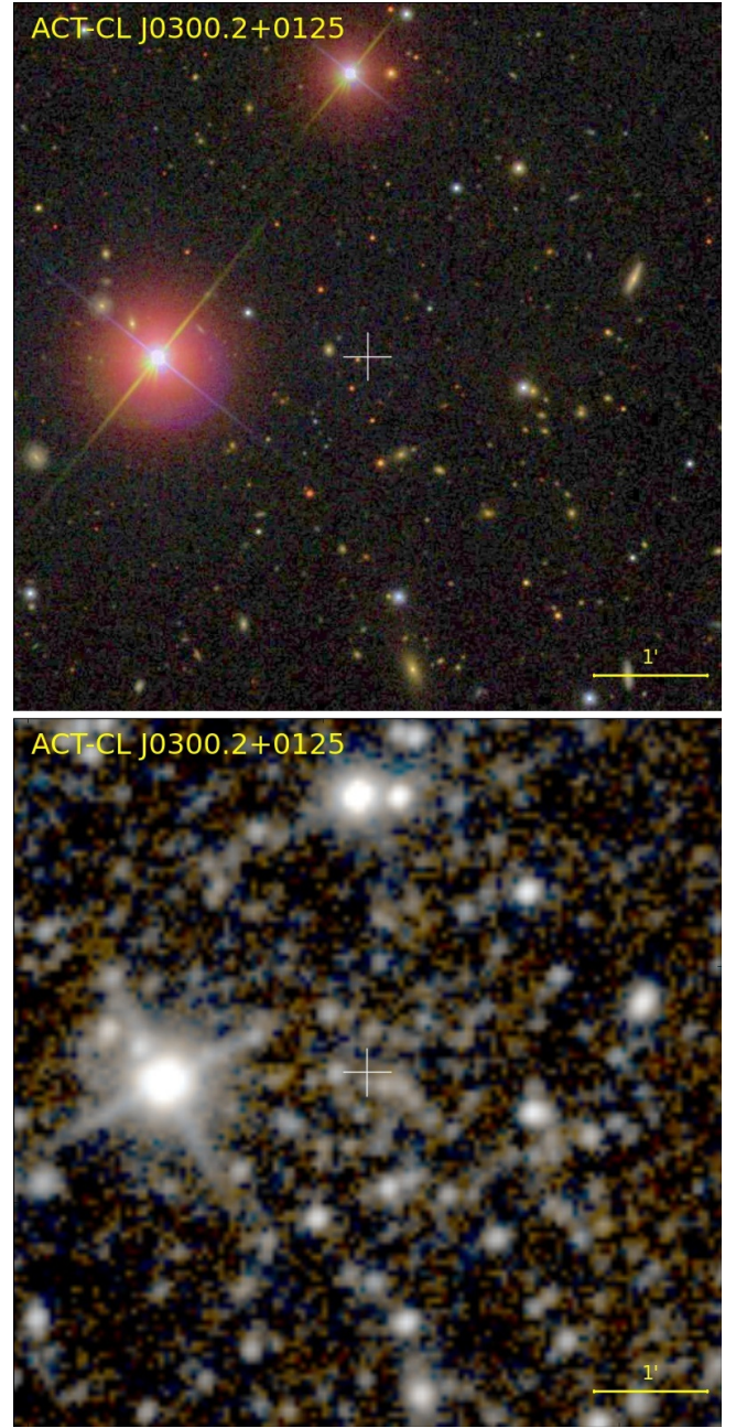
Figure 20. SDSS ( gri ; top) and WISE (W1/W2; bottom) imaging of ACT-CL J0300.2+0125, the candidate detected with the highest SNR (6.6) that does not yet have a redshift measurement. Each image is 6' on a side, with North at the top and East at the left. IR-bright but optically faint galaxies, with IR-colors consistent with those expected for early-type galaxies at z > 1 , are clearly visible close to the position of the SZ detection, which is marked with the white cross. The false color WISE image is taken from the unWISE project (Lang 2014).
