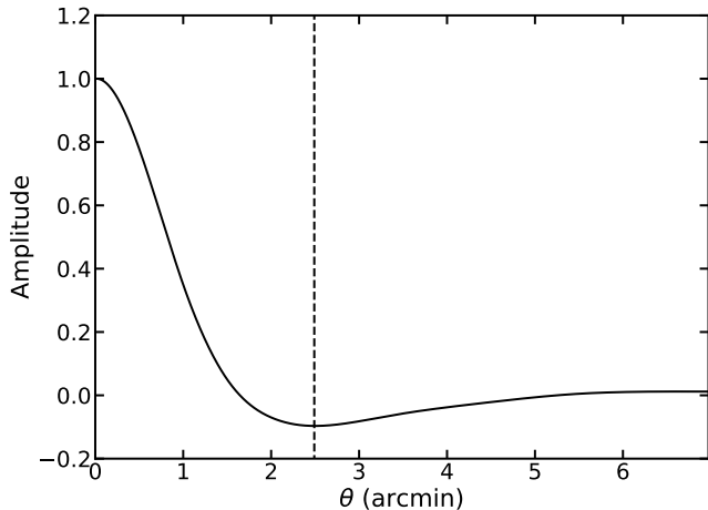
Figure 3. The matched filter profile, for the \theta_{500c} = 2.4' ( M_{500c} = 2 \times 10^{14} M_{\odot} at z = 0.4 ) filter scale. This is the reference scale used to characterize cluster masses and the survey completeness (see Sections 2.3 and 2.4). The vertical dashed line marks the scale on which the map is additionally high-pass filtered. For comparison, the beam FWHM is 1.4' , and the ACT maps have 0.5' pixel scale.
