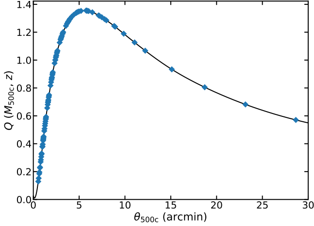
Figure 7. The filter mismatch function, Q , which is used to reconstruct cluster central Compton parameters and in turn infer cluster masses (see Section 2.3), under the assumption that clusters are described by the UPP and A10 scaling relation. In this work, we use a matched filter constructed from a UPP model with M_{500c} = 2 \times 10^{14} M_{\odot} at z = 0.4 ( \theta_{500c} = 2.4' ) as our reference. The blue diamonds mark scales at which the value of Q was evaluated numerically, over wide ranges in mass ( 13.5 < \log M_{500c} < 16 ) and redshift ( 0.1 < z < 1.7 ), while the solid line is a spline fit.
