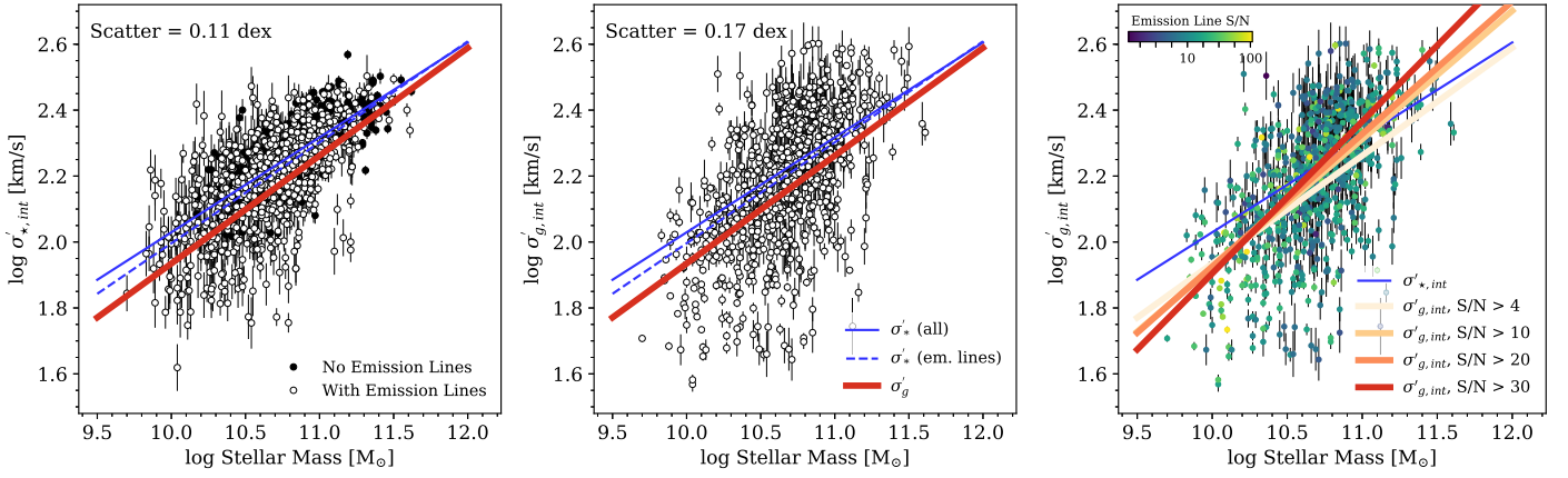
Figure 5. Mass FJ relation measured from absorption ( \sigma'_{*,int} , left panel) and emission ( \sigma'_{g,int} , center and right panels). Open/colored and black symbols indicate galaxies with and without emission lines. Best-fit linear relations with \sigma'_{*,int} (solid line for all galaxies and dashed for only those with emission lines) and \sigma'_{g,int} (thick red line) for subsamples above a range of S/N thresholds (red and orange lines). The Mass FJ relations are very similar for the full population, indicating that either measure can be used to estimate galaxy dynamics; however, the \sigma'_{*,int} relation is much tighter and somewhat shallower, with a vertical scatter of 0.11 dex relative to 0.17 dex measured from \sigma'_{g,int} . This increased scatter translates to an additional uncertainty of \sim 0.2 dex in dynamical mass. Furthermore, relying on bright emission features will bias toward an increasingly steep relation.
