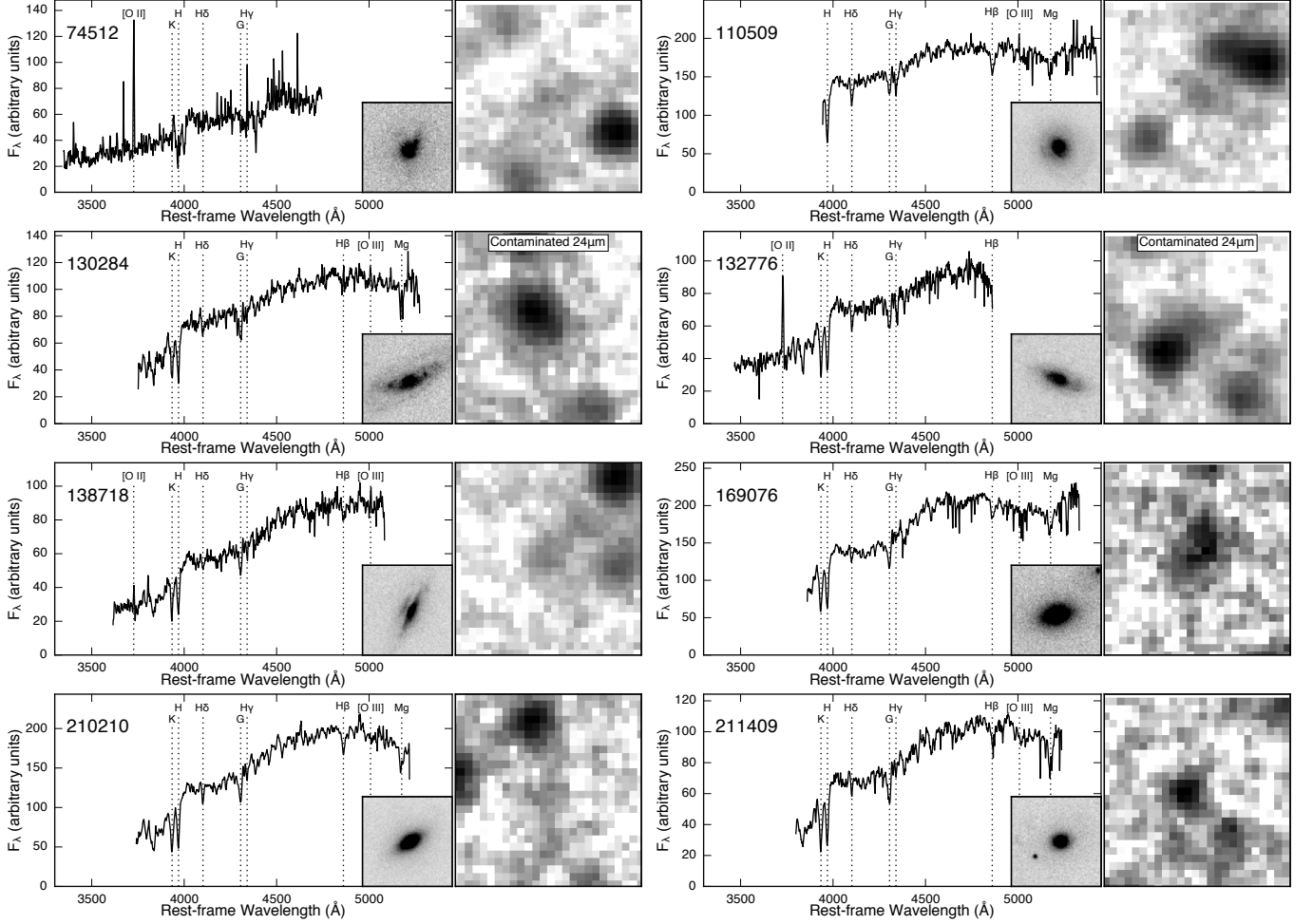
Figure 1. Left: Rest-frame optical LEGA-C spectra for each observed target, with common emission and absorption lines indicated. Spectra have been smoothed with a Gaussian of FWHM 4 \text{ \AA} . Insets: HST /ACS F814W images of each galaxy. Cutouts are 4 \times 4'' . Right: Spitzer /MIPS 24 \mu\text{m} images of each target, logarithmically scaled. Cutouts are 30 \times 30'' . Most galaxies are clearly or marginally detected at 24 \mu\text{m} , although two objects have photometry that is likely contaminated by nearby galaxies.
