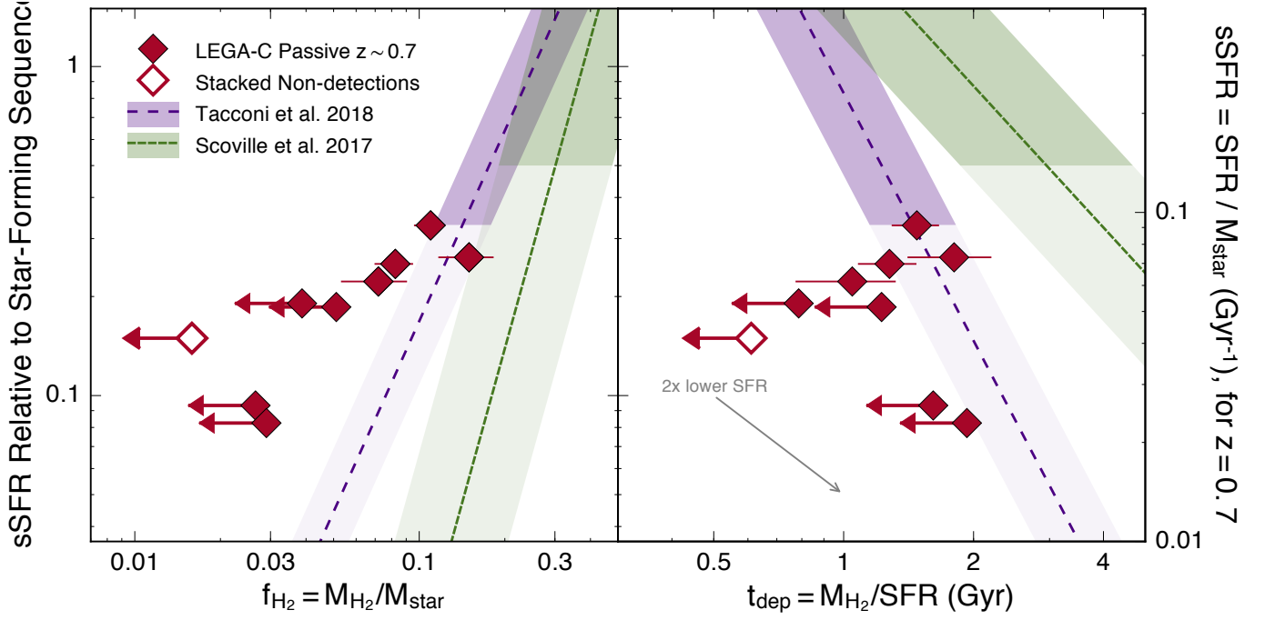
Figure 7. The molecular gas fraction f_{\text{H}_2} (left) and depletion time t_{\text{dep}} (right) versus the specific SFR, compared with observationally-derived literature scaling relations from Scoville et al. (2017) (green densely dashed line and region) and Tacconi et al. (2018) (navy dashed line and region), evaluated for \log M_{\text{star}}/M_{\odot} = 11 . Both literature scaling relations are parameterized in terms of the offset of the sSFR with respect to the expectation from the star-forming sequence, and so the left-hand y-axis is also labeled in these terms. The right-hand y-axis is labeled with the corresponding values of the sSFR, evaluated at z = 0.7 . The shaded regions encompass the quoted approximate 1\sigma residual scatter around the relations. The darker shaded bands correspond to the approximate sSFR lower bounds for galaxies at z = 0.6 - 0.8 that were used in the derivation of the scaling relations; below these regions the scaling relations are extrapolations (lightly shaded). In the right-hand panel, a grey arrow indicates the shift if the SFRs for our galaxies have been overestimated by a factor of 2; the shift is largely parallel to the scaling relations. In general, the CO-detected objects in our sample are in reasonable agreement with the scaling relations, while the undetected objects, and especially the stacked non-detections, are significantly offset from the extrapolated relations. This could indicate either a strong break in the scaling relations at 3-5\times lower sSFR than the star-forming sequence, or a large increase in the scatter of f_{\text{H}_2} and t_{\text{dep}} .
