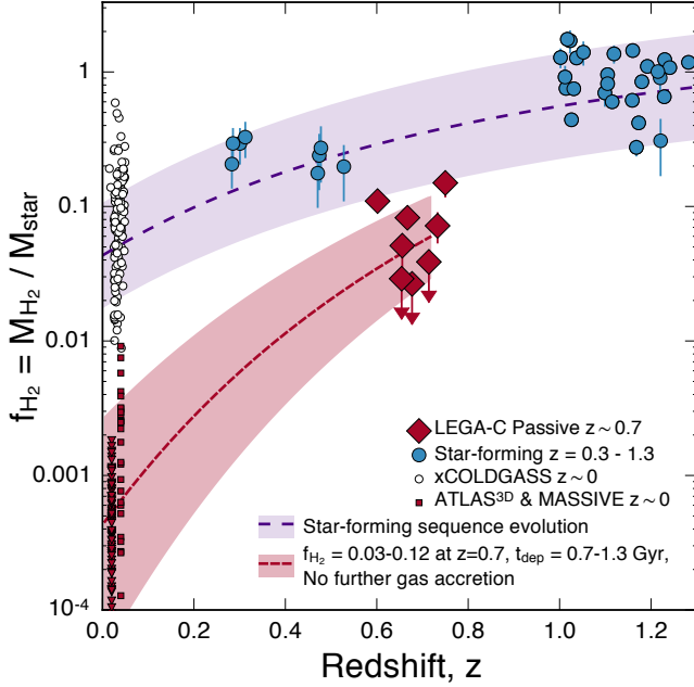
Figure 9. Evolution of f_{\text{H}_2} with redshift for galaxies on and below the star-forming sequence. Our observations are shown with red diamonds, blue circles show galaxies near the star-forming sequence at 0.3 < z < 1.3 (Bauermeister et al. 2013; Tacconi et al. 2013), white circles are z < 0.05 star-forming galaxies with 10 < \log M_{\text{star}}/M_{\odot} < 10.7 from xCOLDGASS (Saintonge et al. 2017), and small red symbols show massive ( \log M_{\text{star}}/M_{\odot} > 10.7 ) quiescent galaxies from the ATLAS 3D and MASSIVE surveys (Young et al. 2011; Davis et al. 2016). For clarity of presentation, all detections and non-detections from these last two surveys are plotted at z = 0.04 and z = 0.02 , respectively; in reality all these galaxies are within 110 Mpc ( z < 0.025 ). The densely-dashed red line and region sketch a plausible evolutionary path for the passive galaxies we observed from z = 0.7 to z = 0 , assuming initial starting f_{\text{H}_2} = 0.03 - 0.12 and constant t_{\text{dep}} = 0.7 - 1.3 Gyr, and no subsequent accretion of gas. The navy dashed line and region show the evolution for galaxies with 10 < \log M_{\text{star}}/M_{\odot} < 11 and within a factor of 3 of the star-forming sequence from Tacconi et al. (2018), where the wide range of these parameters is intended to smooth over the trajectory of individual galaxies around the star-forming sequence. The continuity of this relation and the star-forming sequence requires substantial gas accretion over cosmic time. This Figure demonstrates that the galaxies we have observed at z \sim 0.7 can naturally reproduce the observed gas fractions of the local massive, quiescent population simply by maintaining the same (relatively short) t_{\text{dep}} we measure, with no need for further gas accretion or dynamical stabilization.
