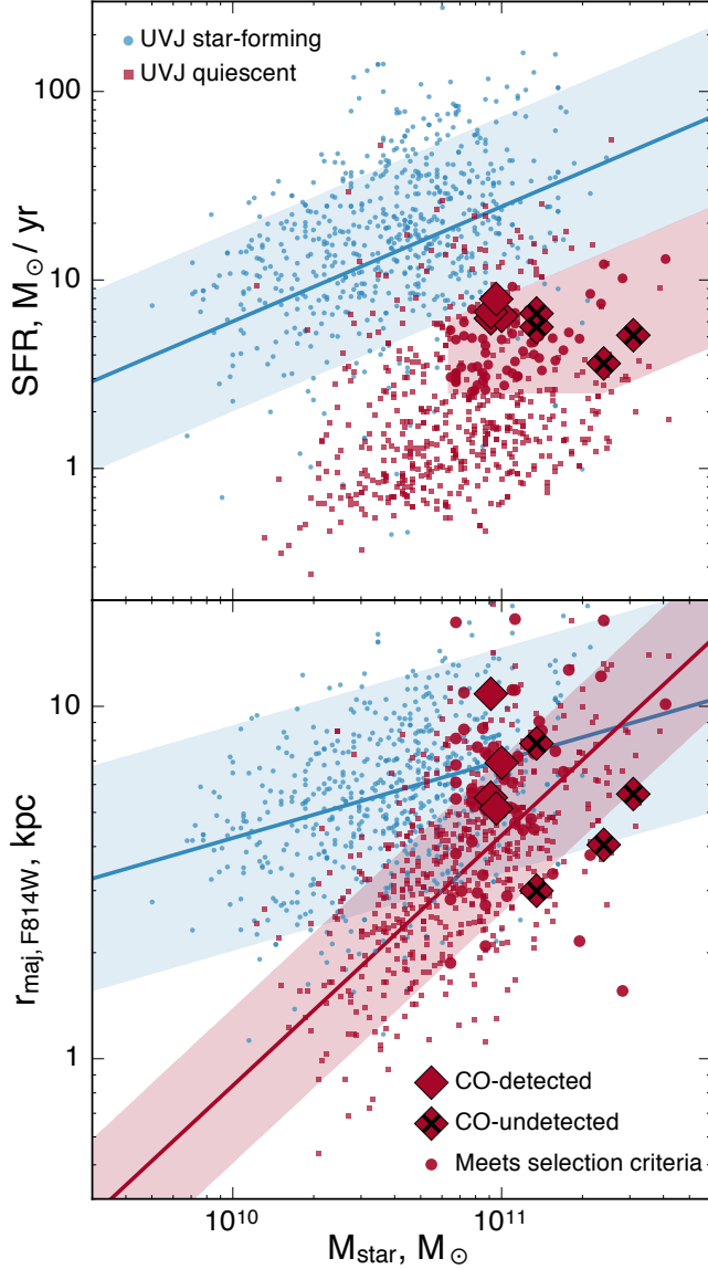
Figure 2. The selection of the ALMA-observed massive, passive sample with respect to the full LEGA-C sample. In both panels, the LEGA-C sample galaxies are color-coded blue (red) if they are classified as star-forming (quiescent) in rest-frame UVJ space (see Figure 3). Red circles are all LEGA-C galaxies that meet our selection criteria, while the ALMA-observed objects are shown with large red diamonds; CO-undetected objects are also marked with a black ‘x’. Top: The ALMA sample was primarily selected based on stellar mass and SFR; see text for details. The blue line shows the star-forming sequence at z = 0.7 from Whitaker et al. (2012), and the blue shaded region encompasses SFRs a factor of 3 above and below the relation. The red shaded region shows our selection box of massive and passive galaxies. Bottom: Size-mass relation for the LEGA-C and ALMA samples. Blue and red lines and regions show the size-mass relations for star-forming and quiescent galaxies at z = 0.75 from van der Wel et al. (2014).
