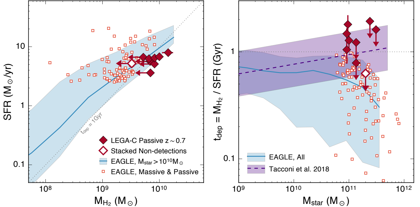
Figure 8. Left: The star formation relation from a z = 0.6 snapshot of the EAGLE simulation, compared with our results. The individual objects and stacked non-detection from our observations are shown with red diamonds. The blue line and shaded region show the median and 90% range of all galaxies in EAGLE with \log M_{\text{star}}/M_{\odot} > 10 . The small orange squares show galaxies in EAGLE that mimic our selection criteria; see text for details. The dotted grey line shows a constant depletion time t_{\text{dep}} = 1 \text{ Gyr} . Right: The gas depletion times as a function of stellar mass from the same EAGLE snapshot. The blue line and shaded region again shows the median and 90% range of depletion times for all EAGLE galaxies, with those that mimic our selection criteria as orange squares. The dashed navy line and region, on the other hand, show the predicted scaling relation from Tacconi et al. (2018) for galaxies on and a factor of 3 above (lower edge of region) and below (upper edge) the star-forming sequence at these redshifts. Note also that this Figure does not contradict our results in Figure 7, even though the t_{\text{dep}} upper limits from the CO non-detections overlap with the shaded region, because these galaxies have significantly lower sSFR than merely 3\times below the star-forming sequence.
