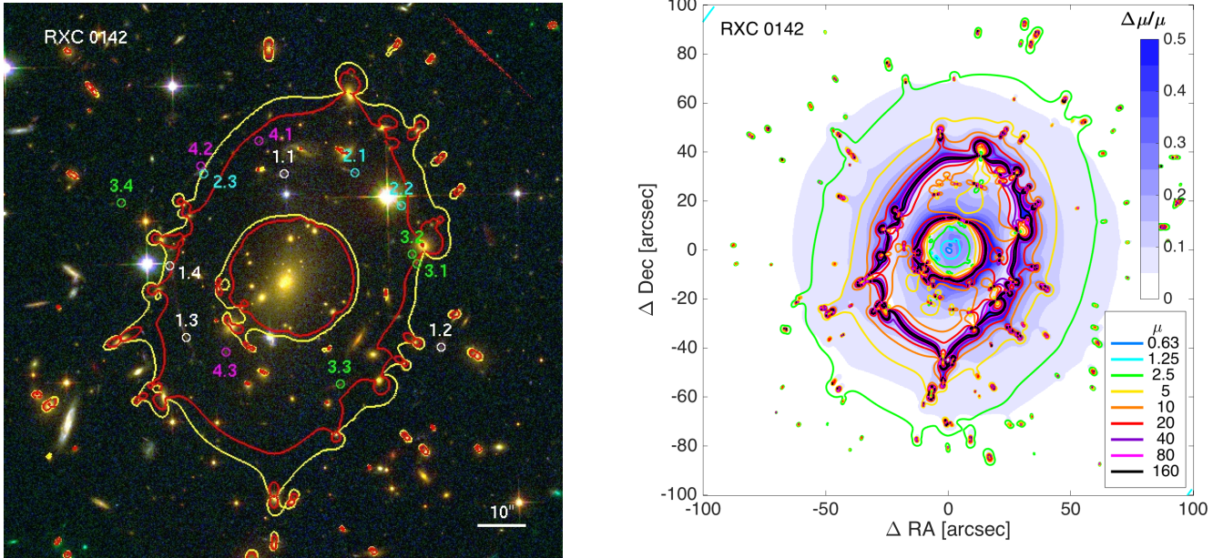
FIG. 2.— Left : Image of RXC J0142+44 created using a combination of WFC3/IR imaging in the red (F160W) and ACS imaging in the green (F814W) and blue (F435W) filters. The locations of multiply imaged lensed galaxies are overplotted and labeled. The red curve marks the location of the critical curve for a source at z = 3.0 . The yellow curve marks the location of the critical curve at z = 9.0 . Right : The magnification for a source at z = 9.0 from the best-fit lens model is shown as contours; contour values are given in the legend. The background colormap indicates the uncertainty level in each location, given as \Delta\mu/\mu . The uncertainty estimate takes into account the source redshift uncertainty, but does not account for other systematics (see text).
