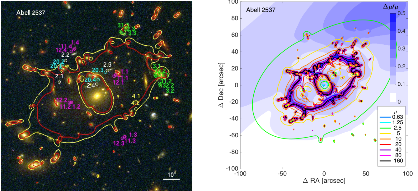
FIG. 1.— Left : Image of Abell 2537 created using a combination of WFC3IR imaging in the red (F160W) and ACS imaging in the green (F814W) and blue (F435W). Multiply imaged galaxies are labeled. The red curve marks the location of the critical curve for a source at z = 3.0 . A second critical curve is plotted in yellow at z = 9.0 . Right : The magnification for a source at z = 9.0 from the best-fit lens model is shown as contours; contour values are given in the legend. The background colormap indicates the uncertainty level in each location, given as \Delta\mu/\mu . The uncertainty estimate takes into account the source redshift uncertainty, but does not account for other systematics (see text).
