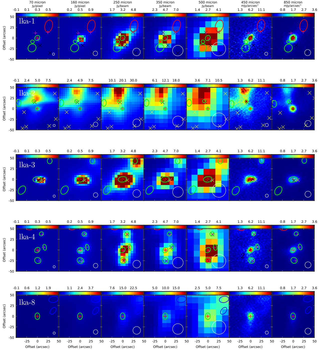
Fig. 9.— Quality-assurance maps for compact sources extracted using getsources showing (left to right) the Herschel /PACS (70 and 160 \mu\text{m} ), Herschel /SPIRE (250, 350, and 500 \mu\text{m} ), and SCUBA-2 (450 and 850 \mu\text{m} ) maps. Each panel is centered on the compact source in question, which is marked with crosshairs. Elliptical regions are the same as in Figures 2 with blue, red, and green ellipses marking identified candidate YSOs at 450 \mu\text{m} , 850 \mu\text{m} , or both, respectively, and with major and minor FWHM and orientation according to the source properties measured with getsources . The internal getsources ID is listed in the upper left corner of the 70 \mu\text{m} map for each source. (We use the internal getsources ID to identify the compact sources, as we make the plots for the complete set of 79 compact sources and not just the subset of 59 candidate YSOs.) This figure is the extended version of Figure 4.
