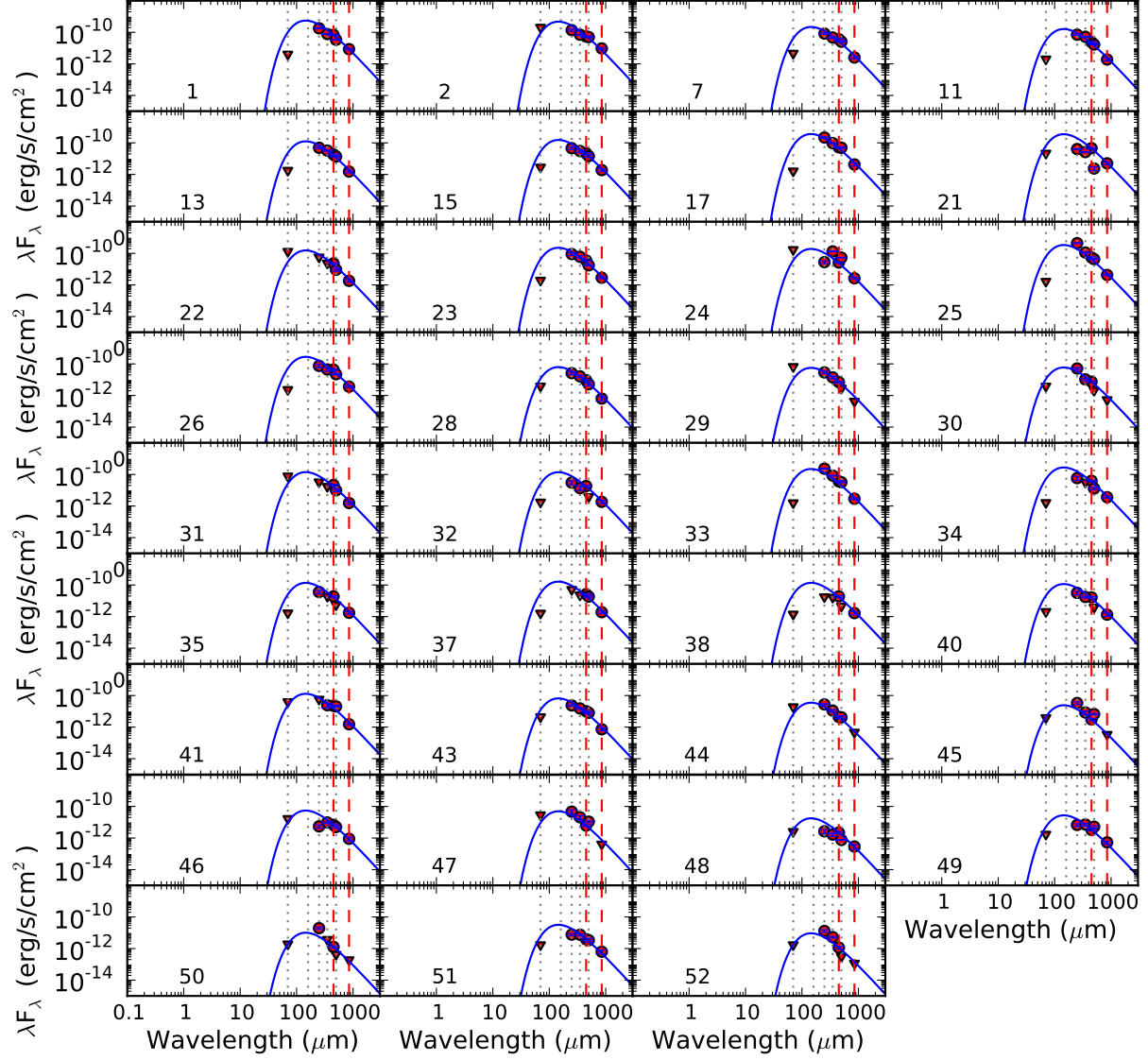
Fig. 7.— SEDs for SCUBA-2 candidate YSOs not associated with Spitzer -identified or Herschel /PACS-identified YSOs (probably due to observational constraints in the region rather than the absence of compact IR flux; see Section 3.3.1). The ID from Table 1 is shown in the bottom of each panel. The blue curve shows the emission from 20 K dust scaled to 450 and 850 \mu\text{m} fluxes where available (see Section 3.6) and listed in Table 3. The red dashed lines mark the SCUBA-2 wavelengths at 450 and 850 \mu\text{m} , and the black dotted lines mark the Herschel /SPIRE wavelengths at 250, 350, and 500 \mu\text{m} .
