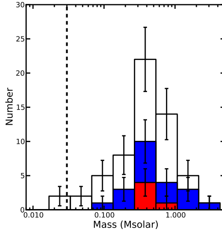
Fig. 8.— Circumstellar (disk + envelope) mass distribution of calculated masses. The distribution for all YSOs, both candidate and robust, is shown in white. The distribution shown in blue includes only robust YSOs with a Spitzer counterpart, and the Class II YSOs are shown in red. The JCMT GBS observations are sensitive to the high-mass end of the mass distribution. The dashed vertical line marks our 3\sigma limit at 850\ \mu\text{m} absent of bright cloud emission at 0.03\ M_{\odot} assuming T = 20\ \text{K} and \beta = 1 . (Mass measurements leftward of this line are due to 450\ \mu\text{m} fluxes.)
