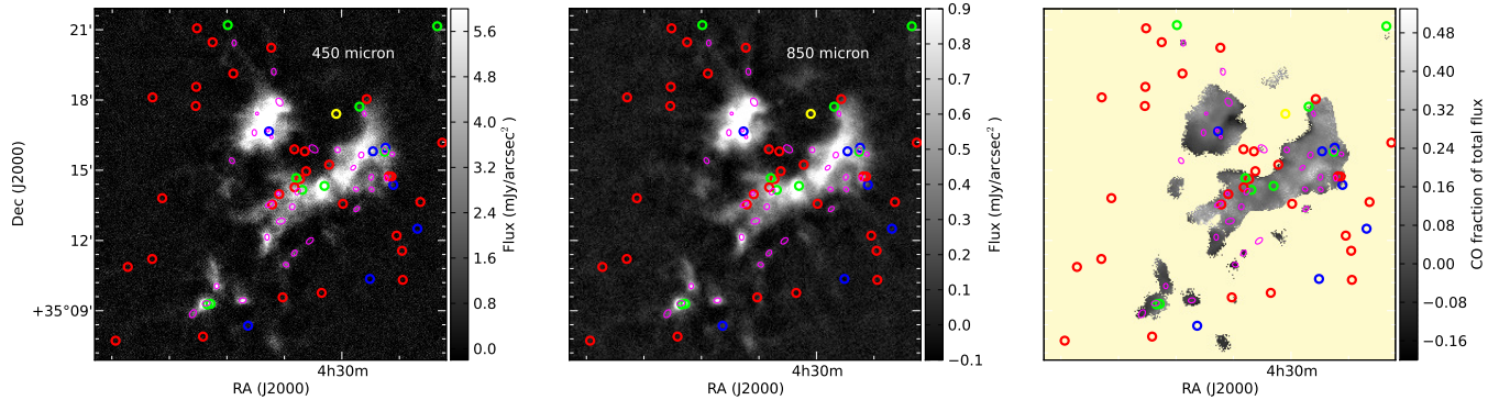
Fig. 5.— The SCUBA-2 450 \mu\text{m} (left) and 850 \mu\text{m} (center) maps of the young cluster around LkH \alpha 101. This is the region where the majority of candidate YSOs (i.e., those without an IR counterpart) are located. The bright cloud emission in the vicinity makes it difficult to identify YSOs at infrared wavelengths with both Spitzer and Herschel /PACS. The locations of SCUBA-2-identified candidate YSOs (magenta ellipses) are shown, with size corresponding to source FWHM. Spitzer -identified YSOs (circles) are shown from the Broekhoven-Fiene et al. (2014) catalog, with green, blue, red, and yellow corresponding to Class I, Class F, Class II, and Class III YSOs, respectively. Very few coincide with the location of our candidate YSOs (see discussion in text). The fractional contribution of CO to the total 850 \mu\text{m} flux (right) is calculated from the CO-subtracted and non-CO-subtracted 850 \mu\text{m} maps in the region around LkH \alpha 101. We mask pixels where the 850 \mu\text{m} flux is not detected, i.e., < 3\sigma (pale yellow background) to measure the fractional contamination of CO in this region from only detected emission. Their locations coincide with lower relative CO contamination (generally levels below \sim 20\% ), since the 850 \mu\text{m} continuum flux is higher.
