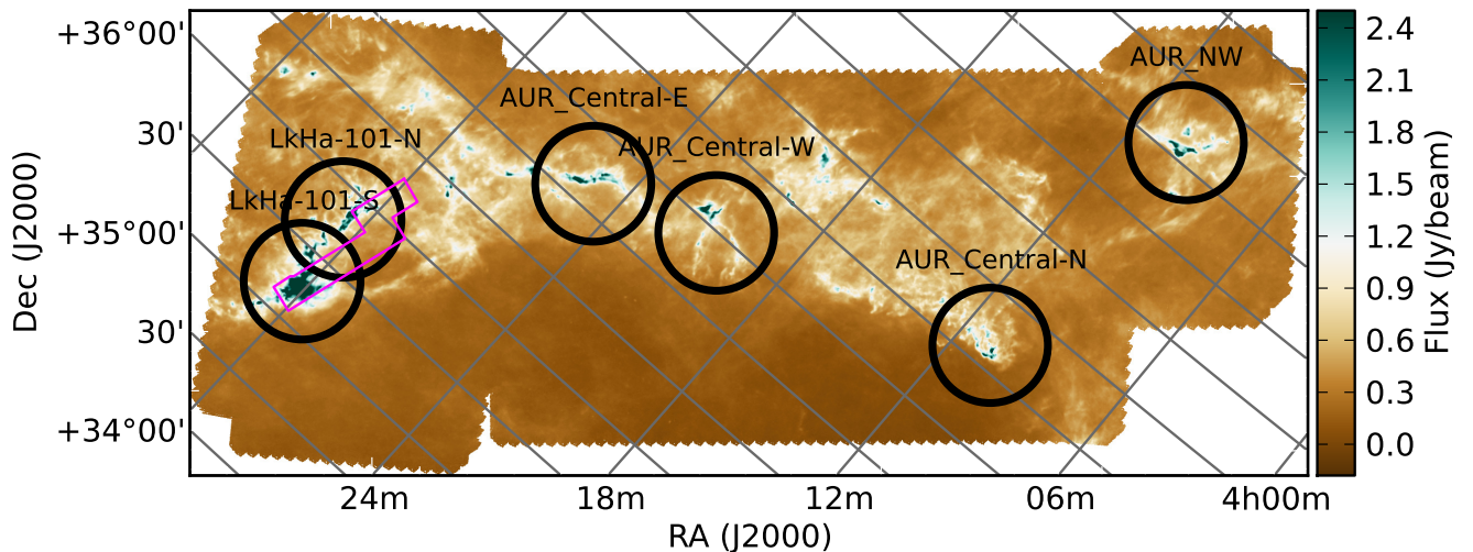
Fig. 1.— SCUBA-2 observed regions in Auriga-Cal. Circles marking the area observed by SCUBA-2 (and labeled according to their observation name) are overlaid on the Herschel 500\ \mu\text{m} map from Harvey et al. 2013 to illustrate the locations throughout the cloud that were mapped. The regions with the highest column density and most compact sizes were targeted, and the LkH \alpha 101 pongs, which cover the part of the cloud with the densest area of star formation, were prioritized to be observed in the best weather (Band 1). The ^{12}\text{CO}\ J = 3 - 2 coverage is outlined in magenta. For optimal display of the entire cloud, the celestial coordinates are tilted; i.e., north is not up as it is in Figure 2.
