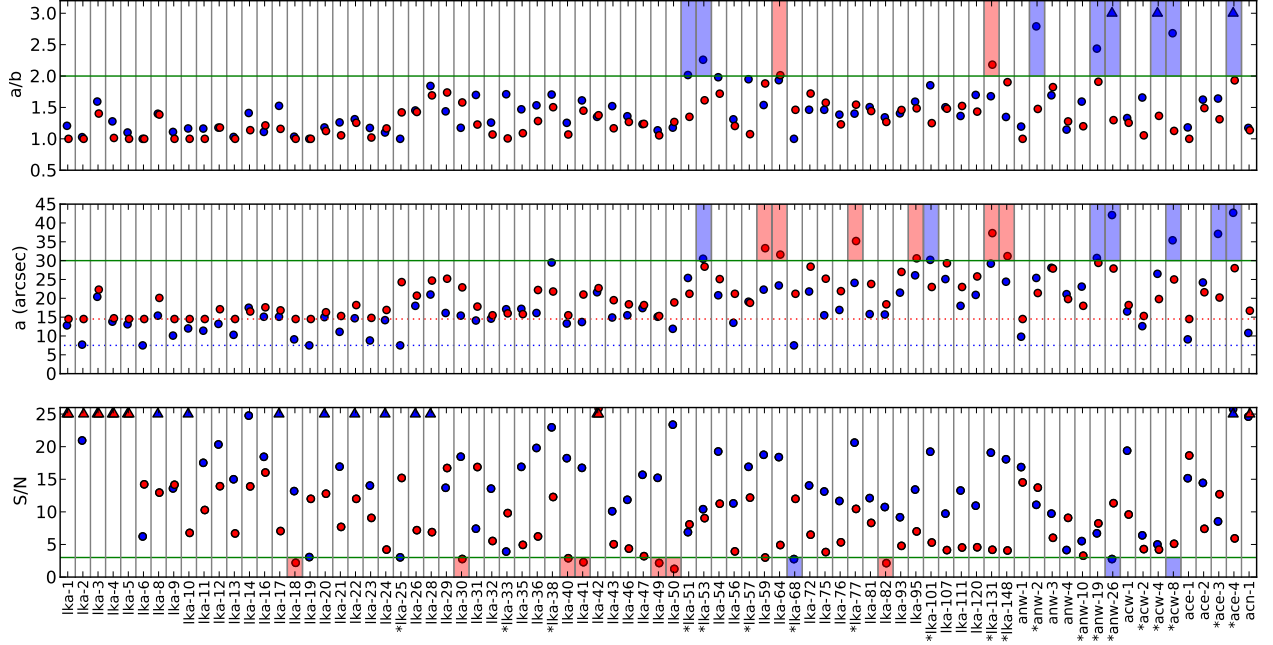
Fig. 3.— Criteria for identifying compact objects from the getsources extraction: aspect ratio (top), size (middle), and S/N (bottom) for each of the 79 objects that meet our criteria for compact sources at one or both SCUBA-2 wavelengths. The green horizontal lines mark the boundaries for each criterion during the initial selection of compact sources. The measured property is displayed for each source at both 450\ \mu\text{m} (blue) and 850\ \mu\text{m} (red). (Note that an upward arrow is displayed for values that extend beyond the plot boundaries.) The area of the plot is shaded where a compact source does not meet the criterion at the wavelength corresponding to the color of the shading (blue= 450\ \mu\text{m} , red= 850\ \mu\text{m} ). Blue and red dotted lines show the 450\ \mu\text{m} and 850\ \mu\text{m} beam sizes, respectively. Additional flags arise during the vetting process if a source is much larger at 450\ \mu\text{m} than at 850\ \mu\text{m} (since the 850\ \mu\text{m} beam is larger and we expect a real protostellar source to have roughly the same physical size at both wavelengths) or when the elongation measured at the two wavelengths is very different. Each compact source is labeled according to the internal getsources ID from the source extraction. Those preceded by a “*” are excluded from the final list of YSO candidates based on the flagging described.
