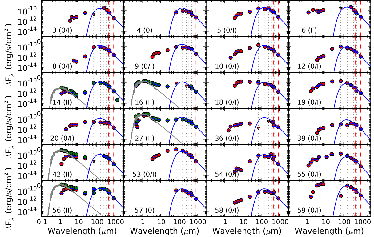
Fig. 6.— SEDs for SCUBA-2 robust YSOs, i.e., those associated with a detected Spitzer YSO and/or Herschel /PACS YSO. The ID number from Table 1 is shown in the bottom of each panel with the YSO class based on the Spitzer infrared spectral slope (from Broekhoven-Fiene et al. 2014) listed in parentheses. Note, however, that since Spitzer cannot distinguish between Class 0 and Class I, we have labeled the Spitzer Class I YSOs as Class 0/I YSOs to represent this ambiguity. Note that YSOs 4 and 57 are only identified with Herschel /PACS in the infrared, so we use the YSO identification from Harvey et al. (2013) (Class 0) for these YSOs. Red circles show observed fluxes. Panels with Class II sources include a sample stellar K7 spectrum that is normalized to the infrared flux at the shortest available wavelength. The fitted stellar spectrum is used to estimate an A_V value and therefore the dereddened fluxes (green circles). The blue curve shows the emission from 20 K dust scaled to 450 and 850 \mu\text{m} fluxes where available (see Section 3.6) and listed in Table 3. The red dashed lines mark the SCUBA-2 wavelengths at 450 and 850 \mu\text{m} , and the black dotted lines mark the Herschel /SPIRE wavelengths at 250, 350, and 500 \mu\text{m} .
