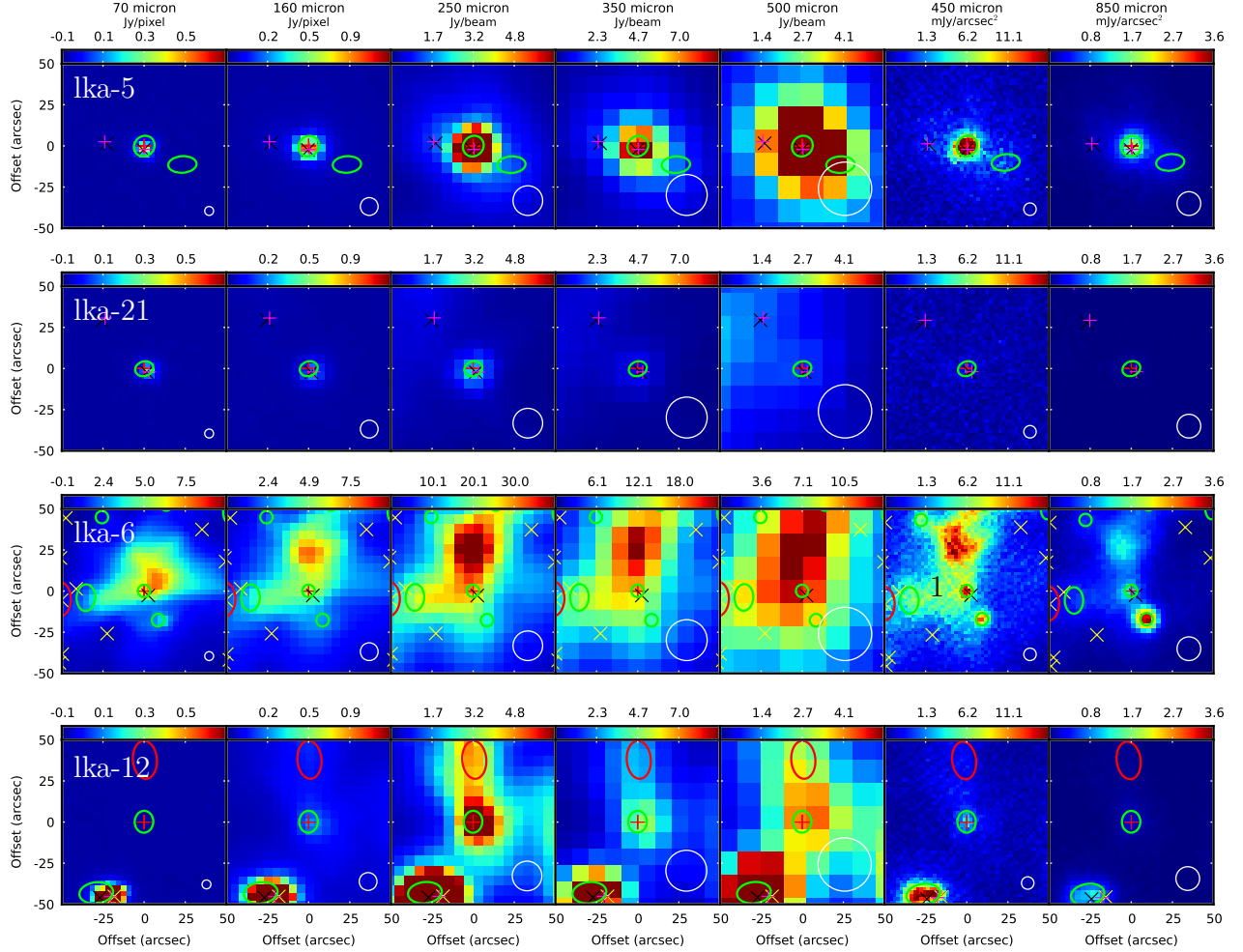
Fig. 4.— Examples of the quality-assurance maps for compact sources extracted using getsources showing (left to right) the Herschel /PACS (70 and 160 \mu\text{m} ), Herschel /SPIRE (250, 350, and 500 \mu\text{m} ), and SCUBA-2 (450 and 850 \mu\text{m} ) maps. Each panel is centered on the compact source in question which is marked with crosshairs. Elliptical regions are the same as in Figures 2 with blue, red, and green colors marking sources that satisfy the compact source criteria at 450 \mu\text{m} , 850 \mu\text{m} , or both, respectively, and with major and minor FWHM and orientation according to the source properties measured with getsources . The internal getsources ID is listed in the upper left corner of the 70 \mu\text{m} map for each source. From top to bottom, the rows show the following. (1) An example of a well-detected compact source (lka-5) associated with a YSO identified with both Spitzer and Herschel /PACS. (2) A compact source (lka-21) identified in SCUBA-2 maps that is not very convincing visually at either 450 or 850 \mu\text{m} , but for which inspection of Herschel maps provided the by-eye conviction of the presence of compact emission. This demonstrates the effectiveness of getsources ’s source identification in the SCUBA-2 maps. (3) An example of a compact source (lka-6) for which the presence of compact 70 \mu\text{m} emission, indicative of a protostellar source, can be neither confirmed nor ruled out given the presence of bright background emission. (4) An example of a seemingly robust submillimeter compact source (lka-12) that is not detected at wavelengths shorter than 160 \mu\text{m} . Each of these four compact sources passes the vetting process to be identified as candidate YSOs. Such figures for the remaining compact sources are included in the Appendix and shown in Figure 9.
