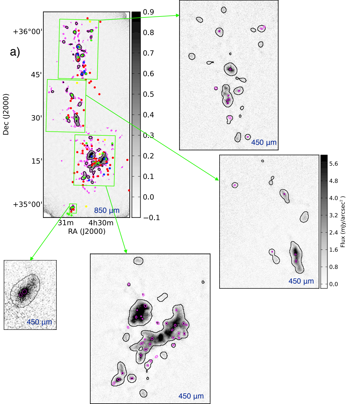
Fig. 2.— (a) Maps of the LkH \alpha 101 regions at 850 \mu\text{m} (top left) and 450 \mu\text{m} (other panels). The continuation of this figure on following pages shows the maps of the AUR_Central-E (b), AUR_Central-W (c), AUR_Central-N (d), and AUR_NW (e) regions at 850 \mu\text{m} (left) and 450 \mu\text{m} (right). Black contours in all panels trace the external mask used in the data reduction (Section 2.1). In the 850 \mu\text{m} panel, magenta contours highlight detected emission tracing an S/N of 1 smoothed over 5 pixels (computed from the data and variance maps). Overlaid are green, blue, red, and yellow points that show the locations of Class I, flat-spectrum, Class II, and Class III YSOs, respectively, from Broekhoven-Fiene et al. (2014). (See discussion in Section 3.2.) The green boxes in the 850 \mu\text{m} panel show the areas that are enlarged for the 450 \mu\text{m} panels. The 450 \mu\text{m} panels are all displayed with the same color-scale ranges. In these panels, magenta ellipses mark identified candidate YSOs in SCUBA-2 maps, with major and minor FWHM and orientation according to the source properties measured with getsources (see Section 3.1 and Figures 4 and 9 for panels of individual candidate YSOs). Some faint filamentary structure is visible in these maps and matches that seen in Herschel 500 \mu\text{m} maps (c.f. Figure 1). (Note that some of the noisy map edges are visible in the area displayed.)
