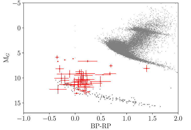
Fig. 2. An HR diagram made using Gaia DR2 data. In red we show the absolute G magnitude, M_G , as a function of the blue–red colour, BP–RP, for AM CVns with known parallaxes. No reddening or extinction corrections have been applied to this figure. For comparison, in grey points we show a sample of essentially randomly selected main sequence stars which have a parallax better than 1 percent. For single white dwarfs shown as slightly larger grey points) we have used the sample of white dwarfs within 20 pc (Hollands et al. 2018). The majority of AM CVns appear to be brighter than the single white dwarf track, though some long-period systems lie on the track. A clear outlier is V407 Vul, which has BP–RP \approx 1.5 through a combination of severe reddening and contamination from an unresolved nearby G-star.
