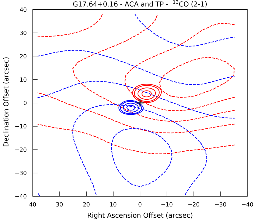
Fig. A.2. Contour plot of the ^{13}\text{CO} outflow emission from the ACA (solid) and TP (dashed) observations. The blue- and red-shifted velocities are 18.5 to 20.1\text{ km s}^{-1} and 28.5 to 30.5\text{ km s}^{-1} respectively. The ACA contours are at 40, 50, 70 and 90 % of the peak value, while the total power are at 10, 30, 50, 70 and 90 % of the peak value. The plot is illustrative of the blue and red shift offset emission that forms the outflow, but also shows that the TP does not map a large enough region to fully map the entire CO emission.
