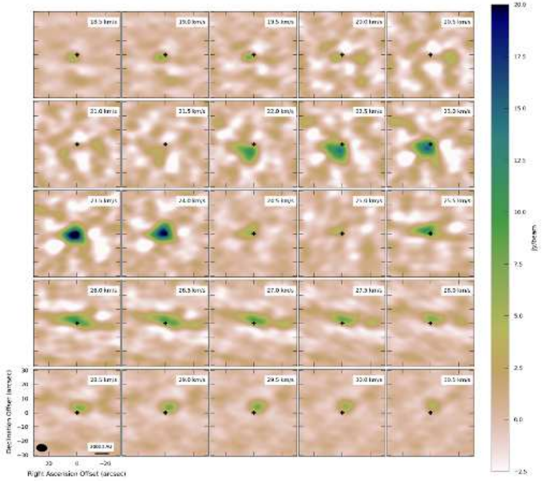
Fig. A.1. Channel map of the ACA ^{13}\text{CO} emission ranging from 18.5 to 30.5 \text{ km s}^{-1} in steps of 0.5 \text{ km s}^{-1} . Recall the source V_{\text{LSR}} is 22.1 \text{ km s}^{-1} . Note the highest velocities of the outflow in the blue- and red-shifted emission occur to the south-east and north-west respectively, perpendicular the putative disc. The blue-shifted emission is detected down to 16.9 \text{ km s}^{-1} but is co-spatial with that shown at 18.5 \text{ km s}^{-1} , while the red-shifted emission is detected to 35.6 \text{ km s}^{-1} but is the same structure as the panel at 30.5 \text{ km s}^{-1} .
