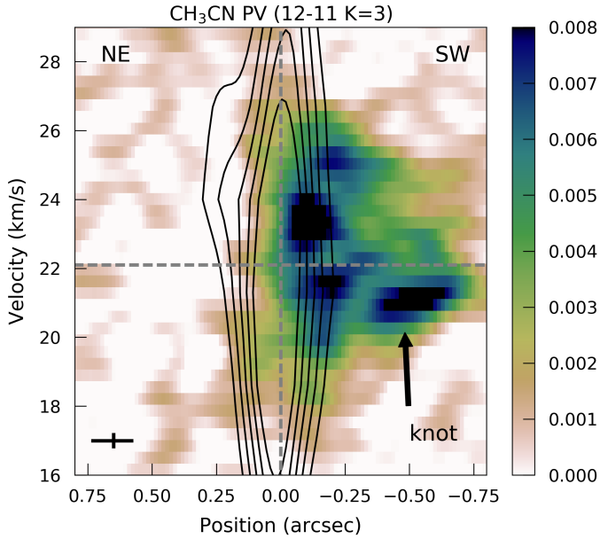
Fig. 7. Position-velocity (PV) diagram of the \text{CH}_3\text{CN} ( J=12-11 ) K=3 line (colour map) overlaid with the PV diagram of the \text{SiO} as in Fig. 4 (black contours). There is notable emission to negative spatial offsets related to a south-west direction along the PV cut, whereas to positives offsets (north-east) there is barely any emission. Both blue- and red-shifted emission coincide to the south-west, related to the signature of either a wide-angle wind, with flows nearly radially, or that there is simultaneous infall from material in front and behind the edge of the disc. The emission at bluer velocities and high negative offset ( -0.5'' ) is associated with the knot structure identified in Fig. 5. The spatial and velocity resolution of the \text{CH}_3\text{CN} map is shown at the bottom left, while the direction along the PV cut to the NE and SW is indicated at the top.
