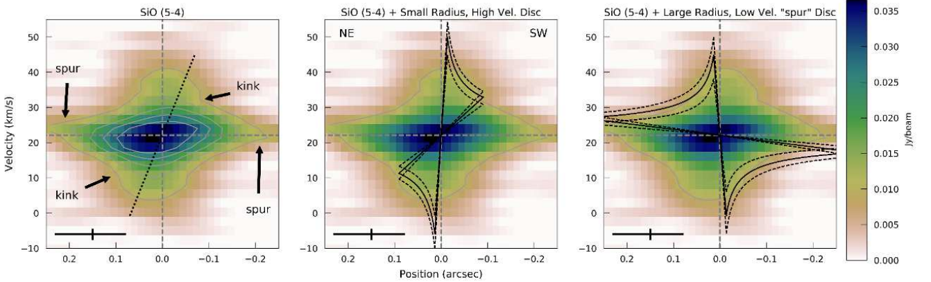
Fig. 4. Left: Position-velocity (PV) diagram of the SiO emission extracted from a cut (as wide as the synthesised beam) at a position angle of 30^\circ across the putative disc major axis (see Fig. 3 - position offsets are positive to north-east). The grey contours are at the 10, 15, 20, 25 and 30 \text{mJy beam}^{-1} level to highlight the structure. The black dotted line is a guide to indicate the excess of high velocity emission at small spatial offsets. Centre: Observed SiO PV as the left plot (colour map with grey contour at a 10 \text{ mJy beam}^{-1} level) overlaid with pure Keplerian rotation profiles for a 200 au radius disc around a 20, 30 and 40 M_\odot (inner dashed, solid, outer dashed lines) O-type YSO, when considering an inclination of 70^\circ (de Wit et al. 2011). The disc outer radius was limited to 200 au such that the lowest velocities roughly matched the kink in the observed data. The disc lines here represent only the high-velocity emission. Right: Observed SiO PV as the left and central plots but overlaid with the contours of pure Keplerian rotation profiles for a disc around a 10, 20, 30 M_\odot (inner dashed, solid, outer dashed lines) OB-type YSO rotating in the opposite direction to that plotted in the central panel (using an inclination of 70^\circ ). The disc outer radius was set to 650 au in an attempt to match the low velocity spurs at large spatial offsets. The spatial and velocity resolution are indicated by the black bars at the bottom left of all plots. Note the central figure indicates the north-east and south-west offset directions that relate to the cut along the disc direction in Fig. 3.
