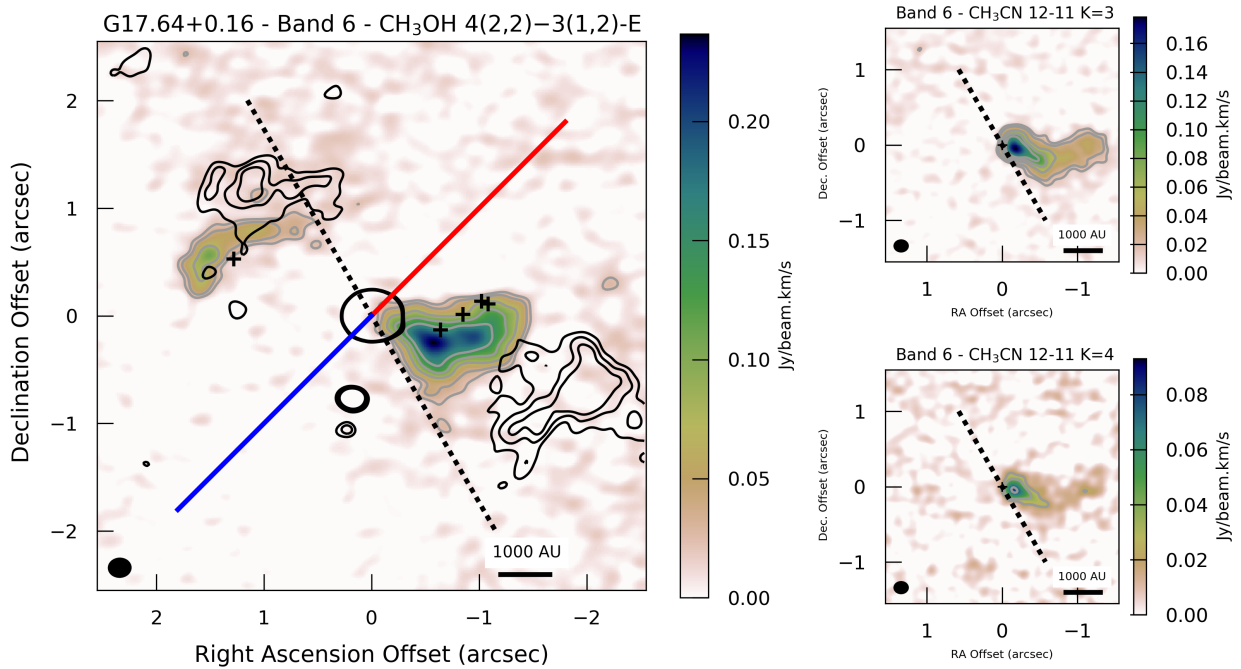
Fig. 6. Left: Moment zero map of the CH 3 OH line at 218.440 GHz integrated between 19.0 and 23.9 km s -1 (colour map). The contours of the CH 3 OH emission (grey) are at the 3, 5, 10, 15 and 20 \sigma level ( \sigma=7.44 mJy beam -1 km s -1 ), while those of the continuum emission at the 3, 4 and 5 \sigma levels are also shown in black (see also Fig. 2). The plume emission both to the east and west curves away from the plane of the proposed SiO disc plane (black dotted line) possibly due to a redirection or collimating of a wide-angle flow to the common CO outflow direction (blue and red solid line). The plus symbols mark the OH masers from Argon et al. (2000). G17.64 is centred at (0,0). Right: Moment zero maps of CH 3 CN (J=12-11) K=3 (top) and K=4 (bottom) also integrated between 19.0 and 23.9 km s -1 (colour map). The contours are at the 3,5,10,15,20 \sigma levels ( \sigma = 4.93 mJy beam -1 km s -1 for the K=3 transition and 7.61 mJy beam -1 km s -1 for the K=4 transition). The dotted line in all panels is that of the SiO disc plane.
