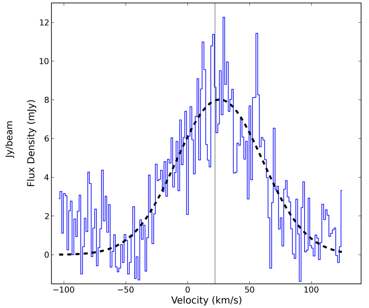
Fig. 8. Spectrum of \text{H}30\alpha line extracted from within a single beam centred upon the continuum peak location over-plotted with a Gaussian fit (dashed black). The velocity resolution is 1.4 \text{ km s}^{-1} . The line is centred at 22.1 \text{ km s}^{-1} the V_{\text{LSR}} of G17.64 as indicated by the vertical grey line. The base flux level for the Gaussian fit was fixed to zero. The line is weak compared to the other O-star sources (Cesaroni et al. 2017) but is exceptionally broad, with a FWHM of \sim 81.9 \pm 1.7 \text{ km s}^{-1} .
