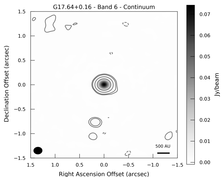
Fig. 1. ALMA band 6 (1.3 mm) continuum image of G17.64 made with a robust 0.5 value. The contour levels are set at -3, 5, 10, 50 and 200\sigma ( 1\sigma = 0.07 mJy beam -1 ) to indicate the weak southern sources and the strength of G17.64 (negative contours are dashed lines). The map is centred (0,0) on G17.64 at J2000 18^{\text{h}}22^{\text{m}}26.385^{\text{s}} -13^\circ30'11.97'' . The synthesised beam is indicated to the bottom left of the figure, while a scale bar is shown in the bottom right.
