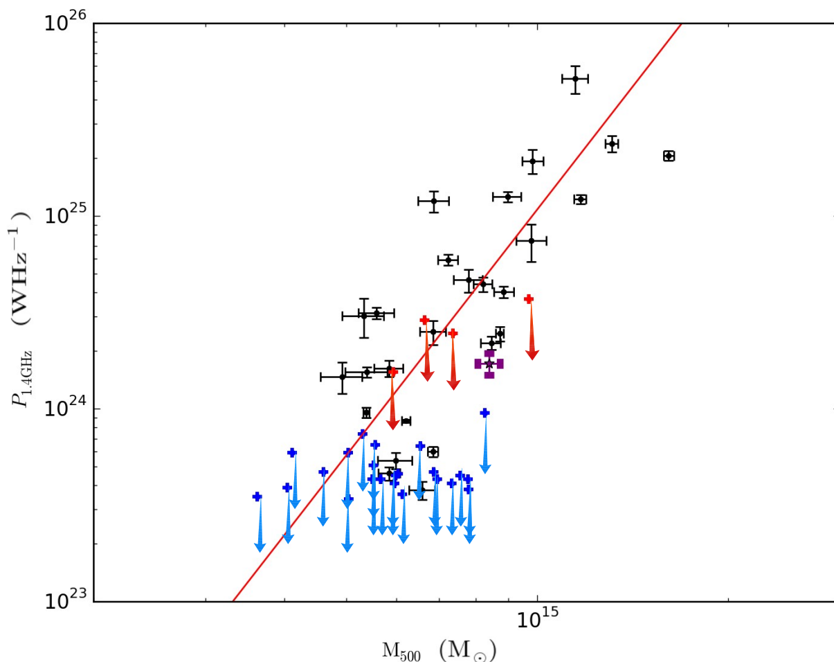
Fig. 4. Synchrotron power of RHs at 1.4 GHz ( P_{1.4GHz} ) vs. cluster mass M_{500} (from Planck Collaboration et al. 2016). Detected radio halos reported in the literature measured at 1.4 GHz (see Martinez Aviles et al. 2016) are shown in black dots. The red line is the best fit for the black dots. The purple star corresponds to the radio halo on PSZ2 G284.97-23.69. The blue arrows correspond to detection limits appearing in Cassano et al. (2013) and references therein. The red arrows are the upper limits for the non-detections presented in this paper (see Table 4).
