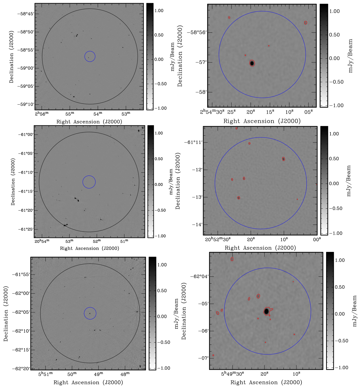
Fig. A.2. Same as Figure A.1. Top: PSZ2 G277.76-51.74; Middle: PLCK G334.8-38.0; Bottom: PSZ2 G271.18-30.95.
