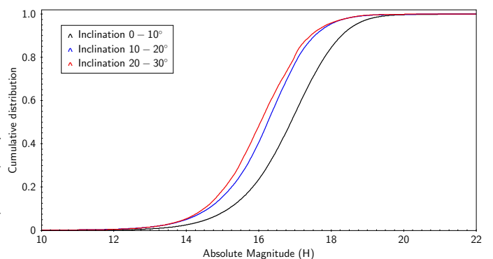
Fig. 14. Discovery bias toward high inclinations: The cumulative distributions of the absolute magnitudes of SSOs in the Asteroid Orbital Elements Database 10 (ASTORB, Bowell et al. 1993 ) for SSOs at different inclinations. A shift in the distribution toward brighter magnitudes for SSOs with higher inclinations is visible. This shows that the census for objects with high-inclinations is less complete, assuming a cumulative size distribution of the SSOs in the shape of a power-law ( Terai et al. 2013 ; Dohnanyi 1969 ; Gladman et al. 2009 ).
