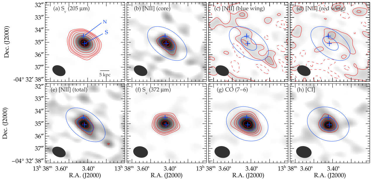
FIG. 1.— Surface brightness images: (a) the continuum at \sim 205 \mu\text{m} (rest frame); the [N II] line emission integrated over (b) the core frequency range from 270.021 to 270.472 GHz (243 to -257 \text{ km s}^{-1} ), (c) the blue wing (270.472 to 270.742 GHz or -257 to -557 \text{ km s}^{-1} ), (d) the red wing (269.751 to 270.021 GHz or 543 to 243 \text{ km s}^{-1} ), or (e) the full frequency range from 269.751 to 270.742 GHz; (f) the continuum at \sim 372 \mu\text{m} (rest frame); (g) the CO (7–6) emission integrated from 148.902 to 149.449 GHz (543 to -557 \text{ km s}^{-1} ); and (h) the [C I] 370 \mu\text{m} emission integrated from 149.499 to 149.847 GHz (320 to -377 \text{ km s}^{-1} ). In each panel, the image and the red contours refer to the same data; the image stretch is from 0 to the highest contour plotted except for panels (c) and (d), in which the gray scales are the same as in panel (b). All the contours start at 3\sigma , except for those in panels (c) and (d). In units of \text{mJy beam}^{-1} , the contours are shown at [3, 5, 7, 12, 24, 48, 96, 120] \times 0.057 in (a) or at [3, 5, 7, 12, 24, 27.6] \times 0.038 in (f). In units of \text{Jy km s}^{-1} \text{ beam}^{-1} , the contours in (b), (e), (g) and (h) are plotted at [3, 5, 7, 7.7] \times 0.11 , [3, 5, 6.4] \times 0.17 , [3, 5, 7, 12, 19] \times 0.12 , and [3, 5, 7, 9] \times 0.092 , respectively. The contours in both (c) and (d) are at [-2, -1, 1, 2] \times \sigma , where \sigma = 0.08 \text{ Jy km s}^{-1} \text{ beam}^{-1} , and the contours of negative values are shown in dashed line. The black ellipse at the lower left corner in each panel indicates the relevant (FWHM) synthesized ALMA beam. The blue ellipses in each line image indicate respectively the two apertures used for extracting the 1d spectra in Fig. 3. The two blue crosses in each panel mark the locations of sources N and S (see the text). The 5 kpc scale is shown in panel (a).
