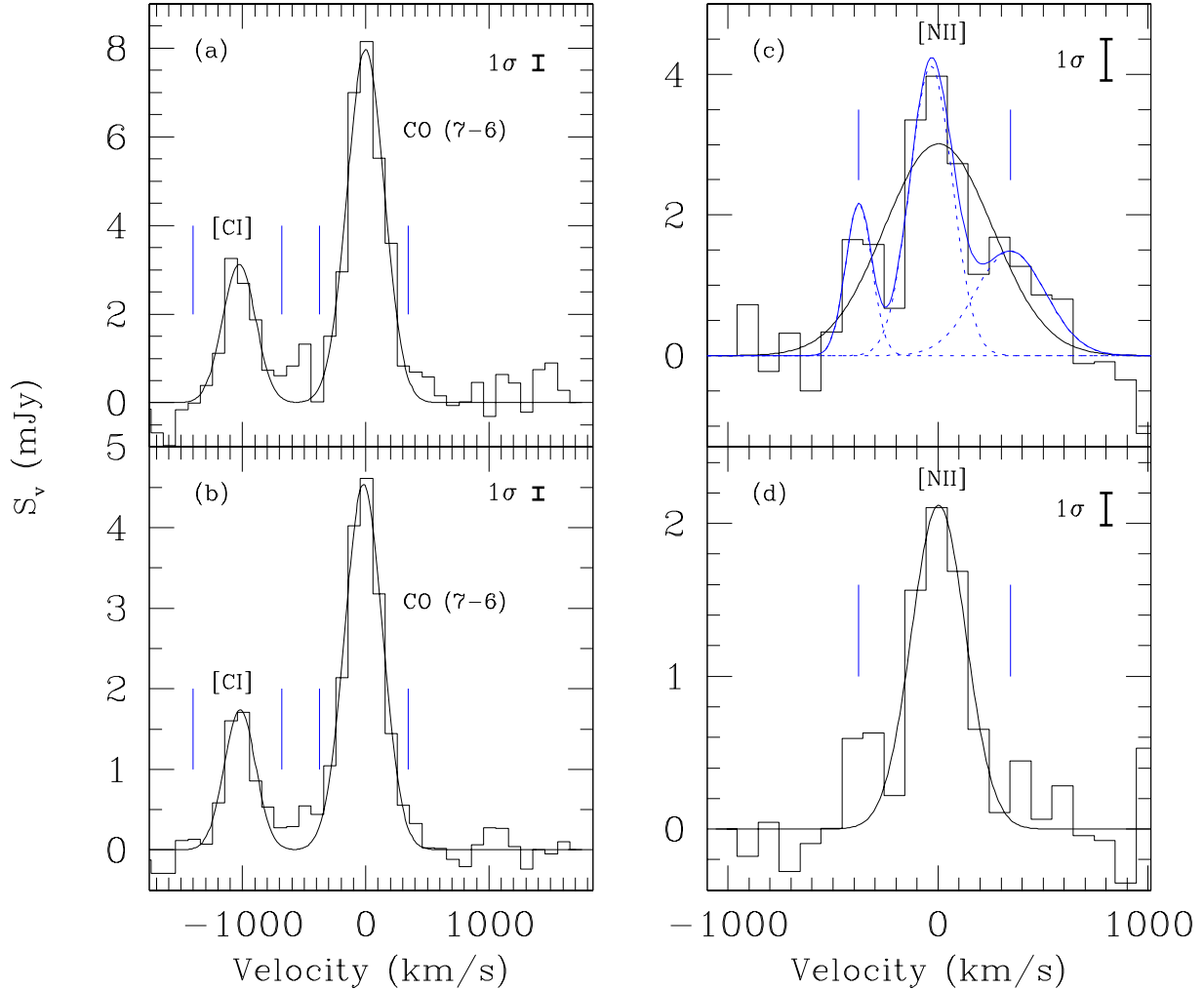
FIG. 3.— Extracted 1d spectra from the CO (7–6) (left panels) and [N II] (right panels) spectral cubes, respectively, using an elliptical aperture of the size index n = 2.5 (upper panels) or n = 1.0 (lower panels). The aperture size index n (see the text) is the common stretch factor for the major and minor axes of the aperture relative to the reference ellipse defined by the 2d Gaussian fit to the frequency-integrated line image. The velocity scales are with respect to the CO (7–6) and [N II] line central frequencies (in Table 1), respectively. Therefore, the observed central frequency of the [C I] line is located at -1,025 \text{ km s}^{-1} . The black solid curve in each panel is the best fit to the spectrum using either one or two Gaussian functions assuming zero residual continuum. The blue solid curve in panel (c) is a 3-component Gaussian fit to the spectrum with the individual components shown by the dotted curves in blue. For each spectral line, a pair of blue vertical bars mark the velocities of the peaks of the two minor Gaussian components of the [N II] emission in panel (c). The estimated 1\sigma error bar is shown in each panel.
