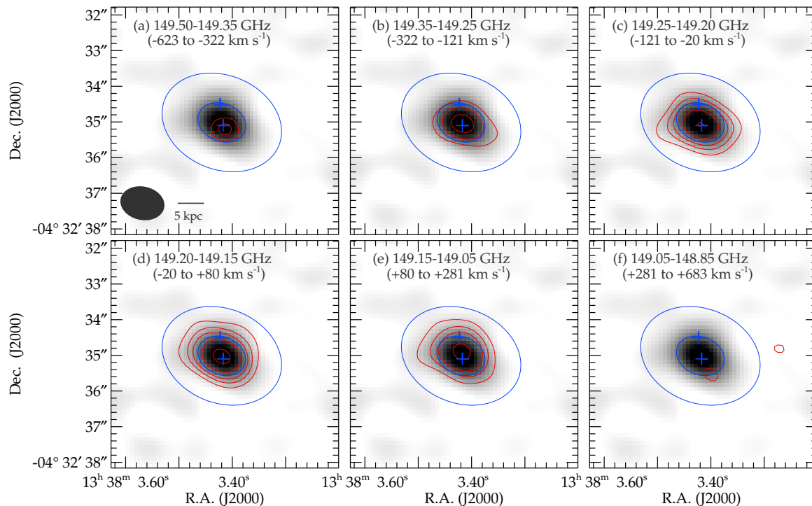
FIG. 4.— Velocity channel images of the CO (7–6) line emission with the channel frequency and velocity ranges noted in each panel. The gray image is always the total CO (7–6) image from Fig. 1g. Starting at 3 \times the r.m.s. noise and being in units of \text{Jy beam}^{-1} \text{ km s}^{-1} , the contour levels are: (a) [3.0, 3.6] \times 0.052 , (b) [3, 6, 9] \times 0.046 , (c) [3, 6, 9, 15, 22] \times 0.027 , (d) [3, 6, 9, 15, 22] \times 0.028 , (e) [3, 6, 9, 15] \times 0.041 , and (f) [3.0] \times 0.049 . The other over-plotted symbols are the same as in Fig. 1.
