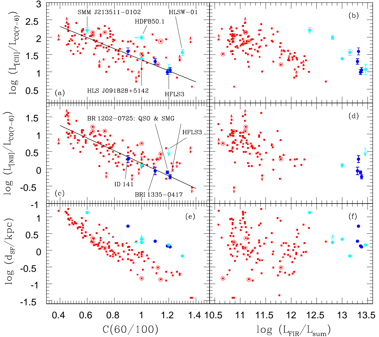
FIG. 6.— Plots of \log L_{\text{CII}}/L_{\text{CO}(7-6)} (top panels), \log L_{\text{NII}}/L_{\text{CO}(7-6)} (mid panels) and \log d_{\text{SF}} (bottom panels) as a function of the FIR color (left panels) or \log L_{\text{FIR}} (right panels), for the local (U)LIRG sample (filled squares in red) and a number of distant ULIRGs at 2 < z < 6.5 (filled circles in cyan or blue) from Lu et al. (2015), which also has an explanation for the labelling of the high- z galaxies here. The data points further circled in red are the local (U)LIRGs, for which the AGN contribution is likely to dominate the bolometric luminosity based on a number of mid-IR diagnostics (see Lu et al. 2015). Those high- z targets that are also in our ALMA program are plotted in blue (Lu et al. 2017b and this work), including ID 141 for which we used C(60/100) and L_{\text{FIR}} from Cox et al. (2011), a gravitational de-magnification factor of 4.1 from Brusa et al. (2012) and our own [N II] line flux measurement in Cheng et al. (2018, in preparation). The solid lines in (a) and (c) represent the average correlation of the local sample given in Lu et al. (2017b). The value of d_{\text{SF}} is derived from the L_{\text{FIR}} -based SFR and C(60/100) as prescribed in Lu et al. (2015) and has an uncertainty of about a factor of 2.
