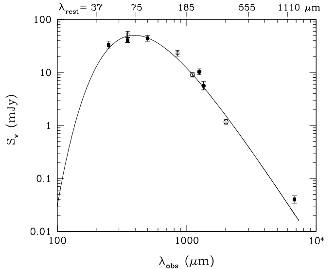
FIG. 5.— Plot of continuum flux measurements as a function of the observed wavelength. (The corresponding range of the rest-frame wavelength is indicated on the top.) Different symbols indicate the sources of the data: filled squares (Wagg et al. 2014), open squares (Benford et al. 1999), open circles (this work), and filled circles (Guiloteau et al. 1997). The solid curve is the best gray-body SED fit (with a fixed power-law emissivity index \beta = 1.8 ) to the data based on an equal weight basis, yielding T_{\text{dust}} = 41.5 K.
