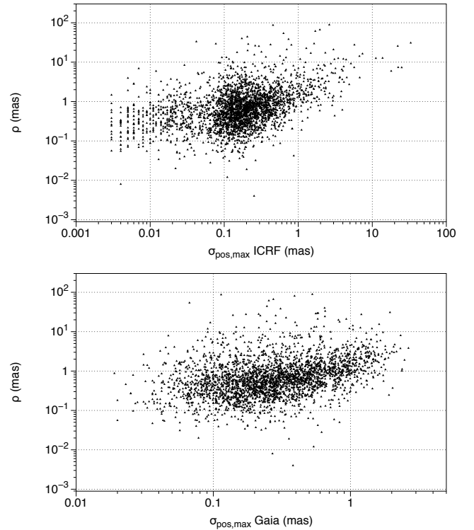
Fig. 17. Angular position differences \rho between Gaia DR2 and the ICRF3-prototype as function of the formal uncertainties \sigma_{pos,max} of the ICRF3-prototype (top) and Gaia DR2 (bottom).
