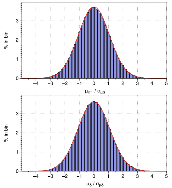
Fig. 10. Distributions of the normalised components of proper motions of the QSOs found with Gaia data, with \mu_{\alpha^*} (top) and \mu_\delta (bottom). A normal distribution with zero mean and standard deviation of 1.09 for \mu_{\alpha^*} (1.11 for \mu_\delta ) is drawn in red.
