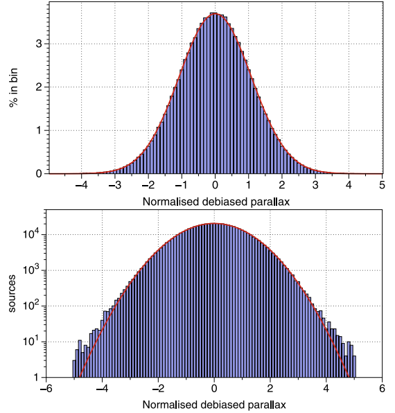
Fig. 9. Distribution of the normalised debiased parallaxes, (\varpi + 0.029 \text{ mas})/\sigma_\varpi , for the Gaia -CRF2 quasars in linear scale (top) and logarithmic (bottom). The red curve is a normal distribution with zero mean and standard deviation 1.08.
