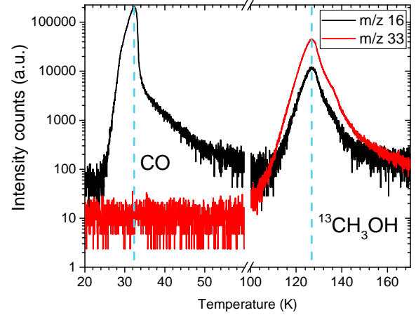
Fig. 2. Desorption profile of the 1:24 ^{13}\text{CH}_3\text{OH}:\text{CO} mixture, heated at 1\text{ K min}^{-1} . CO is traced by m/z 16 (black) and desorbs just above 30 K, while ^{13}\text{C} -methanol is traced by m/z 33 (red) and desorbs around 130 K. The presence of m/z 16 at the methanol desorption peak is due to the ^{13}\text{CH}_3 ( = 16\text{ amu} ) fragment.
