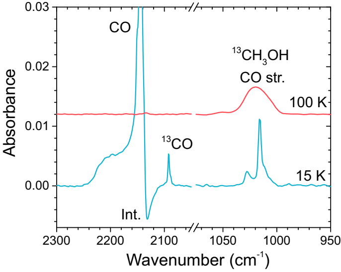
Fig. 1. Representative IR spectrum taken after deposition at 15 K (blue) of the 1:24 ^{13}\text{CH}_3\text{OH}:\text{CO} mixture and during the TPD at 100 K (red), showing the main IR features of CO and ^{13}\text{CH}_3\text{OH} . For the methanol CO stretch mode, the ^{13}\text{CO} and CO peak (cut-off due to its high peak intensity) are visible. Between the two CO peaks an artefact, labelled int., is visible caused by the high intensity of the CO peak.
