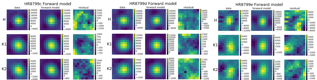
Figure 12. A summary of the forward model performance for HR 8799 c (left) d (middle) and e (right). Klipped data is shown to the left, the forward model is in the middle panel and the rightmost panel shows the difference between these two. Each image stamp is summed over the bandpass. Pixel values are in raw data units. Residual speckle noise appears to be influencing the K1 reduction of HR 8799 e.
