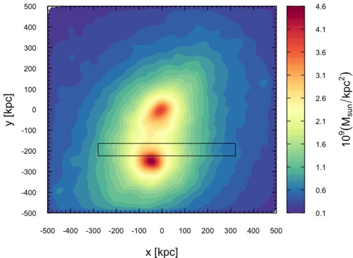
Figure 8. Total mass density distribution in the MUSIC simulated halo at z = 0.333 . The field of view is 1 \text{ Mpc}^2 and the colour coding indicates the mass density in 10^9 M_\odot / \text{kpc}^2 . The rectangular sector marks the region in which we compute the sector projected mass shown in Fig. 8.
