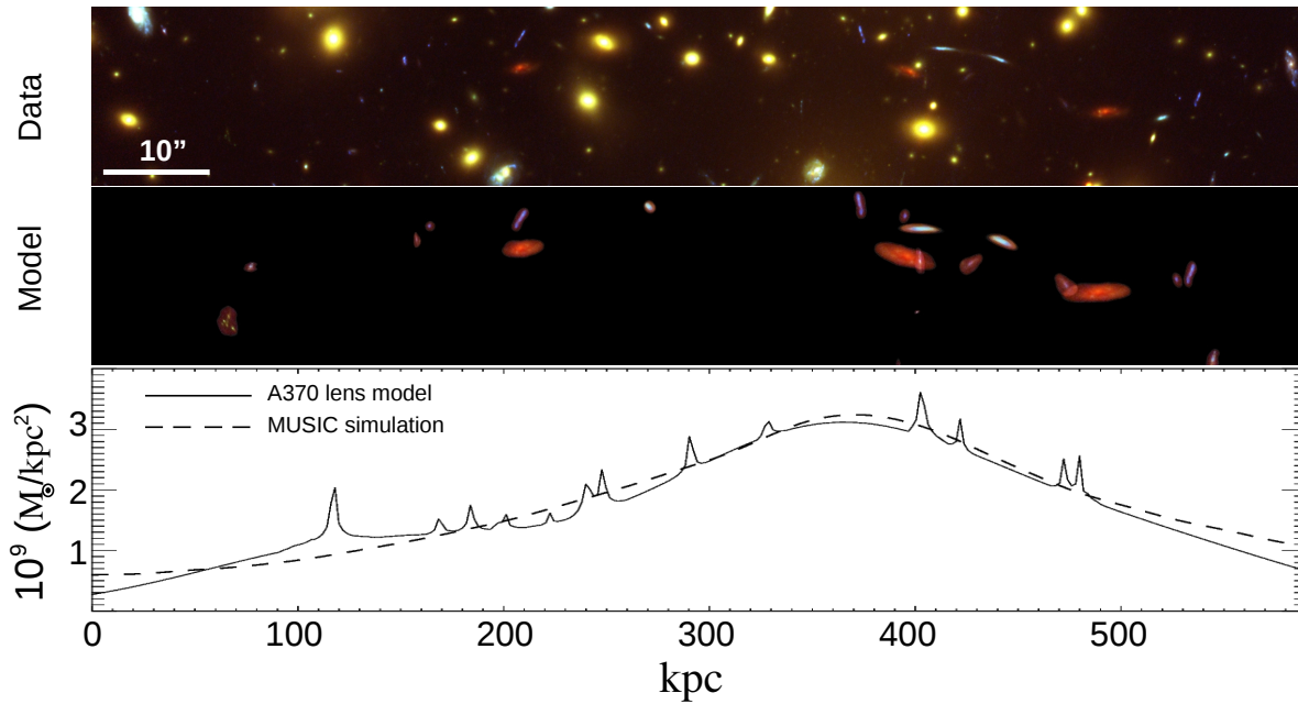
Figure 3. The top panel shows the rectangular sector highlighted in Fig.1. The middle panel shows the predicted lensed images based on the driver model. The bottom panel shows the average total mass projected along the vertical direction within the rectangular region.
