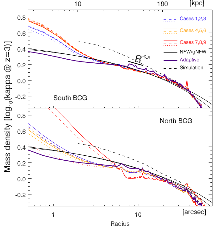
Figure 7. The total mass density (convergence) profile at z = 3 for the models centered on the BCG in the south (top panel) and centered on the BCG in the north (bottom panel). The coloured solid lines are for the cases 1,4 and 7 in table 1, the dashed lines are for cases 2, 5 and 8 and the dotted lines are for cases 3, 6 and 9. The black solid lines correspond to an NFW model (thick solid line) and a gNFW model (thin solid line). The NFW has a low concentration ( C = 2 ) and a virial radius = 3 Mpc. The gNFW model has the same virial radius but a larger concentration ( C = 4 ) compensated by a smaller inner slope ( \gamma = 0.9 ). The short solid line represents a power law R^{-0.3} . The NFW and gNFW models are the same in both panels for comparison purposes. The thick dark blue solid line corresponds to the alternative lens model discussed in section 8.1 (Case 10 in table 1). The black dashed line corresponds to the total mass (gas plus dark matter) profile of a simulation discussed in section 7. The total mass profile of the simulation below 10 kpc ( 2'' ) is not shown as it is below the smoothing length of the simulation.
