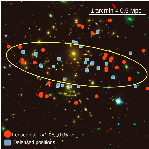
Figure 9. The red circles mark the observed positions of the galaxies in the narrow redshift interval z \in [1.0, 1.1] in the GLASS data. 80% of the GLASS data in this interval have Q_z > 2 . The squares mark the corresponding original positions in the source plane after deprojecting the observed positions with the driver lens model. A filament-like structure (marked with a yellow ellipse) can be hinted closer to (and behind) the northern BCG.
