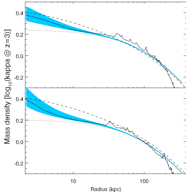
Figure 11. Stellar mass contribution to the BCGs. The solid lines correspond to the alternative model discussed in section 8.1 (shown also as thick dark blue solid lines in Fig. 7). The top panel shows the main BCG in the south and the bottom panel shows the secondary BCG in the north. The blue shaded region is the profile ( 3\sigma interval) from adding the estimated stellar mass to a dark matter toy model with a flat core (dotted lines). For comparison purposes we also show as dashed lines the NFW profile (with concentration parameter c = 2 ) of Fig. 7.
