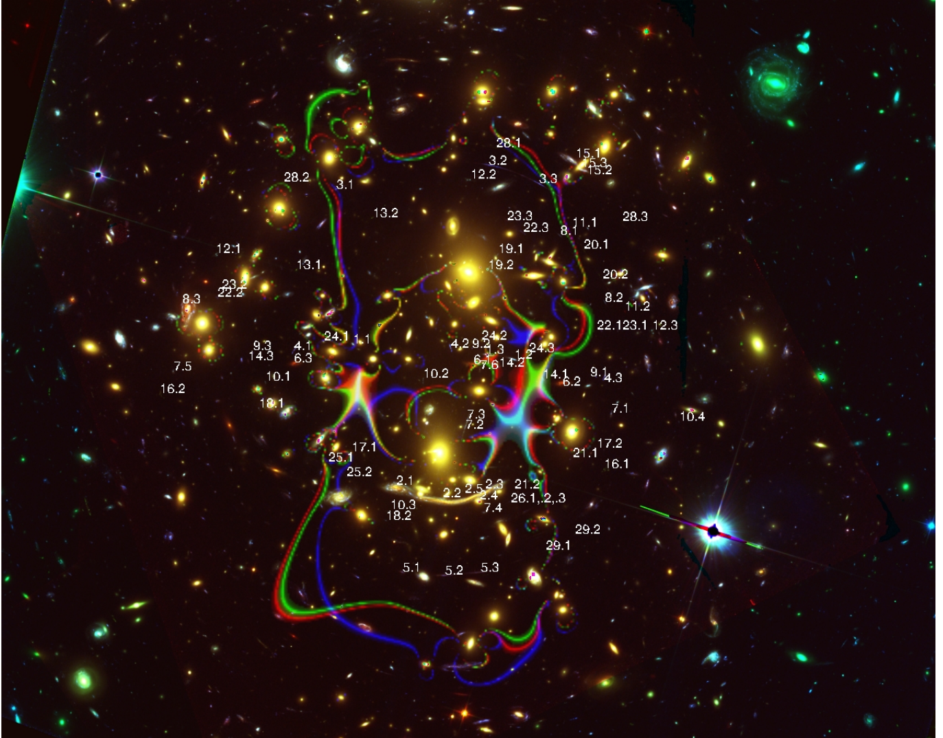
Figure 6. Critical curves for the Case 1 (blue), Case 2 (green), and Case 3 (red) lens model in Table 1. The systems used in this work are marked in their location (with small shifts in some of them to avoid overlap).
