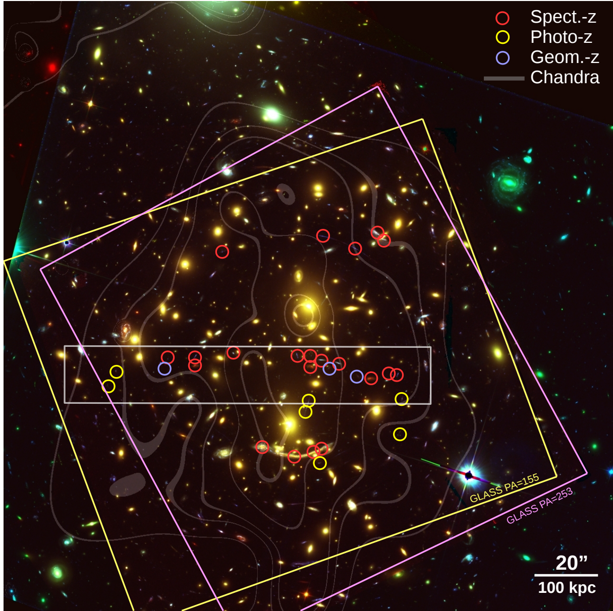
Figure 1. A370 as seen by HST (red=IR bands, green = F814W band and blue = F415W+F606W bands) with Chandra contours overlaid. The field of view is 3.2' . The circles mark the positions of the multiply lensed systems with spectroscopic, reliable photometric and/or reliable geometric redshift used to build the preliminary driver lens model. The gray central rectangular region marks the area with the highest density of reliable lensing constraints. The yellow and magenta square regions mark the field-of-view of the GLASS data at two position angles.
