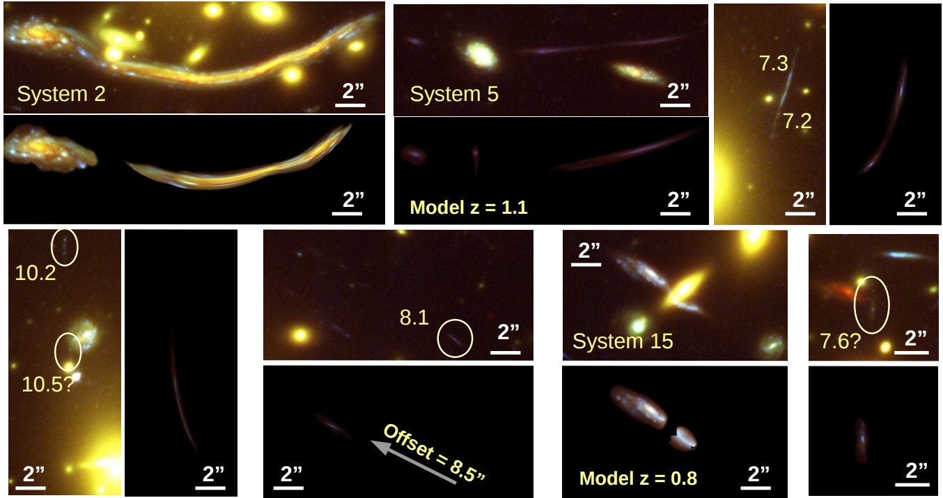
Figure 5. The driver model generally predicts the observed data with a high level of accuracy (Fig. 3). This figure compiles some of the exceptions where the model does not perform as well (see text for a detailed discussion of each case). The image candidate labeled as 7.6 is included in this figure is an example of the success of the model given the accurate agreement of the appearance and location of this image with our prediction (note its somewhat redder colour is due to the incomplete current coverage of the IR data used in making this colour figure).
