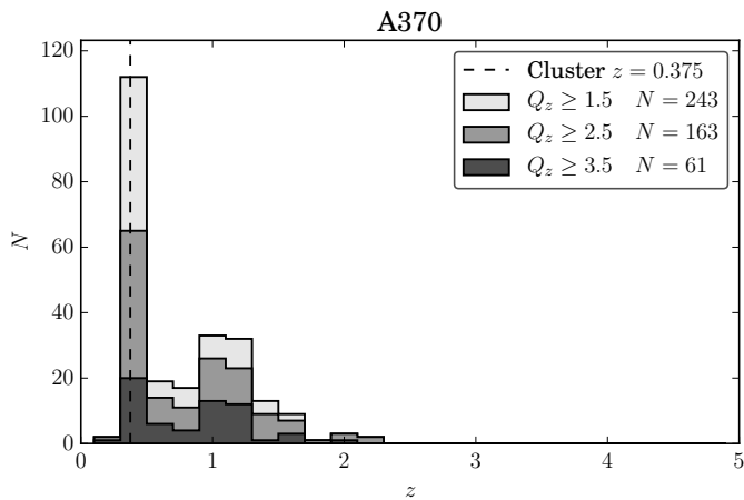
Figure 2. The redshift distribution of the publicly available GLASS v001 redshift catalog of A370. Q_z refers to the quality of the individual redshifts ( Q_z = 1 worst; Q_z = 4 best). Cluster members at z \sim 0.375 (vertical dashed line) are clearly separated from the rest of the sample. A second over-density of objects is apparent at z \sim 1 . This overdensity is discussed in Section 8.
