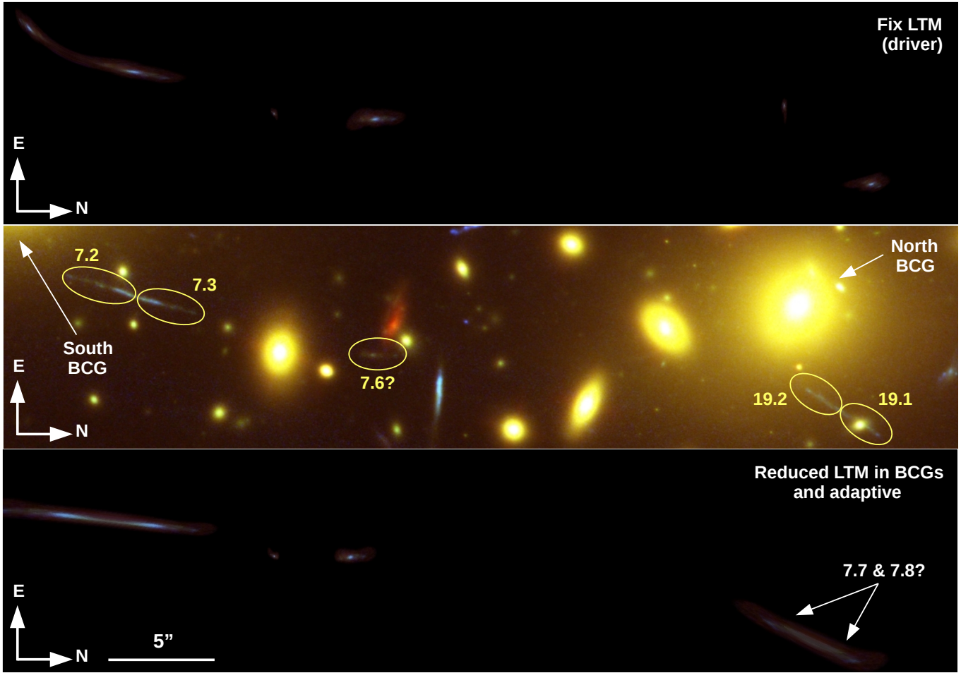
Figure 10. Central counterimages of system 7 as predicted by the driver model (top), as seen in the data (middle) and as predicted by the alternative multi-resolution model with reduced contribution from the BCGs (bottom). Note how the multi-resolution model straightens up the arc 7.2-7.3. The images are rotated 90^\circ (clockwise) with respect to the original image.
