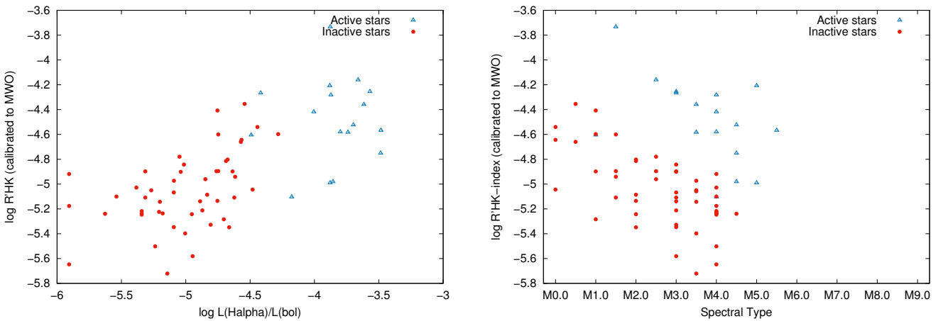
Figure 4. R'_{HK} values as a function of normalised H \alpha luminosity (left panel) and spectral type (right panel). All of values are calibrated to the S-index values obtained by the Mount Wilson Observatory (MWO).
