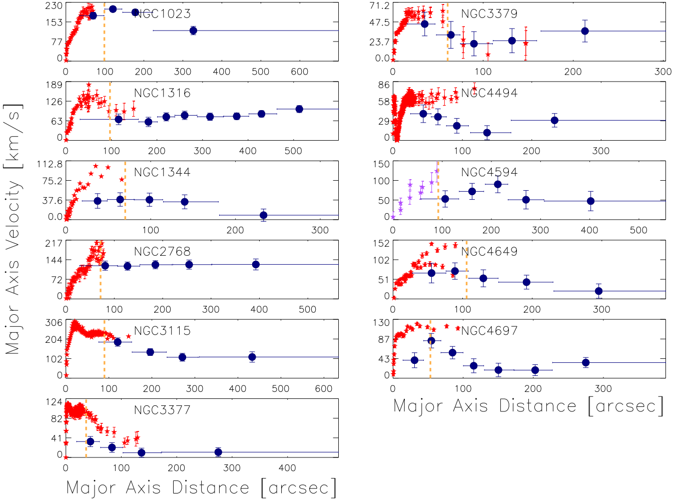
Fig. 6. Rotation velocity profiles for the fast rotators with highest number of tracers along the major axis. The full circles show the fitted amplitude V_{\text{maj,ax}} on the PN velocity fields. The red stars are stellar kinematics along the photometric major axis from the literature (references in table 1). The PN kinematics of NGC 4594 is compared with the stellar kinematics from a slit parallel to the major axis, offset by 30 arcsec (purple stars). The orange vertical lines mark the sizes of the photometric disks (see text). NGC 4494 shows a decrease in V_{\text{maj,ax}} , but there is no photometric evidence for a stellar disk. When the disk fades in the slowly rotating spheroid, the rotation velocity decreases. In addition, the PN rotation velocity may be lower than the values from absorption line spectroscopy at the same radii because of the smoothing that averages disk and spheroid PNe for near edge-on disks.
