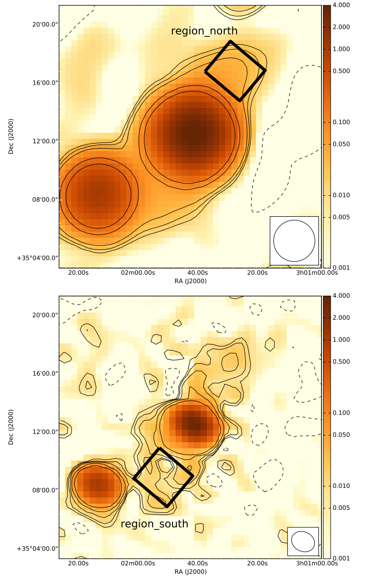
Fig. 3. Top - LOFAR image at 145 MHz convolved to 2.9-arcmin resolution. Contours represent -2, 2, 3, 5, 10, 20 \times \sigma ( 5 \text{ mJy beam}^{-1} ). Bottom - LOFAR image at 145 MHz and 80 \text{ arcsec} \times 98 \text{ arcsec} resolution. Contours represent -2, 2, 3, 5, 10, 20 \times \sigma ( 3 \text{ mJy beam}^{-1} ). The black regions represent the boxes used to extract the flux density in the Northern lobe and Southern lobe respectively. The colour scale is set in \text{Jy beam}^{-1} .
