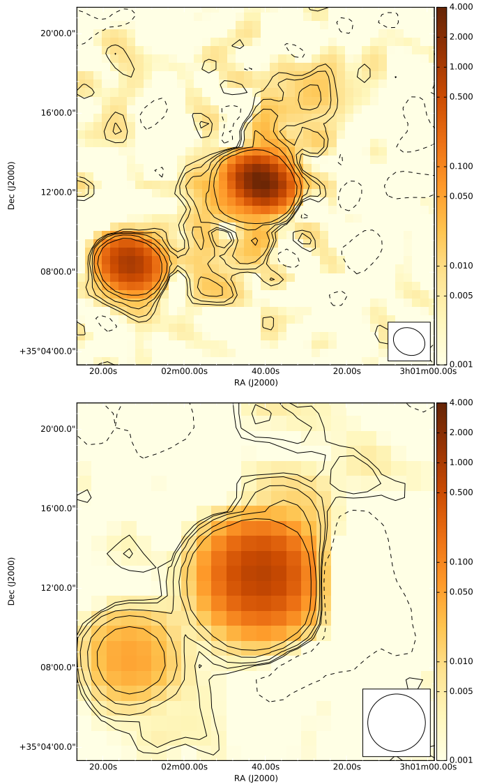
Fig. 2. Radio maps of the source B2 0258+35. Top: LOFAR 145-MHz map at 80 arcsec × 98 arcsec resolution. Levels: -2, 2, 3, 5, 10, 20 \times \sigma ( 3 mJy beam -1 ). Bottom: SRT 6600-MHz map at 2.9-arcmin resolution. Levels: -2, 2, 3, 5, 10, 20 \times \sigma ( 0.9 mJy beam -1 ). The colour scale is set in Jy beam -1 . In both panels the beam is shown at the bottom right corner.
