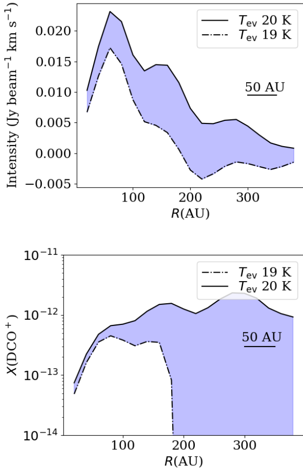
Fig. 3: The top panel shows the residual radial profiles from the models shown in Fig. 1 with an evaporation temperature of CO T_{\text{CO}}=19\text{K}-20\text{K} and a constant abundance X_{\text{in}}=5.0\times 10^{-5} . The bottom panel shows a vertically averaged abundance estimate of the radial curves of the top panel using the same excitation temperature profile and prescription proposed by Salinas et al. (2017) to convert emission to column densities. The 50 AU bar corresponds to the semi-minor axis of the synthesized beam and serves as a measure of the spatial resolution.
