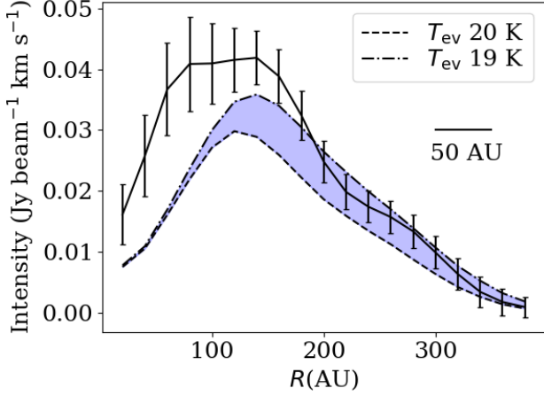
Fig. 1: The black continuous line shows the observed DCO + radial profile. These profiles are obtained by averaging the values of concentric ellipsoids of the integrated intensity maps. The error bars of the observed DCO + radial profile corresponds to 3\sigma , where \sigma is the standard deviation of the values contained in the ellipsoid divided by the square root of the number of beams. The 50 AU bar corresponds to the semi-minor axis of the synthesized beam and serves as a measure of the spatial resolution. The dashed lines show radial profiles of the emission from models with two different evaporation temperature of CO T_{\text{CO}}=19\text{-}20 K and a constant abundance X_{\text{in}}=5.0\times 10^{-5}
