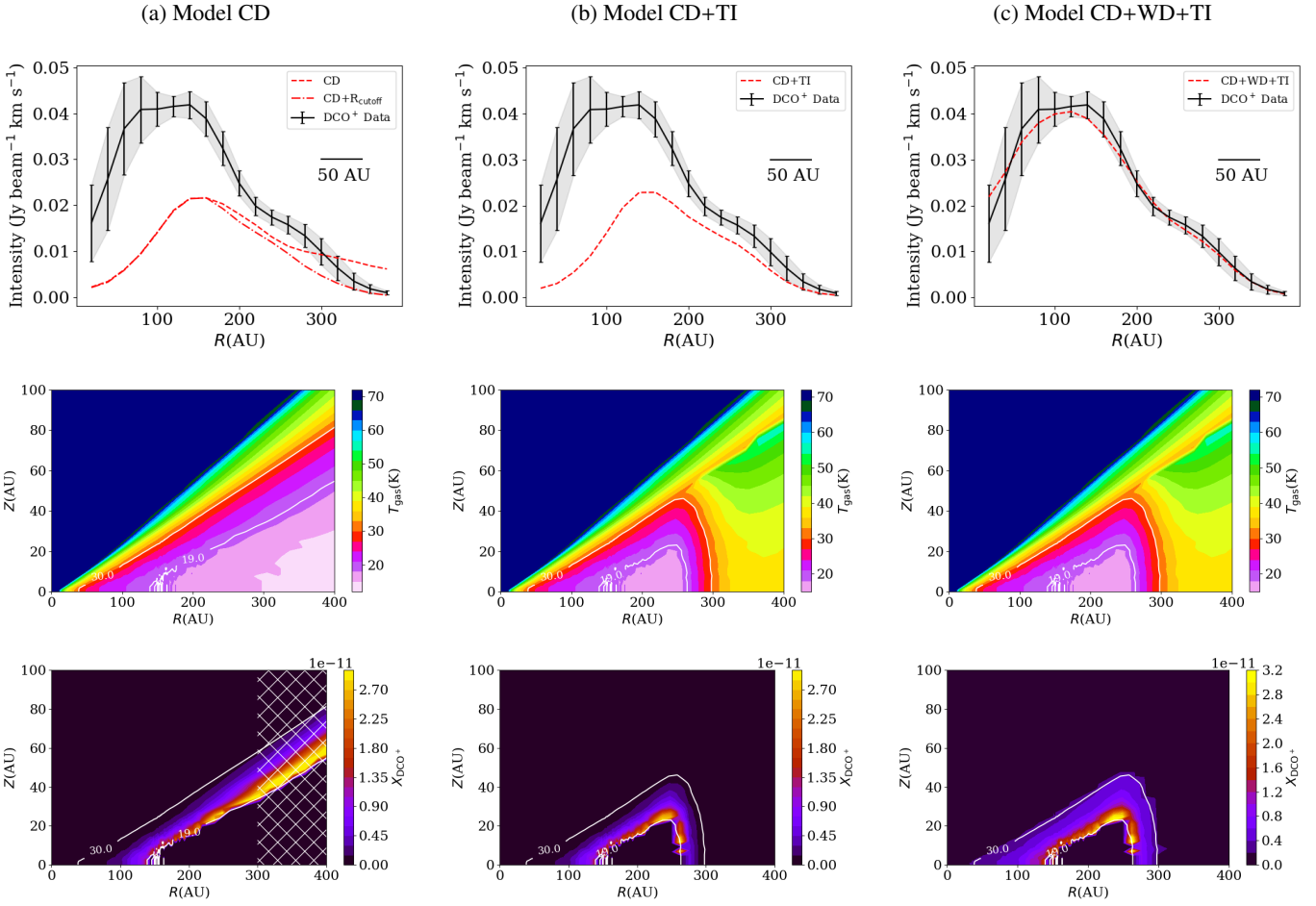
Fig. 4: The top panels show the resulting radial profile of the DCO + integrated intensity map of both models and data. The error bars on the data corresponds to 3\sigma , where \sigma is calculated as the standard deviation of a single ellipsoid divided by the square root of the number of beams. The middle panels show the models' temperature profile with contours at 19 and 30 K. The bottom panel shows the DCO + abundance profile over-plotted with temperature contours at 19 and 30 K. The hatched region in the DCO + abundance from model CD marks the radial cut off used in our standard model to reproduce the absence of emission at R > 300 AU.
