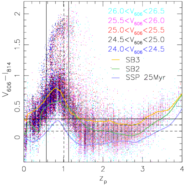
Figure 4. V_{606} - I_{814} colours of galaxies in the CANDELS fields as function of the peak photometric redshift z_p from S14. The colour coding splits the galaxies into our different magnitude bins. The horizontal lines mark our different colour cuts (dependent on cluster redshift and galaxy magnitude, see Sect. 6.2), while the vertical lines indicate the cluster redshift range 0.57 \leq z \leq 1.13 (solid), as well as z = 1.01 (dashed), at which cluster redshift the colour cuts change. The curves indicate synthetic V_{606} - I_{814} colours of galaxy SED templates from Coe et al. (2006).
