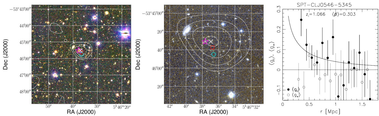
Figure G4. Weak lensing results for SPT-CL J0546-5345. See the descriptions in the captions of Fig. 14 and Fig. 16 for details.
