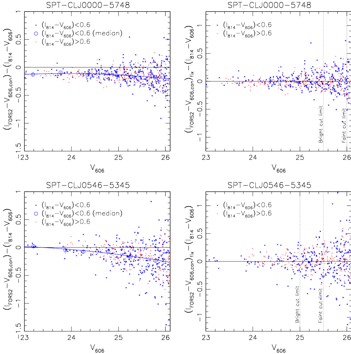
Figure D1. Details on the colour selection for SPT-CL J 0000–5748 ( top ) and SPT-CL J 0546–5345 ( bottom ): Left : Difference between the colour ( I_{\text{FORS2}} - V_{606,\text{con}} ) measured with the FORS2 I-band and the convolved HST/ACS F606W images, and the colour ( I_{814} - V_{606} ) measured from the unconvolved HST/ACS data in the inner cluster region, as function of V_{606} . Small blue crosses indicate blue galaxies with (I_{814} - V_{606}) < 0.6 , while red points show red galaxies with (I_{814} - V_{606}) > 0.6 . The open circles mark the median values for the blue galaxies within 0.5 mag wide magnitude bins, with error-bars indicating the uncertainty on the mean for a Gaussian distribution, and the curve showing their best-fit second-order polynomial interpolation. The right panels show the same data after subtraction of this function. We sample the photometric scatter distribution for the ACS-FORS2 selection from this distribution of offsets. Because of the lower scatter in the deeper FORS2 data of SPT-CL J 0000–5748 we can include fainter galaxies in the ACS-FORS2 selection than for SPT-CL J 0546–5345 (see Table 2 and the indicated bright/faint cut limits).
