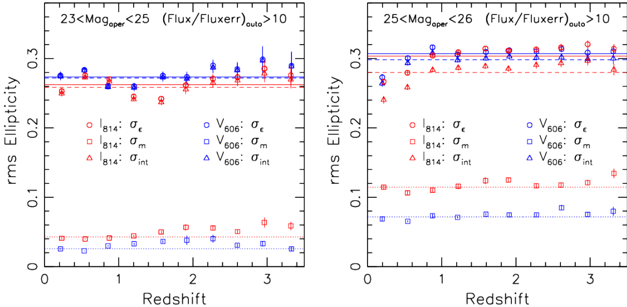
Figure A4. Galaxy ellipticity dispersion per ellipticity component as function of photometric redshift for bright 23 < \text{mag} < 25 galaxies (left), and faint 25 < \text{mag} < 26 galaxies (right). The horizontal lines show the weighted averages. See the caption of Fig. A1 for further details.
