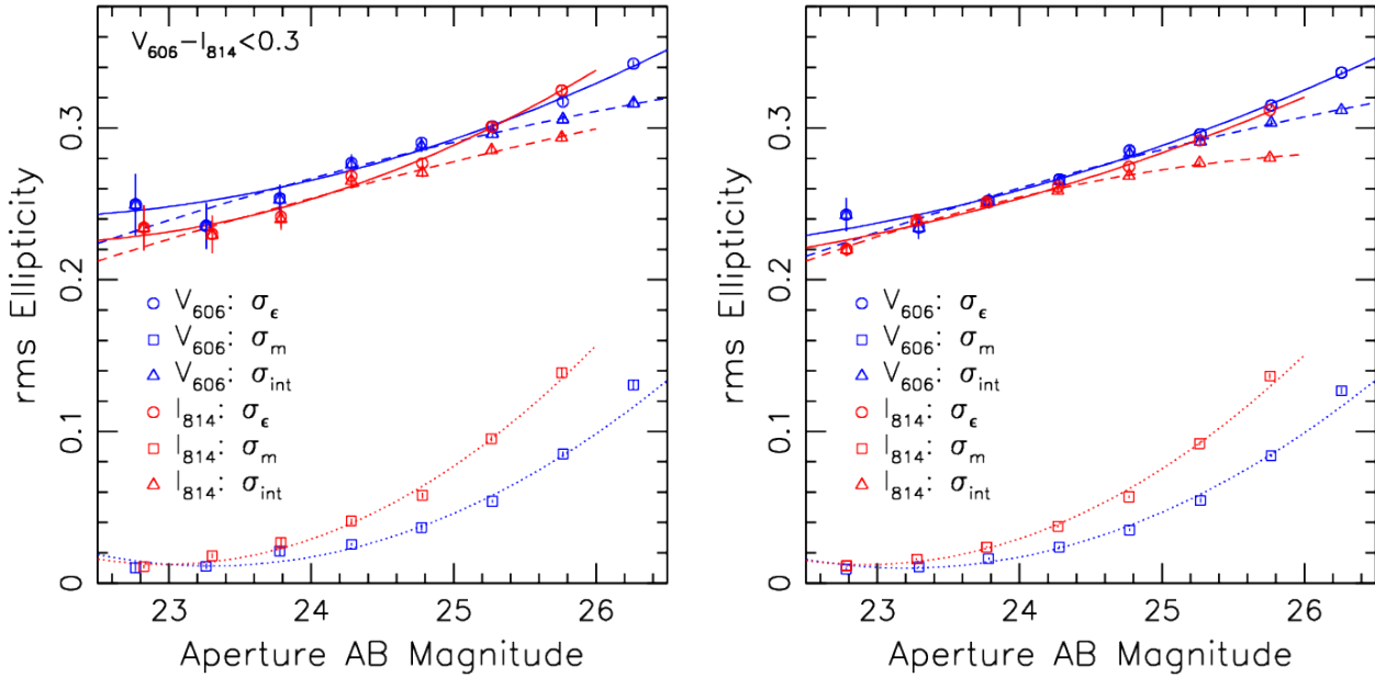
Figure A2. Galaxy ellipticity dispersion per ellipticity component as function of AB magnitude V_{606} or I_{814} . See the caption of Fig. A1 for further details.
