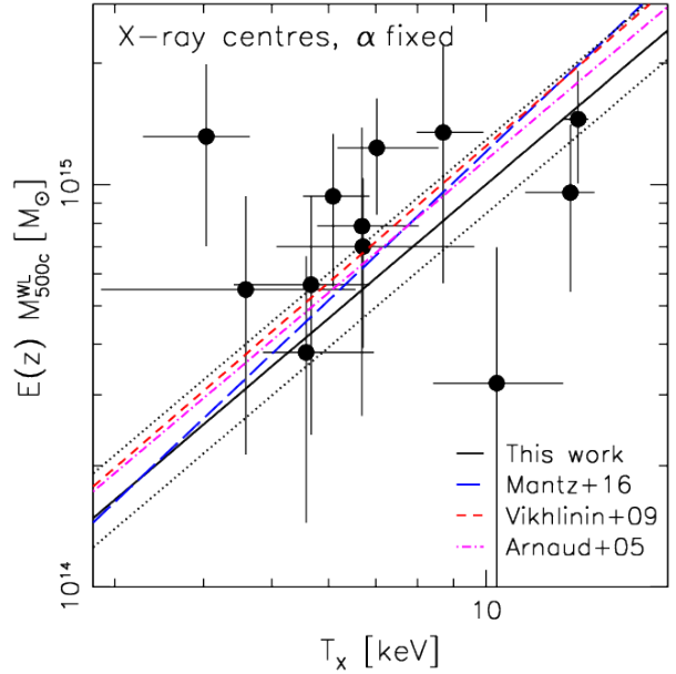
Figure 19. Core-excised X-ray temperatures measured in the range (0.15-1) \times r_{500c} based on Chandra data versus E(z)M_{500c}^{WL} from the weak lensing analysis using the X-ray centroids and assuming the M - c relation from Diemer & Kravtsov (2015). The solid black line shows our best-fit estimate of the scaling relation when assuming a fixed slope \alpha = 3/2 . The dotted lines correspond to normalisations that are lower or higher by 1\sigma , combining the statistical and systematic uncertainties of our constraints. The dashed and dashed-dotted lines indicate best-fit estimates derived by Arnaud, Pointecouteau & Pratt (2005); Vikhlinin et al. (2009a) and Mantz et al. (2016).
