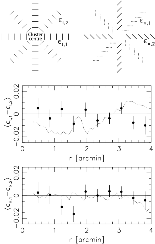
Figure 2. Testing for residual CTI systematics in the cluster fields: Top: Illustration of the separation of the tangential and cross components of the ellipticity into components affected by CTI ( \epsilon_{t,1} , \epsilon_{x,1} ), and those unaffected by CTI ( \epsilon_{t,2} , \epsilon_{x,2} ). The middle (bottom) panel shows the difference in the tangential (cross) ellipticity component with respect to the cluster centre as estimated from the CTI-affected and the CTI-unaffected components. Here we combine the signal from all galaxies passing the shape cuts with 24 < V_{606, \text{auto}} < 26.7 in all cluster fields. The points are consistent with zero ( \chi^2/\text{d.o.f.} = 0.96 ) suggesting that the CTI has been fully corrected within the statistical precision of the data. For comparison, the dotted curve shows the signal which would be measured from an uncorrected CTI saw-tooth ellipticity pattern with \langle \epsilon_1 \rangle = -0.05 , where small wiggles are caused by the sampling at the galaxy positions and the masks applied.
