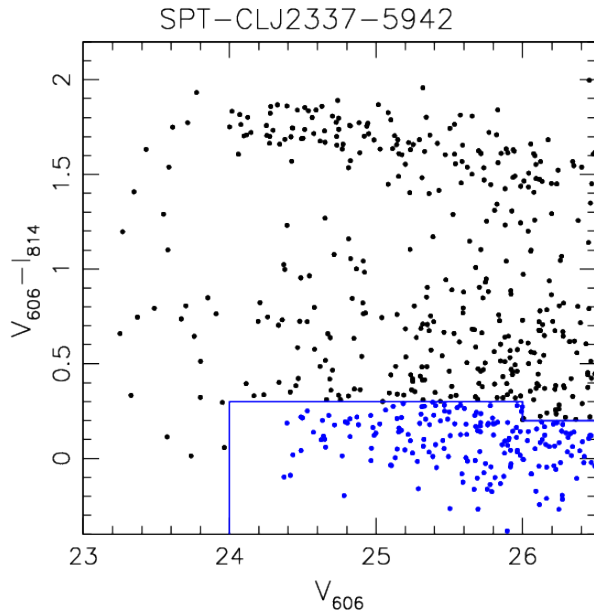
Figure 3. Measured V_{606} - I_{814} colours as function of V_{606} for galaxies in the field of SPT-CL J2337-5942 that pass our weak lensing shape cuts, and that are located within the central I_{814} ACS tile. The blue lines indicate the region of blue galaxies that pass our colour selection. The cluster red sequence is clearly visible at V_{606} - I_{814} \sim 1.7 .
