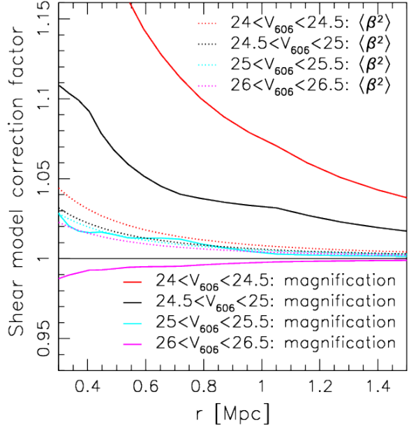
Figure 11. Correction factors to the reduced shear profile model of a M_{200c} = 7 \times 10^{14} M_{\odot} galaxy cluster at z_l = 0.87 due to the impact of magnification on the source redshift distribution (solid curves) and the finite width of the redshift distribution ( \langle\beta^2\rangle , see Eq. 12, dotted). The different colours correspond to different bins in the V_{606} aperture magnitude.
