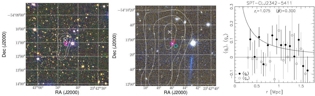
Figure G11. Weak lensing results for SPT-CL J2342–5411. See the descriptions in the captions of Fig. 14 and Fig. 16 for details.
