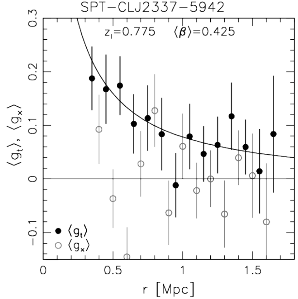
Figure 16. Tangential reduced shear profile (black solid circles) of SPT-CL J2337-5942 centred on the X-ray centroid and obtained by combining the profiles of all contributing magnitude bins of the ACS-only plus the ACS+FOR2 selection (see Sect. 7.2). The curve shows the correspondingly-combined best-fitting NFW model prediction obtained by fitting the data in the range 500 \text{ kpc} \leq r \leq 1.5 \text{ Mpc} and using the Diemer & Kravtsov (2015) mass-concentration relation. The grey open circles indicate the 45 degrees-rotated reduced cross-shear component, which is a test for systematics, shifted by dr = -0.05 \text{ Mpc} for clarity. The corresponding plots of the other clusters are shown in Appendix G.
