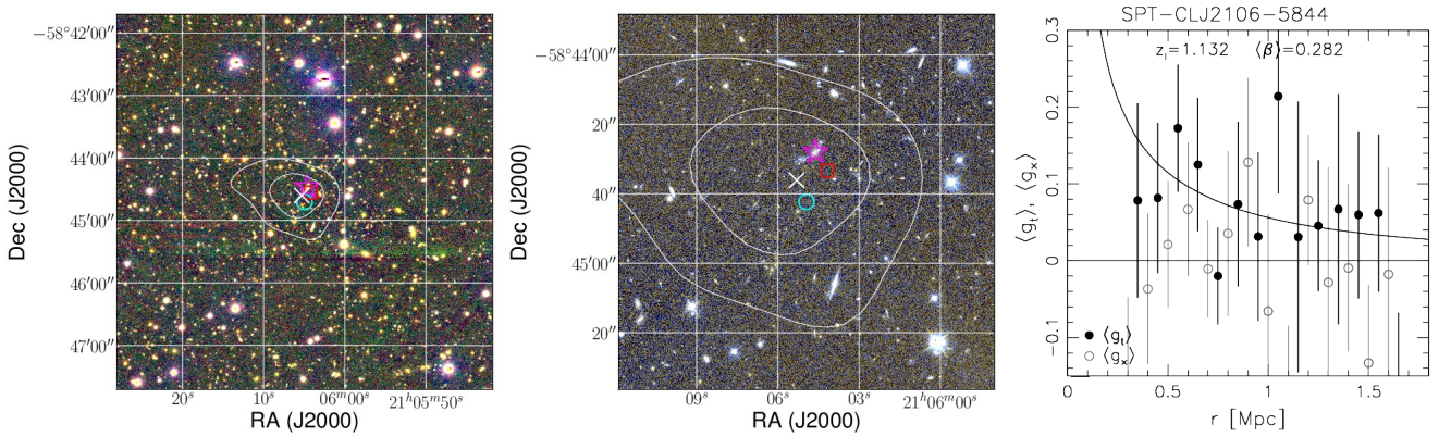
Figure G8. Weak lensing results for SPT-CL J2106–5844. See the descriptions in the captions of Fig. 14 and Fig. 16 for details.
