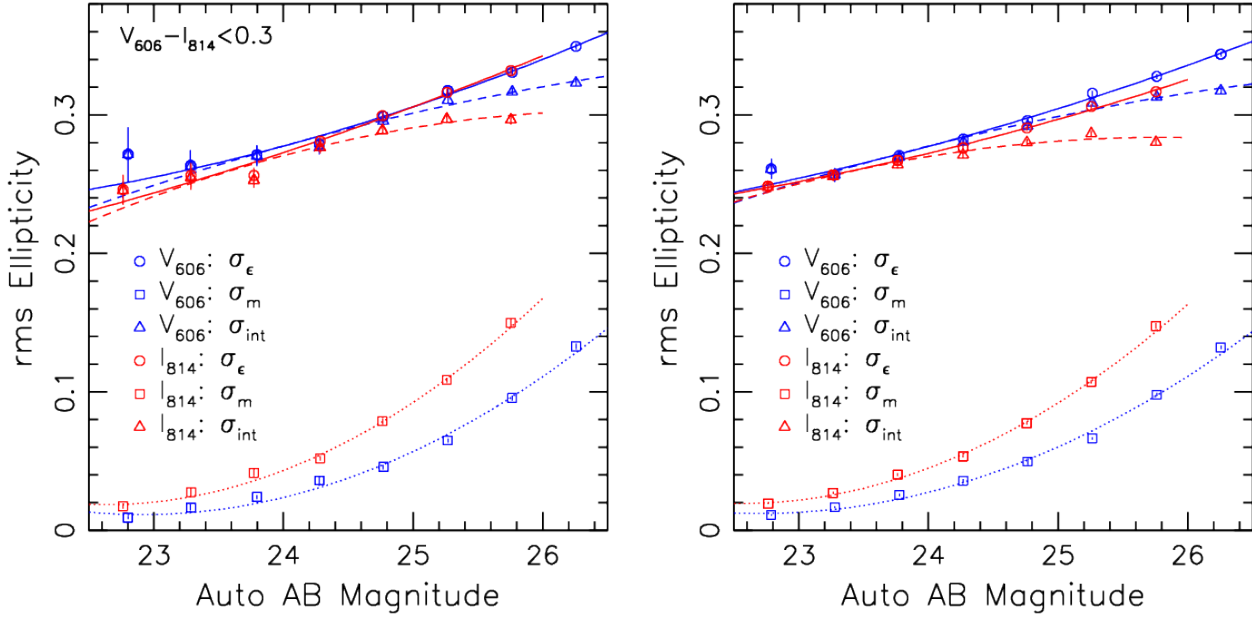
Figure A3. Galaxy ellipticity dispersion per ellipticity component as function of AB auto magnitude from SExtractor. See the caption of Fig. A1 for further details.
