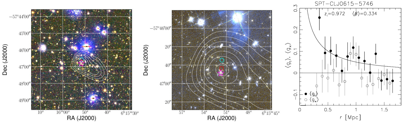
Figure G6. Weak lensing results for SPT-CL J0615–5746. See the descriptions in the captions of Fig. 14 and Fig. 16 for details.
