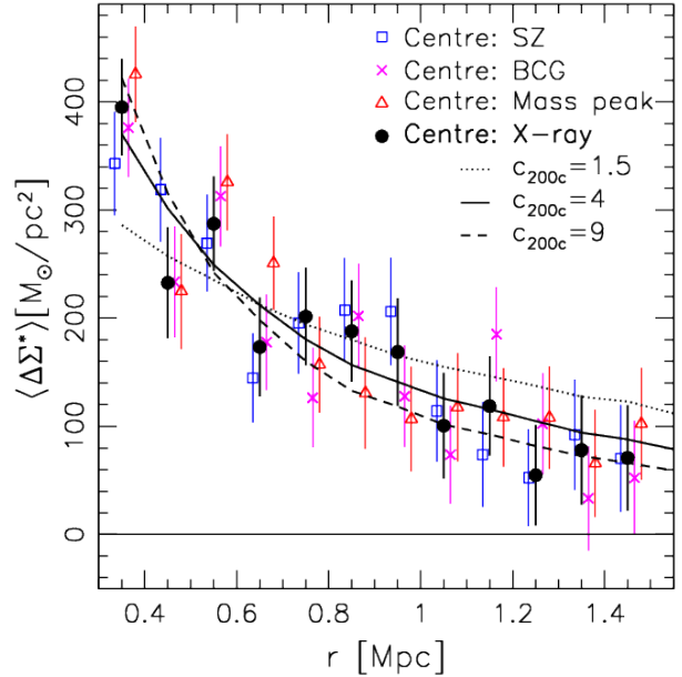
Figure 17. Weighted average of the rescaled differential surface mass density profiles from all clusters. The circles, squares, crosses, and triangles show the signal measured around the X-ray centroids, the SZ peak positions, the BCG locations, and the weak lensing mass peaks, respectively. The circles showing the signal around the X-ray centroids are displayed at the correct radius, while the other symbols are shown with a horizontal offset for clarity. The curves show the correspondingly averaged best-fit model predictions for different fixed concentrations for the analysis employing the X-ray centres and using an extended fit range 300 kpc to 1.5 Mpc, which increases the sensitivity for constraints on the average concentration.
