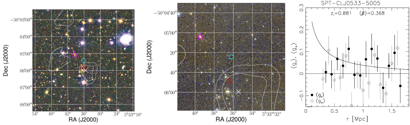
Figure G3. Weak lensing results for SPT-CL J0533-5005. See the descriptions in the captions of Fig. 14 and Fig. 16 for details.
