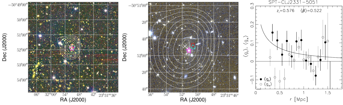
Figure G9. Weak lensing results for SPT-CL J2331–5051. See the descriptions in the captions of Fig. 14 and Fig. 16 for details.
