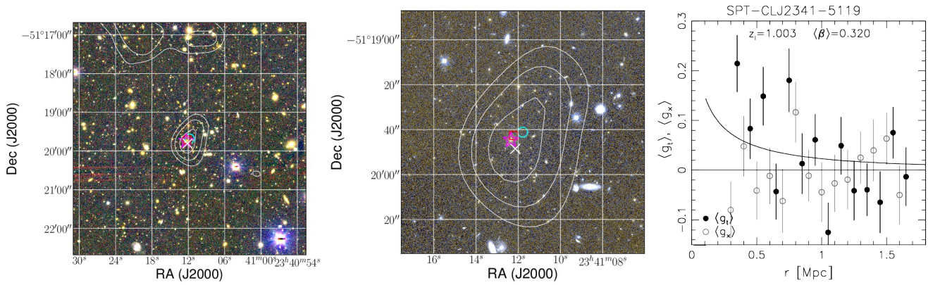
Figure G10. Weak lensing results for SPT-CL J2341–5119. See the descriptions in the captions of Fig. 14 and Fig. 16 for details.
