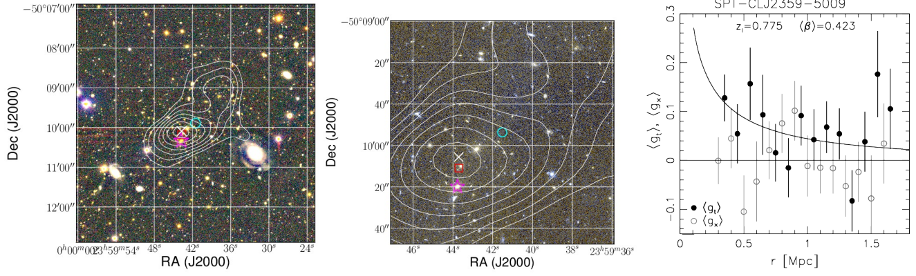
Figure G12. Weak lensing results for SPT-CL J2359–5009. See the descriptions in the captions of Fig. 14 and Fig. 16 for details.
