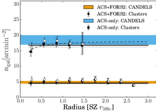
Figure 13. Density of sources n_{\text{gal}} for the ACS-only and ACS+FOR2 colour selections as function of cluster centric distance around the X-ray centre in units of r_{500c} , as estimated from the SZ signal. The profiles account for both masks and obscuration by cluster members. Solid (open) symbols include (do not include) the correction for magnification. The coloured regions indicate the one sigma constraints on the mean background density from the five CANDELS fields. Black solid and dotted lines show the maximum likelihood and 68% uncertainty range for a constant density model. The dashed line shows for the ACS-only selection the maximum likelihood contamination model following a 1/r functional form.
