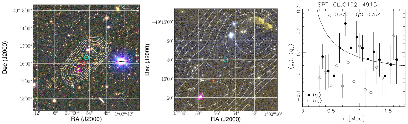
Figure G2. Weak lensing results for SPT-CL J0102–4915. See the descriptions in the captions of Fig. 14 and Fig. 16 for details.
