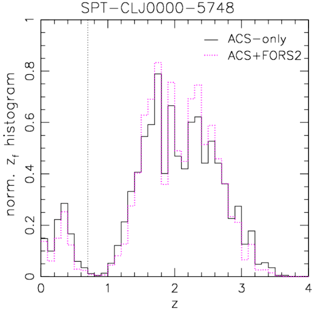
Figure 7. Normalised histogram of the statistically corrected photometric redshift estimates z_f for all galaxies in our CANDELS catalogues that pass the weak lensing cuts and the colour selection after adding noise to mimic the properties of the SPT-CL J0000–5748 data, both for the ACS+FORS2 (magenta dotted) and the ACS-only (black solid) selection. The vertical dotted line indicates the cluster redshift, at which both selections achieve an efficient suppression also in the presence of noise.
