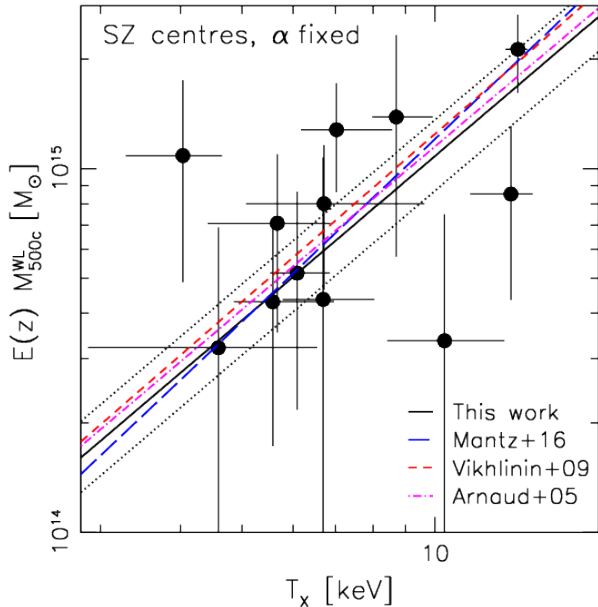
Figure 20. As Figure 19, but employing the weak lensing results for the SZ centres.
