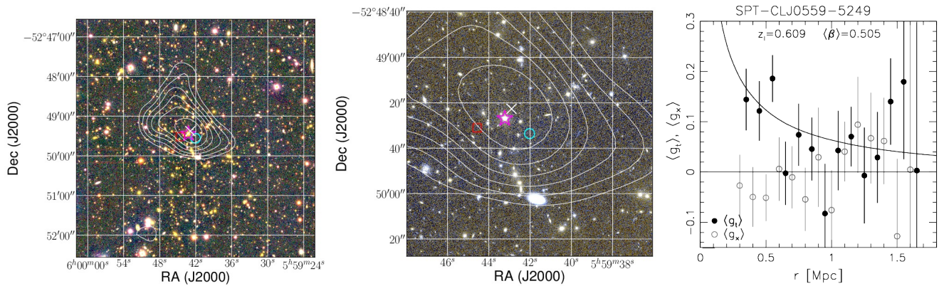
Figure G5. Weak lensing results for SPT-CL J0559-5249. See the descriptions in the captions of Fig. 14 and Fig. 16 for details.
