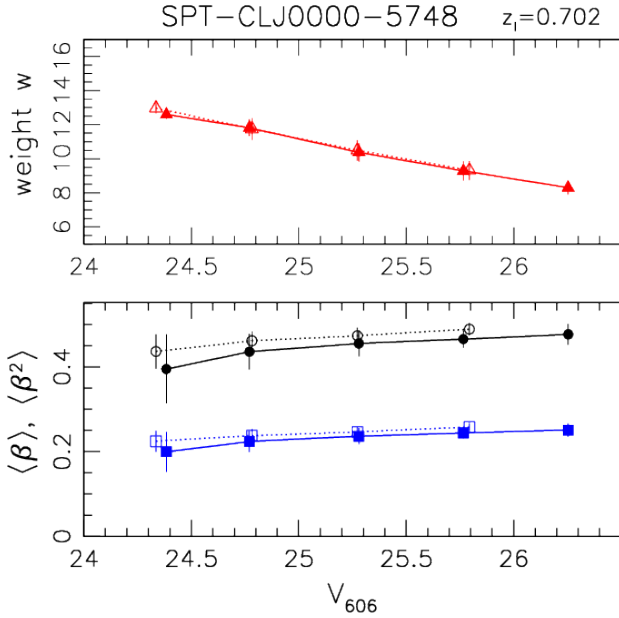
Figure 8. Analysis of SPT-CLJ0000-5748 as function of V_{606} magnitude, where the solid (open) symbols correspond to the ACS-only (ACS+FOR2) analysis. Top: Mean weak lensing shape weight w with error-bars indicating the dispersion from all selected galaxies in the magnitude bin. Bottom: \langle\beta\rangle (circles) and \langle\beta^2\rangle (squares) with error-bars showing the dispersion of their estimates computed from all CANDELS sub-patches (see Sect. 6.6), thus indicating the expected line-of-sight variations for the field sizes of our cluster observations.
