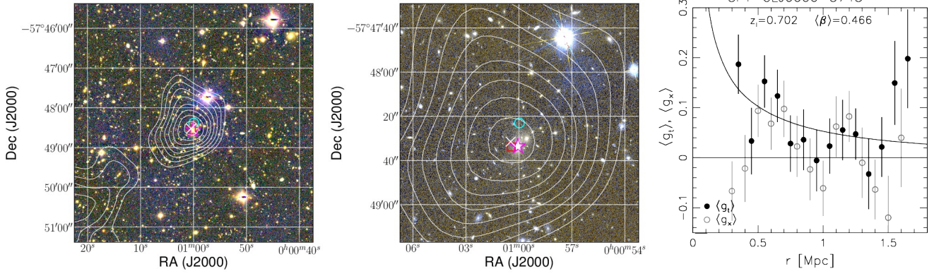
Figure G1. Weak lensing results for SPT-CL J0000–5748. See the descriptions in the captions of Fig. 14 and Fig. 16 for details.
