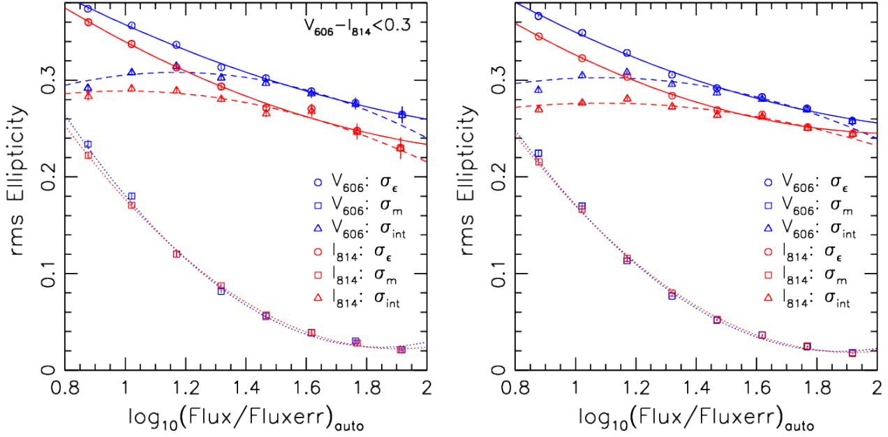
Figure A1. Galaxy ellipticity dispersion per ellipticity component as function of the logarithmic flux signal-to-noise ratio (measured by SExtractor as FLUX_AUTO/FLUXERR_AUTO ) with ( left ) and without colour selection ( right ), estimated from ACS F606W and F814W data in the CANDELS fields (see the text for details), and averaged over both ellipticity components. The circles show the r.m.s. of our KSB ellipticity estimates \sigma_\epsilon , with polynomial interpolations indicated by the solid curves. The squares show the measurement noise \sigma_m estimated from the difference between the ellipticity estimates in overlapping tiles, with polynomial interpolations indicated by the dotted curves. The triangles show the estimate for intrinsic shape noise \sigma_{\text{int}} = \sqrt{\sigma_\epsilon^2 - \sigma_m^2} , with polynomial interpolations indicated by the dashed curves. The symbols mark the bin centres, and error-bars indicate the uncertainty estimated via bootstrapping.
