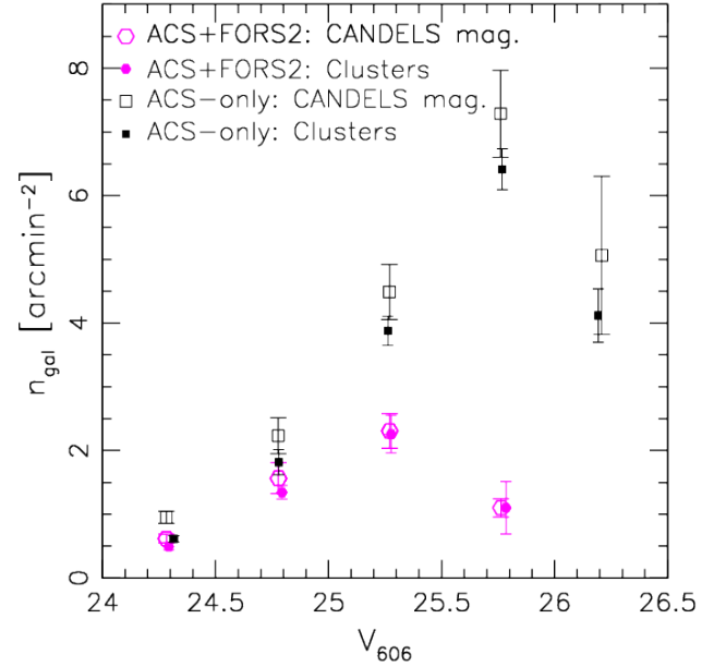
Figure 12. Selected source density n_{\text{gal}} as function of V_{606} accounting for masks and averaged over all the cluster fields (small solid symbols) and the corresponding source density averaged over the CANDELS fields when mimicking the same selection and accounting for photometric scatter and magnification (large open symbols). Black squares show the ACS-only selection, while magenta hexagons correspond to the ACS+FOR2 selection. We include only galaxies located within the fit range of the shear profiles (see Sect. 7.2) to avoid limitations of the magnification correction at small radii. The error-bars show the uncertainty on the mean from the variation between the contributing cluster fields or the five CANDELS fields, respectively, assuming Gaussian scatter. They are correlated between magnitude bins due to large-scale structure.
