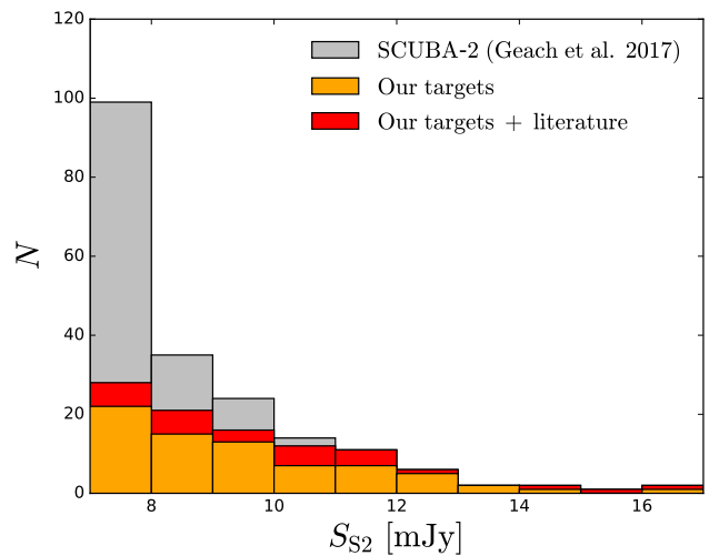
Figure 1. Histogram showing the debosted flux density distribution of the parent SCUBA-2 CLS survey from Geach et al. (2017) , our 75 targets, and our full catalogue including these 75 targets and 28 archival sources from Simpson et al. (2015) , Younger et al. (2007) , Younger et al. (2009) and Ikarashi et al. (2011) , which are included in our counts analysis. Our sample is a nearly complete selection of single-dish 850\text{-}\mu\text{m} SCUBA-2 sources with flux densities brighter than 10 mJy.
