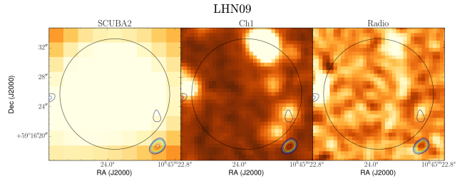
Figure 5. SMA flux density contours of LHN09, from 3\sigma to 6\sigma in steps of 0.5\sigma , overlaid over Spitzer -IRAC 3.6 \mu\text{m} , VLA 1.4 GHz and the parent SCUBA-2 850 \mu\text{m} images. We see a large offset between the peak SCUBA-2 850 \mu\text{m} flux density and the SMA detection. This could be due to the fact that this is a rather complicated field, with at least four IR galaxies and two radio galaxies all within the SCUBA-2 beam.
