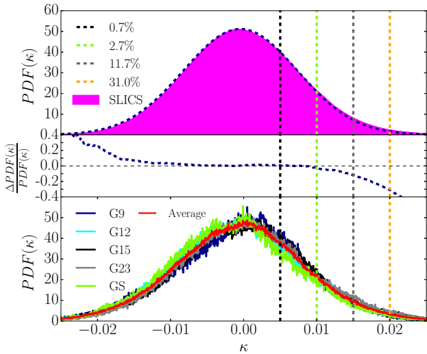
Figure 2. Upper: PDF of the convergence \kappa from 50 SLICS realisations in magenta and a Gaussian fit in dashed blue. The percentage deviations between the Gaussian fit and the PDF( \kappa ) at \kappa = (0.005, 0.010, 0.015, 0.020) , shown by the dashed lines, are detailed in the legend. Middle: the fractional difference between the Gaussian fit and the SLICS PDF( \kappa ). Lower: The PDFs of the five KiDS-450 patches and their average.
