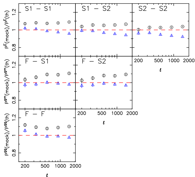
Figure B1. Ratio of power spectra measured on the numerical simulations and the theoretical power spectra. The top row shows the auto-correlation and cross-correlation of the cosmic shear power spectra for the two shape samples, the middle row shows the galaxy-matter power spectrum for one foreground sample and two shape samples, and the bottom row shows the angular power spectrum of the foreground sample. Open black circles (blue triangles) correspond to theoretical power spectra computed using the non-linear corrections of Smith et al. (2003) (Takahashi et al. (2012)). Error bars show the error on the mean of the different mock realisations.
