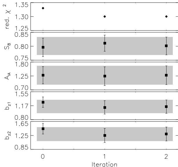
Figure D1. Constraints on the reduced \chi^2 value of the best-fitting model and the fit parameters S_8 , A_{IA} , b_{z1} and b_{z2} , where we iteratively update the analytical covariance matrix using the best-fitting parameter values from the previous run, and starting with a fiducial Planck Collaboration et al. (2016) cosmology and effective galaxy biases of unity. The constraints on the galaxy biases shift significantly after the first iteration, but do not change after the second iteration.
