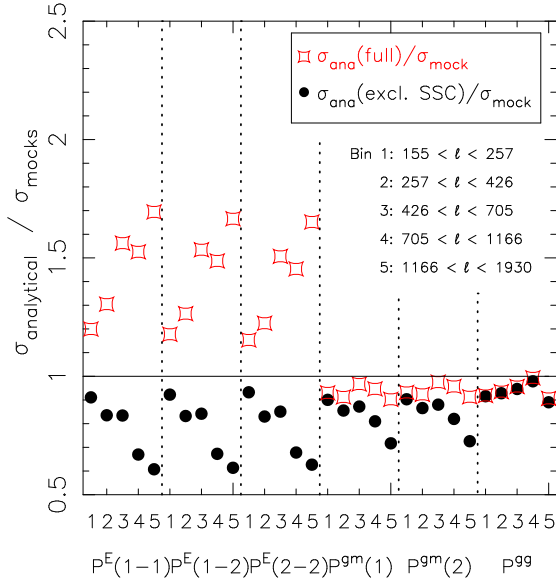
Figure B2. Comparison of the analytical and numerical simulation covariance matrix, for the case without shape noise. The left-hand side shows the ratio of the square root of the diagonals, separately for the six different power spectra. Numbers on the horizontal axis correspond to the different \ell ranges, as indicated in the figure. Red open squares correspond to the full analytical covariance matrix, black circles to the analytical predictions excluding SSC. These two extremes bracket the mock covariance, which has some SSC, but not the full effect. The right-hand side shows the correlation matrix, with the analytical covariance including SSC in the top left and the numerical simulation covariance matrix in the lower right. The off-diagonal terms agree reasonably well.
