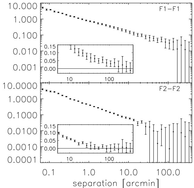
Figure 5. Angular correlation function of the two foreground galaxy samples from GAMA. The inset in each panel shows the signal on large scales with a linear vertical axis. The errors are derived from jackknifing over 2.5 \times 3 degree non-overlapping patches and serve for illustration. When we fit models to our power spectra we used analytical errors throughout.
