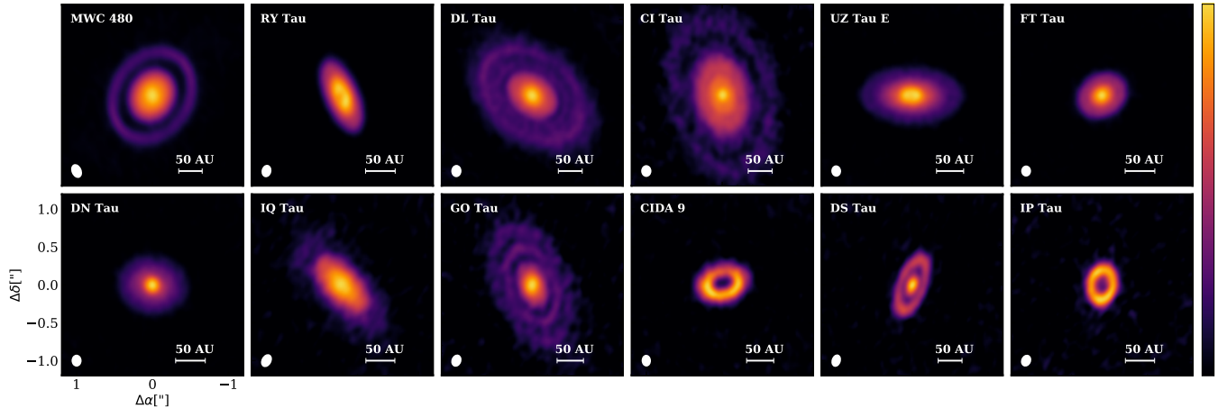
Figure 1. Synthesized images of the 1.33 mm continuum with a Briggs weighting of \text{robust} = 0.5 . The images are displayed in order of decreasing mm flux, from the top left panel to the bottom right panel, and are scaled to highlight the weaker outer emission. The beam for each disk is shown in the left corner of each panel.
