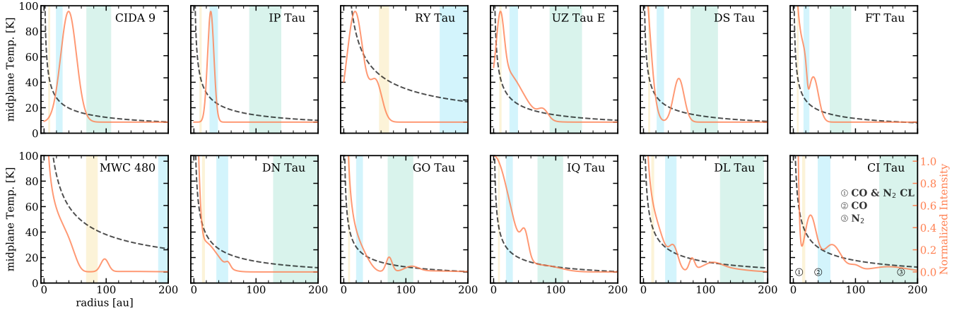
Figure 10. The disk midplane temperature profile (grey dashed line) and normalized intensity profile (orange line) for each disk. The matched ice line locations are marked as shaded regions, with \text{N}_2 in cyan, CO in blue, and the clathrate-hydrate CO and \text{N}_2 in orange.
