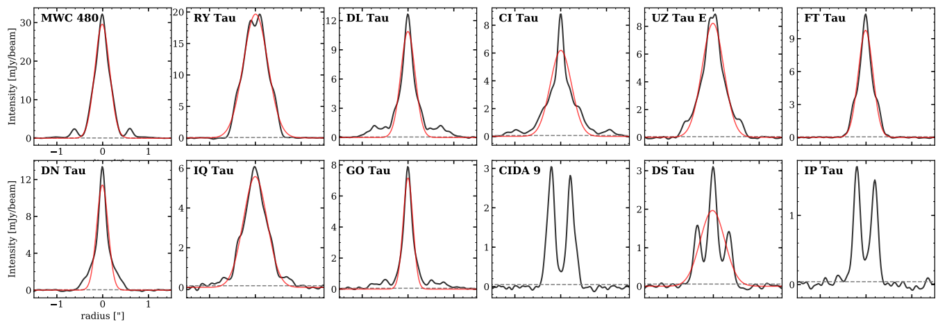
Figure 2. Radial intensity profiles (black lines) along disk major axis for the 12 selected disks with dust substructures, as the same order of Figure 1. The fitted Gaussian profile is shown in red to highlight the disk substructures, except for CIDA 9 and IP Tau, which have deep inner cavities. The 1\sigma noise level is shown in dashed line.
