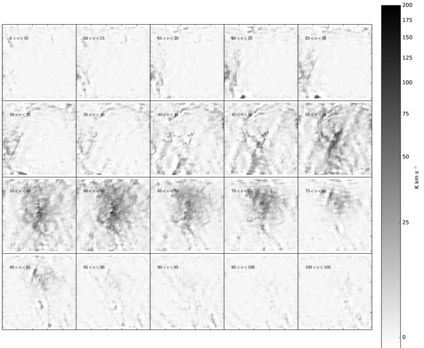
Figure 20. Channel maps of the \text{HC}_3\text{N } J=10-9 line. Each panel shows the integrated intensity over a 5 \text{ km s}^{-1} velocity range as indicated on the figures. The data shown here are 12\text{m}+7\text{m} images made excluding the long-baseline data sets to emphasize large angular scales combined with total power data by feathering the images. The ‘ridge’ feature discussed in the text is most evident in the 50\text{-}55 \text{ km s}^{-1} channel, and these images show that it is dominated by a single velocity component.
