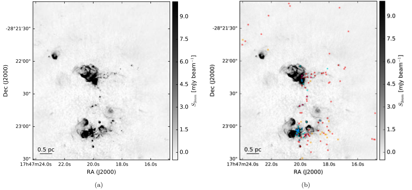
Figure 2. Images of the ALMA 3 mm continuum in the Sgr B2 M and N region. The right figure additionally includes markers at the position of each identified continuum pointlike source: red dots are ‘conservative’, high-confidence sources, orange squares are ‘optimistic’, low-confidence sources, cyan are H II regions, magenta +’s are CH 3 OH masers, blue +’s are H 2 O masers, and green X’s are X-ray sources. The massive protocluster Sgr B2 M is the collection of H II regions and compact sources in the lower half of the image. The other massive protocluster, Sgr B2 N, is in the center. The crowded parts of the images are shown with inset zoom-in panels in Figure 3.
