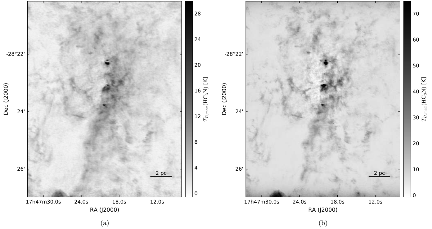
Figure 21. Peak intensity maps of \text{HC}_3\text{N} J=10-9. The left image shows the 12m short-baseline data combined with 7m and total power data; by excluding the long-baseline data, the large angular scales are emphasized. The right image shows the robust 0.5-weighted 12m+7m data combined with total power data; it reaches a substantially higher peak intensity in the compact regions, but the lower-intensity diffuse emission is relatively hidden. In the right image, the negative bowls seen near Sgr B2 M and N in this peak-intensity image indicate that intermediate size scales were not well-recovered. The bright feature on the bottom-left of both images may be an imaging artifact.
