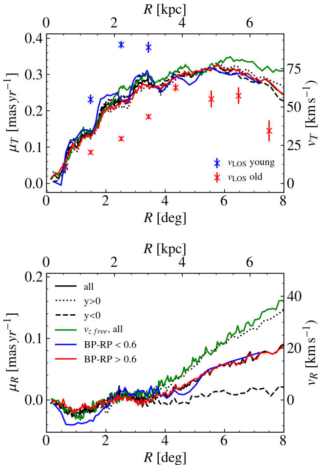
Fig. 18. Rotation curve (top) and median v_R (bottom) of the LMC. The assumed values for the centre-of-mass velocity and orientation of the disc ( i and \Omega ) are taken from a fit to all stars within angular radii \rho < 3^\circ of the LMC centre. Angular distances and velocities given on the lower and left axes have been converted to real-space values on the upper and right axes assuming a distance to the LMC of 50.1 kpc (Freedman et al. 2001). The points shown in the upper panel are derived from observed line-of-sight velocities of old and young stars by van der Marel & Kallivayalil (2014, their Table 4.)
