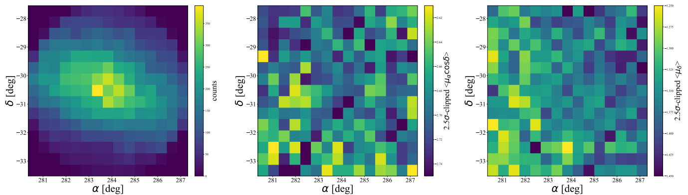
Fig. 13. Counts in 0.2 deg wide bins on the sky with at least 100 stars for stars in the Sagittarius dwarf (left) and the average PM in \mu_{\alpha*} (middle) and \mu_{\delta} (right) for each of these bins.
