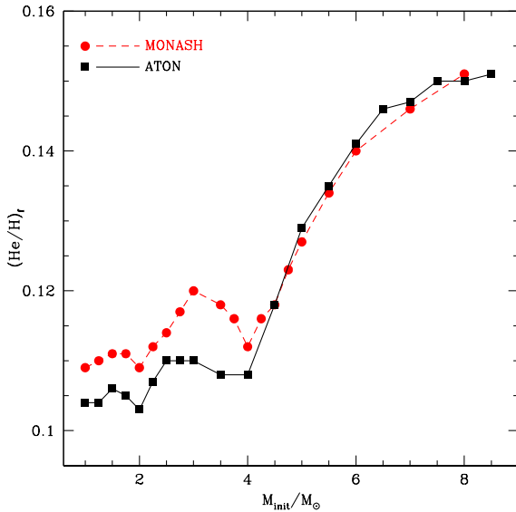
Figure 13. The final \text{He}/\text{H} fraction of AGB models of different mass.
