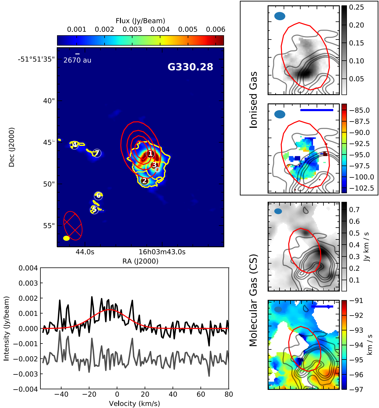
Fig. 2. Continuum, H29 \alpha , and CS emission from G330.28. Top left panel: 256 GHz continuum in colour scale in which the 5 GHz emission is shown in red contours; the red contours in the other images represent this same 5 GHz emission for comparison. The yellow contours show the outlines of the FeIIWalker identified cores. Bottom left panel: H29 \alpha emission (black) with its Gaussian fit. The grey line shows the residuals from the Gaussian fit. In these spectra, the emission has been re-centred to the expected rest velocity of the source, thus the velocity shift of the line peak (from zero) represents a difference between the ionised and molecular gas velocities. Top two panels on the right: moment 0 and moment 1 maps of the H29 \alpha emission ( top and bottom ), while bottom two panels on the right: moment 0 and moment 1 maps of the CS emission ( top and bottom ).
