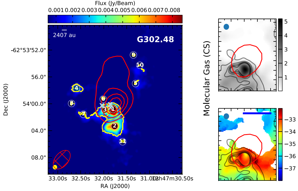
Fig. 7. Continuum and CS emission from G302.48. Left panel: 256 GHz continuum in colour scale with 5 GHz emission in red contours. The yellow contours show the outlines of the FellWalker identified cores. Two right panels: moment 0 and moment 1 ( top and bottom , respectively) maps of the CS emission focussed on the brightest clump, where the HII region is expected to be (although no H29 \alpha was detected, the 5 GHz continuum shows its location).
