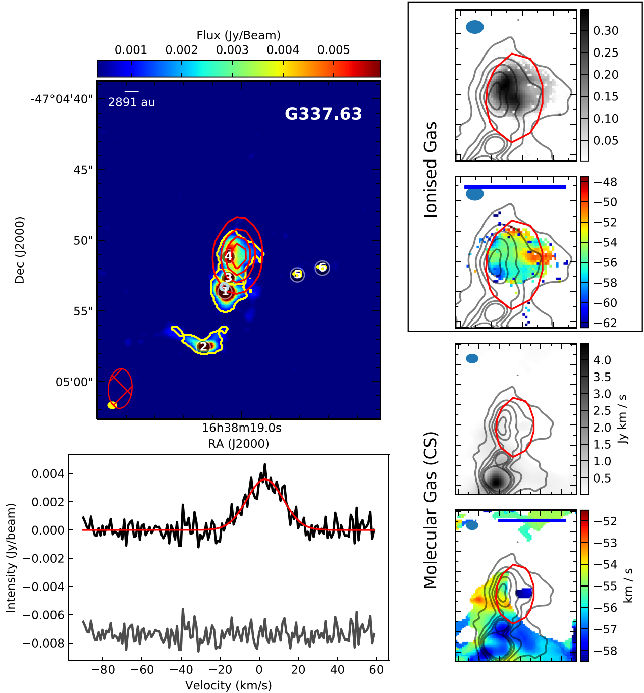
Fig. 4. Continuum, H 29\alpha , and CS emission from G337.63. Top left panel: 256 GHz continuum in colour scale in which the 5 GHz emission is shown in red contours; the red contours in the other images represent this same 5 GHz emission for comparison. The yellow contours show the outlines of the FeIIWalker identified cores. Bottom left panel: H 29\alpha emission (black) with its Gaussian fit. The grey line shows the residuals from the Gaussian fit. In these spectra, the emission has been re-centred to the expected rest velocity of the source, thus the velocity shift of the line peak (from zero) represents a difference between the ionised and molecular gas velocities. Top two panels on the right: moment 0 and moment 1 maps of the H 29\alpha emission ( top and bottom ), while bottom two panels on the right: moment 0 and moment 1 maps of the CS emission ( top and bottom ).
