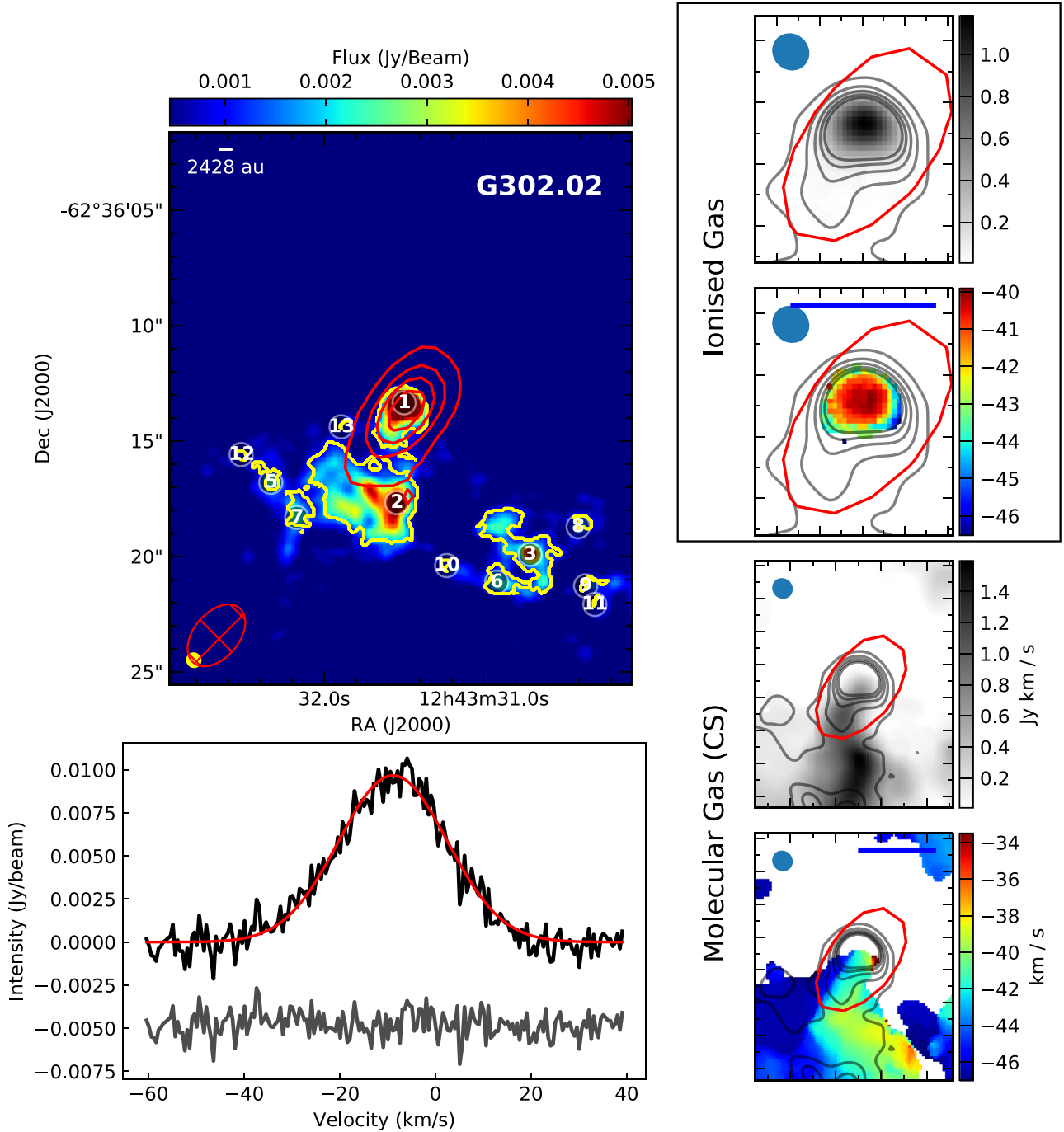
Fig. 1. Continuum, H29 \alpha , and CS emission from G302.02. Top left panel: 256 GHz continuum in colour scale in which the 5 GHz emission is shown in red contours; the red contours in the other images represent this same 5 GHz emission for comparison. The yellow contours show the outlines of the FeIIWalker identified cores. Bottom left panel: H29 \alpha emission (black) with its Gaussian fit. The grey line shows the residuals from the Gaussian fit. In these spectra, the emission has been re-centred to the expected rest velocity of the source, thus the velocity shift of the line peak (from zero) represents a difference between the ionised and molecular gas velocities. Top two panels on the right: moment 0 and moment 1 maps of the H29 \alpha emission ( top and bottom ), while bottom two panels on the right: moment 0 and moment 1 maps of the CS emission ( top and bottom ).
