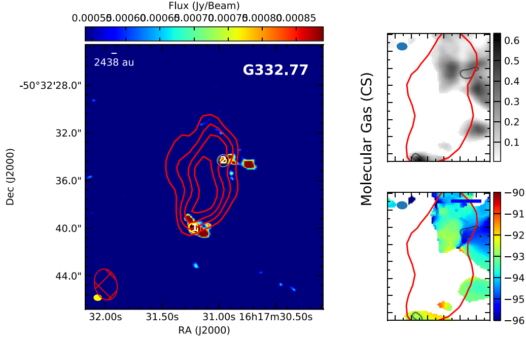
Fig. 9. Continuum and CS emission from G332.77. Left panel: 256 GHz continuum in colour scale with 5 GHz emission in red contours. The yellow contours show the outlines of the FellWalker identified cores. Two right panels: moment 0 and moment 1 ( top and bottom , respectively) maps of the CS emission focussed on the brightest clump, where the HII region is expected to be (although no H29 \alpha was detected, the 5 GHz continuum shows its location).
