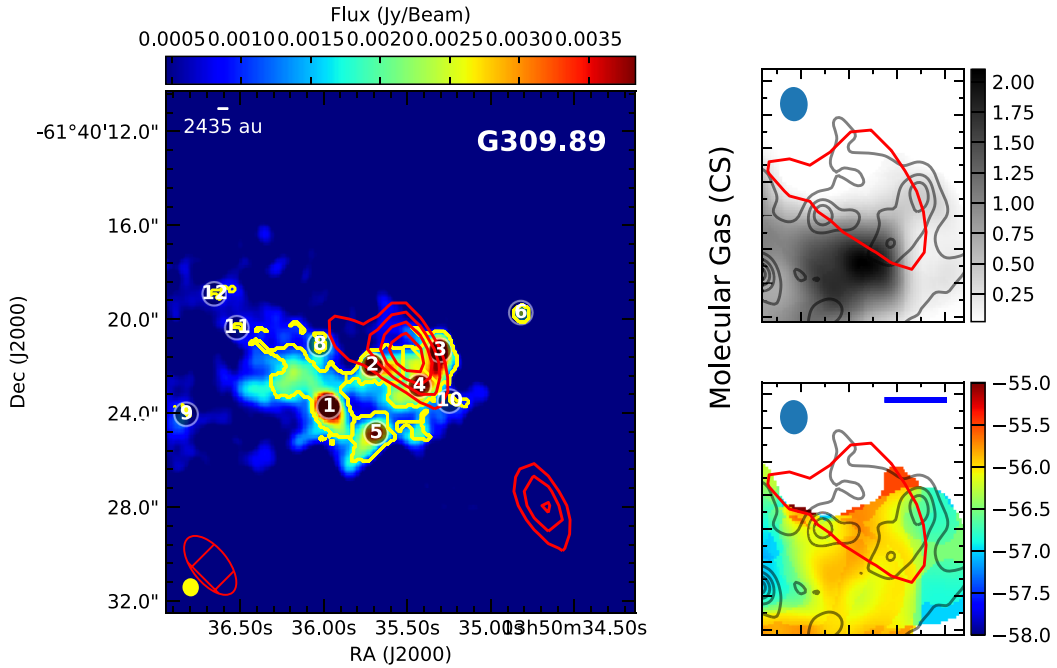
Fig. 8. Continuum and CS emission from G309.89. Left panel: 256 GHz continuum in colour scale with 5 GHz emission in red contours. The yellow contours show the outlines of the FellWalker identified cores. Two right panels: moment 0 and moment 1 ( top and bottom , respectively) maps of the CS emission focussed on the brightest clump, where the HII region is expected to be (although no H29 \alpha was detected, the 5 GHz continuum shows its location).
