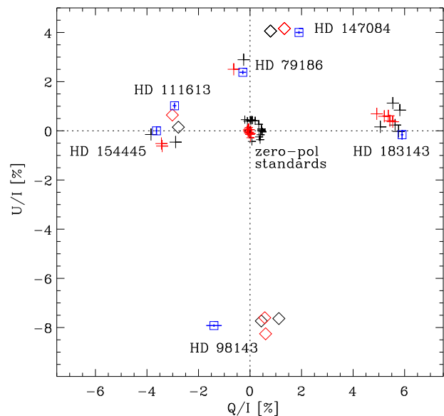
Fig. 25. Polarization of high polarization standard stars for the N_R filter: black symbols give efficiency or c1 corrected values while red symbols are also corrected for the telescope polarization (c2-correction). For individual targets, either plus-signs or diamonds are used in order to avoid confusion. Corresponding literature values are plotted as blue squares with error bars. Also included are the zero-polarization standard stars from the previous subsection.
