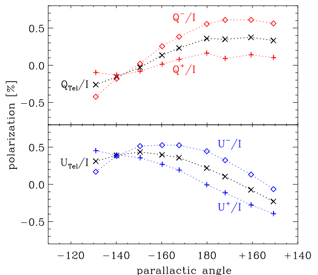
Fig. 23. Residual telescope polarization q_{\text{tel}} = Q_{\text{tel}}/I and u_{\text{tel}} = U_{\text{tel}}/I as function of parallactic angle for the unpolarized star \epsilon Eri in the VBB filter. Also shown are the measurements q^+ , q^- , u^+ , and u^- of a polarimetric cycle, which include instrument polarization component \pm p_{\text{SZ}} for the P2-mode and a field position angle offset of 60^\circ .
