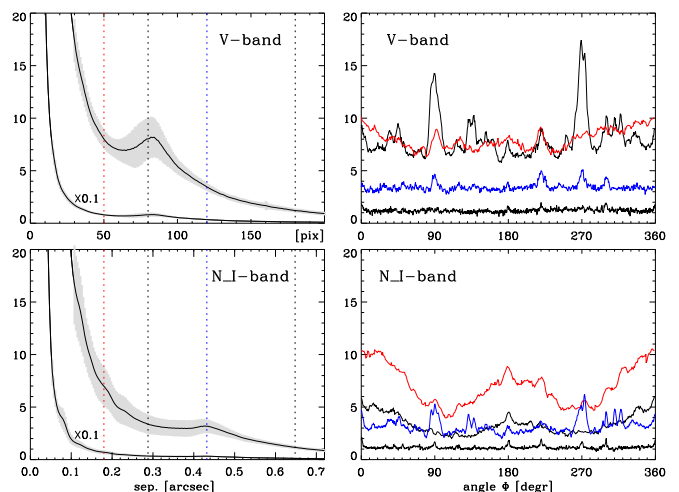
Fig. 9. Azimuthally averaged radial profiles ct_{\text{n6}}(\rho) (left) and azimuthal profiles ct_{\text{n6}}(r, \phi) for r = 50, 80, 120 and 180 pix (right) corresponding to \rho = 0.18'', 0.29'', 0.43'', and 0.65'' , respectively for the PSFs of HD 183143 shown in Fig. 8. Also indicated as gray shading are the standard deviations of the azimuthal points \sigma(ct_{\text{n6}}(r, \phi)) . The location of the azimuthal cuts are indicated in the ct_{\text{n6}}(r) -panels and in Fig. 8.
