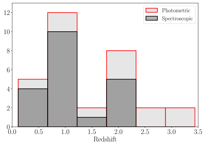
Fig. 4: Redshift distribution for our detected VLBI sources. There are 20 spectroscopic redshifts (dark grey) and 11 photometric redshifts (light grey) for these objects. The over-density of sources at z \sim 2 are briefly discussed in Section 5.1. Optimal bin widths were calculated using the prescription in Knuth (2006).
