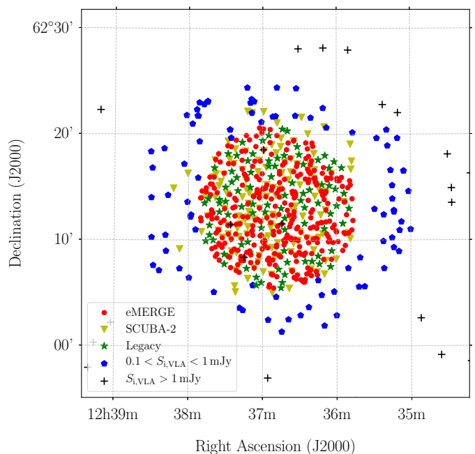
Fig. 1: Sources / sub-fields targeted by these observations. The central 7.5 radius area complements the eMERGE survey and targets eMERLIN detected sources (red circles), SCUBA sub-mm sources (yellow inverted triangles) and ‘legacy’ positions (green stars) which aim to fill in the gaps in coverage. The outer annulus targets only the brightest sources detected by the VLA in Morrison et al. (2010). Those with integrated flux densities 0.1 < S_{i,\text{VLA}} < 1 \text{ mJy} (blue heptagons) are targeted to a radius of 12’ and bright sources S_{i,\text{VLA}} > 1 \text{ mJy} (black crosses) are targeted to the edge of the Morrison et al. (2010) survey.
