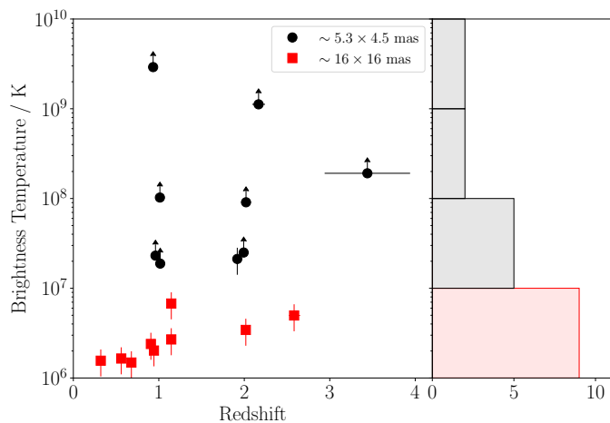
Fig. 7: Brightness temperature distribution with respect to redshift. The black circles and red squares correspond to those sources detected with a \sim 5.3 \times 4.5 mas restoring beam and those detected with a \sim 16 \times 16 mas beam respectively. Arrows correspond to the lower limits for sources classified as unresolved (i.e. either \theta_{\text{maj}} or \theta_{\text{min}} is less than the minimum resolvable size). The histogram shows the distribution of brightness temperatures which is colour coded with the markers. The majority of brightness temperatures are between 10^6 and 10^8 K.
