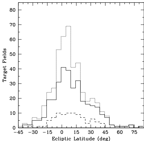
Fig. 6. Distribution of the NEA ecliptic latitudes.
