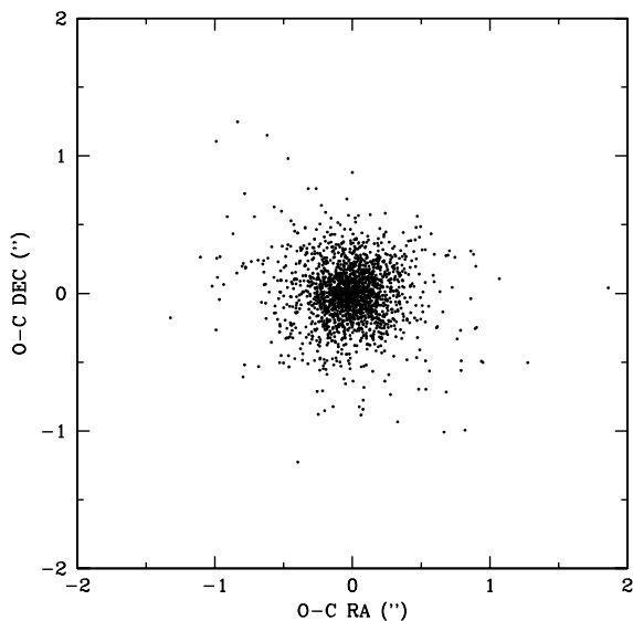
Fig. 7. O-C residuals for 1,854 positions of 280 one-opposition NEAs.
