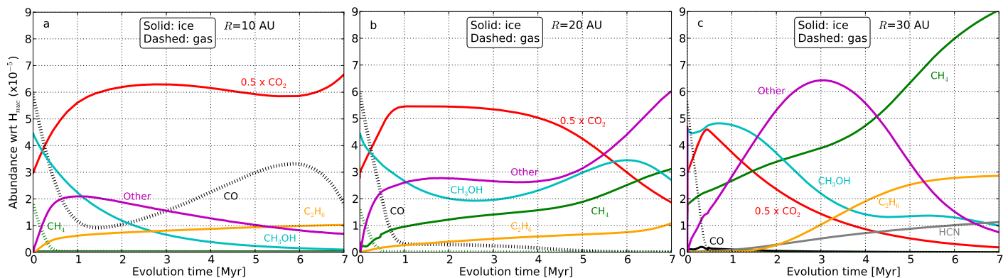
Fig. 8. Time evolution of the main volatile species at 10, 20 and 30 AU, plotted on linear scales to ease comparison to Fig. 7 of Yu et al. (2016) and Fig. 2 of Yu et al. (2017). The \text{H}_2\text{O} ice abundance in these plots is at least 80. Note the rapid decrease of gaseous CO within 1 Myr. Notice that \text{CO}_2 ice is plotted at half its abundance to emphasise the steep drop for CO gas before 1 Myr at all three radii.
