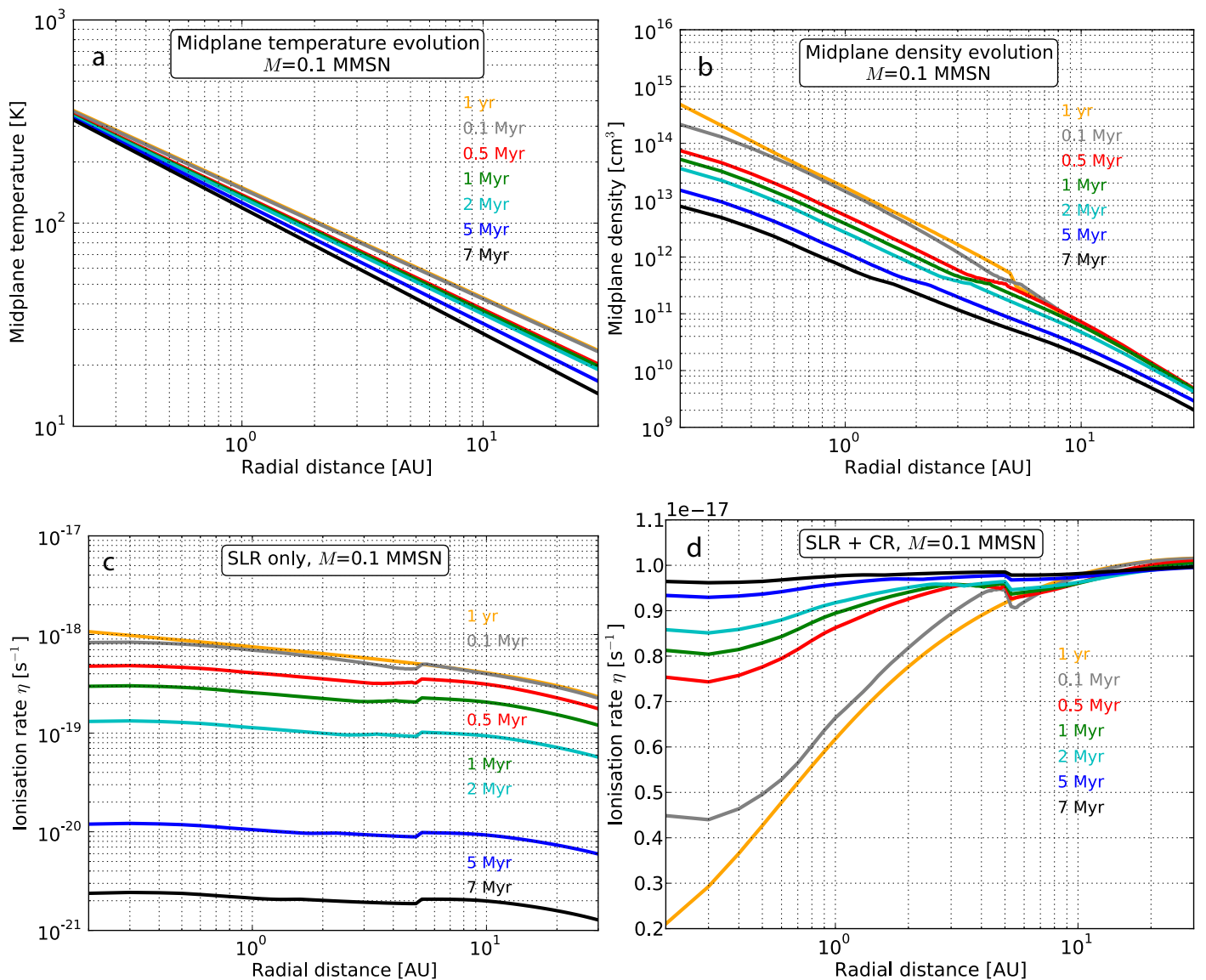
Fig. 1. Midplane temperature and density (top) and ionisation rates (bottom) as functions of disk radius for different evolutionary times for the 0.1 MMSN evolving disk model. For this model, the starting conditions at 1 yr are given by the orange profiles shown here, which feature slightly different physical conditions than that for the static disk structure adopted by Paper 1 (see text for details).
