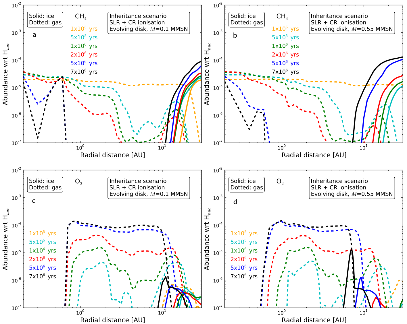
Fig. 6. Same as Fig 5, but for \text{CH}_4 and \text{O}_2 .
