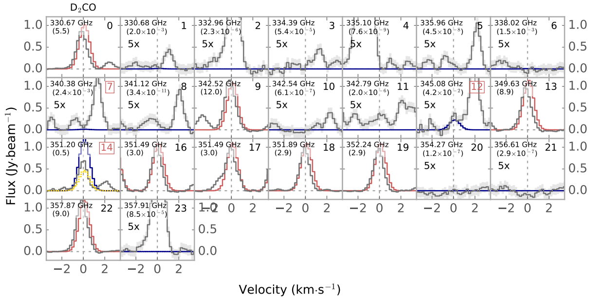
Fig. B.5. All the lines of D 2 CO with the best fit LTE model overplotted. Synthetic spectra in red indicate optical depth beginning to play a significant role i.e. \tau > 0.6 . Numbers in top right corner with red boxes indicate lines used to fit the column density. The emission line at 332.96 GHz is possibly glycolaldehyde and ethylene glycol, and at 357.91 GHz methyl formate.
