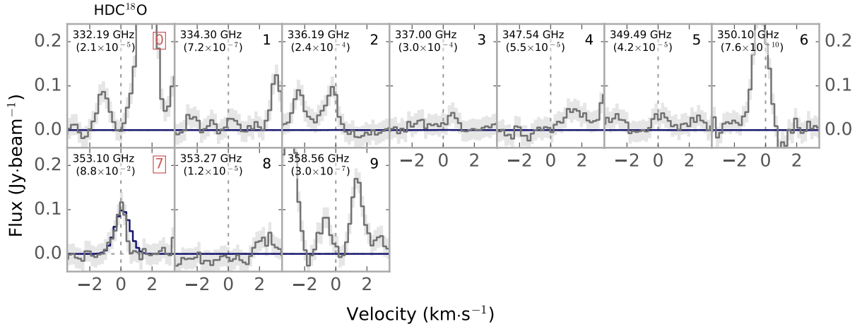
Fig. B.4. All the lines of HDC 18 O with the best fit LTE model overplotted. Synthetic spectra in red indicate optical depth beginning to play a significant role i.e. \tau > 0.6 . Numbers in top right corner with red boxes indicate lines used to fit the column density. The number in parenthesis is the estimated optical depth. The emission line at 350.10 GHz is probably methanol.
