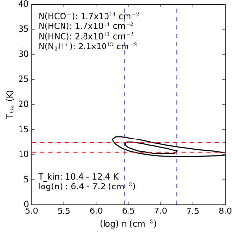
Figure 6. Chi-square minimization of observed and RADEX model intensities using four main molecular lines (HCO, HCN, HNC and \text{N}_2\text{H}^+ ) molecules for clump AGAL333.103-0.502S. Peak contour level shows the constraints in density and kinetic temperature.
