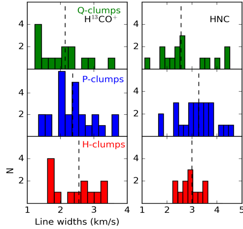
Figure 4. Line widths, of Q, P and HII clumps, determined from Gaussian fit to the peak spectra of optically thin lines \text{H}^{13}\text{CO}^+(3-2) and \text{HNC}(3-2) . The mean value for each distribution is indicated by dotted black line.
