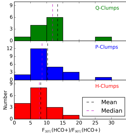
Figure 2. \text{HCO}^+(3-2) integrated intensity ratios within contour region of 30% and 90% of the peak towards different type of clumps. The mean and median for each distribution is indicated by dotted color lines.
