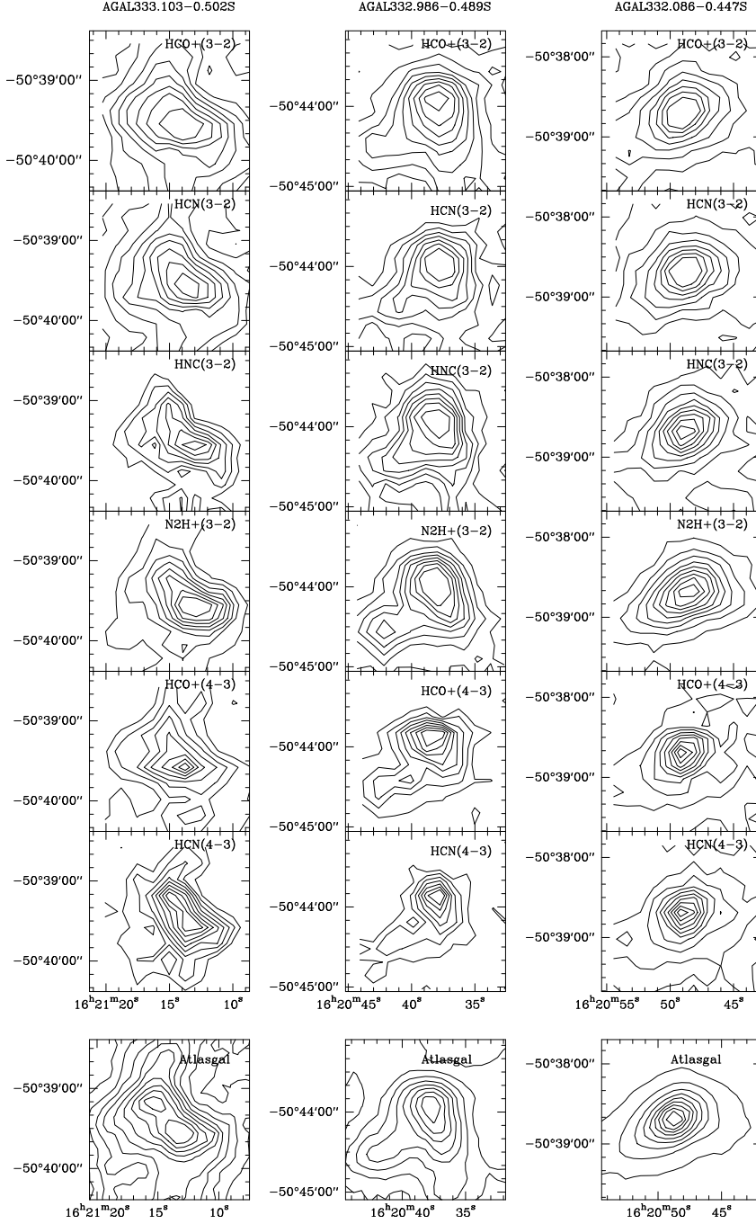
Figure 1. Contour maps of the emissions of 6 different molecular lines and Atlasgal (870μm) continuum map from three types of clumps (AGAL333.103-0.502S: pre-stellar (left), AGAL332.986-0.489S: proto-stellar (middle), and AGAL332.086-0.447S: HII clump (right)). Contour levels have steps of 10% and the peak contour is at 90% level of the peak emission. The molecular species and transition lines are shown inside each box.
