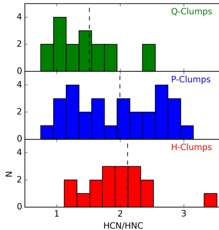
Figure 5. HCN(3-2) to HNC(3-2) integrated intensity ratios from the peak spectra towards Q, P and HII clumps. The average for each distribution is indicated by dotted black line.
