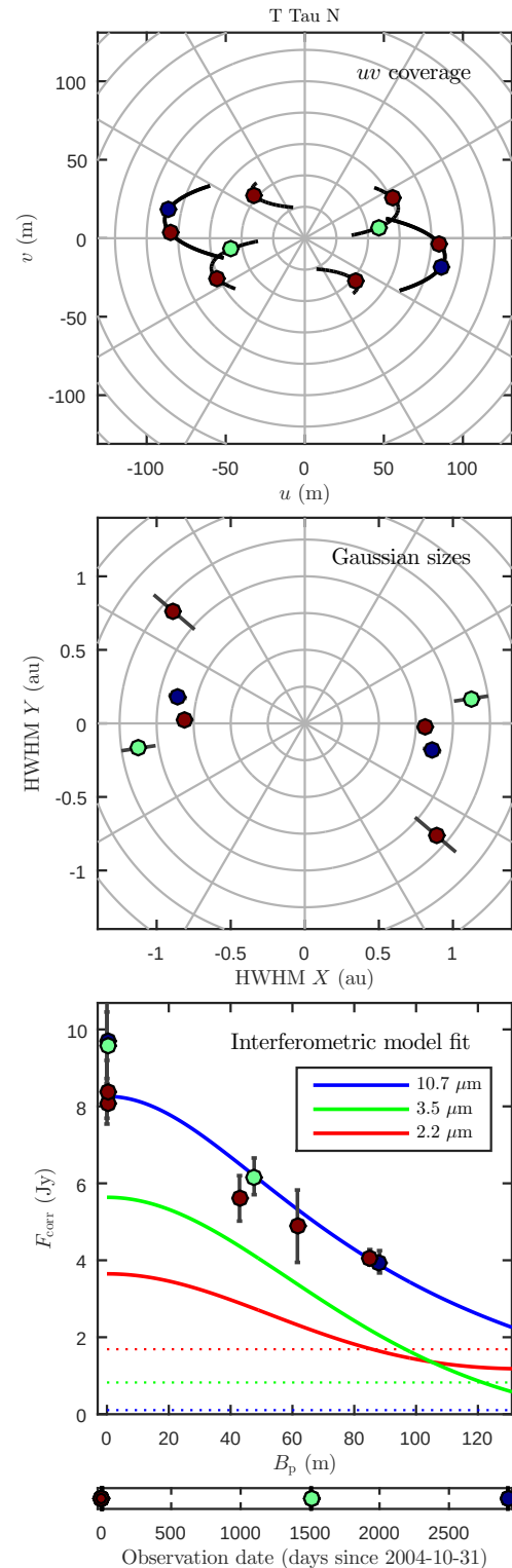
Fig. 2. Figure outputs of the atlas for T Tau N as an example. Top: uv -coverage plot. Middle: Gaussian size diagram. The plot shows the physical sizes of the disk (HWHM, in au, see Eq. 2) individually measured for each observation corresponding to different baseline angles. Bottom: Results of the interferometric modeling to the correlated and total fluxes (shown at 0 m baseline) at 10.7 \mu\text{m} as a function of baseline length. The blue solid line shows continuous model fit. Red and green lines show the correlated fluxes extrapolated from the continuous model to the K and L bands, respectively (see Sections 3.3 and 4.5 for more details). Dotted lines show the estimates for the unresolved stellar emission. Data points on each subplot are color-coded for observing date. For the other sources in the sample see Fig. B.1 in Appendix B.
