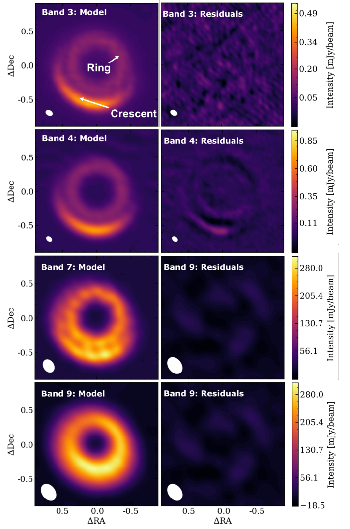
Fig. 6: Models derived from the MCMC using the parameters in Tab. 1, and relative residuals for the four data sets available for HD 135344B. The color scale is the same for the models and the residuals. The white ellipses show the synthesized beam sizes.
