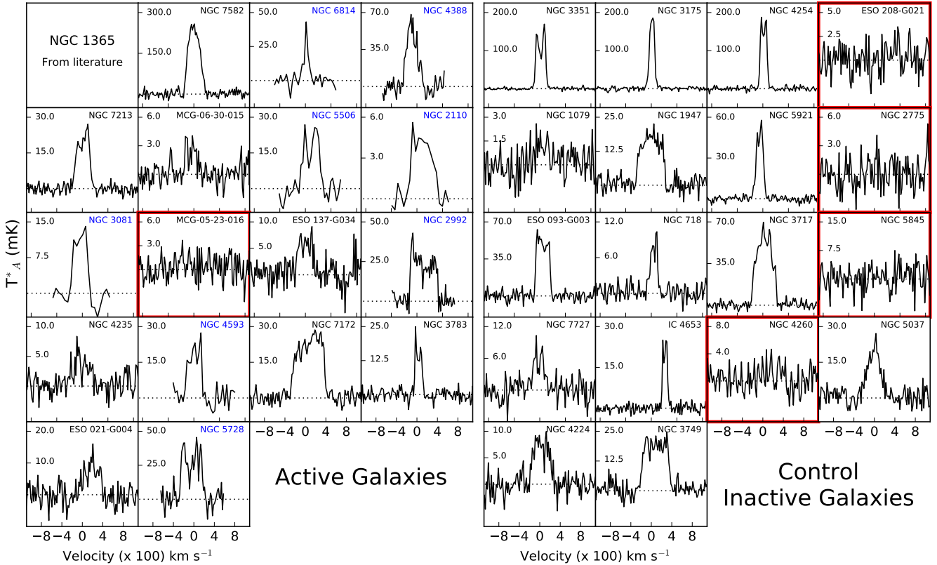
Figure 2. CO 2→1 line spectra of the galaxies from the LLAMA survey featured in this study. Each panel spans a fixed range of 2200 km s -1 of velocity around the systemic velocity of the galaxy to allow a simple visual comparison of the kinematics of the lines. Fluxes are expressed as atmosphere-corrected antenna temperatures ( T_A^* ). AGN hosts are shown on the left and control galaxies on the right, following the same order as Figure 1. Black and blue labels for the names respectively indicate the galaxies for which APEX and JCMT observations were taken. We relied on literature measurements of CO 2→1 for NGC 1365 and do not plot a spectrum here. Panels with red boundaries mark the targets which are not detected in CO at SNR < 3.
