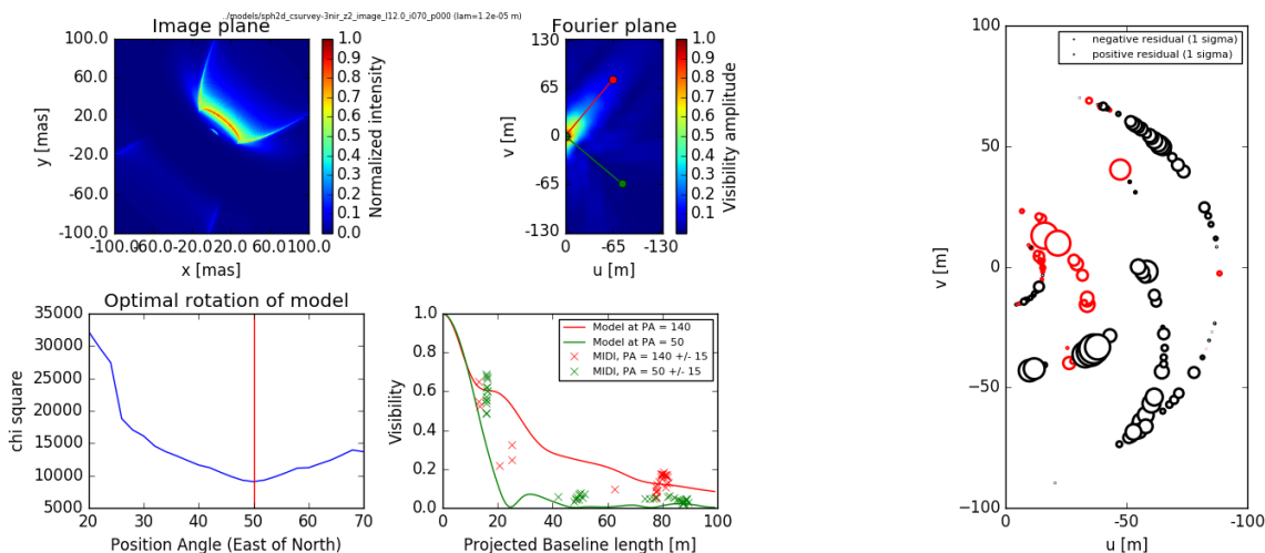
Fig. 20. Radiative transfer model for Circinus. Upper left panel: image at 12 \mu\text{m} ; upper middle panel: visibility amplitudes; lower left panel: \chi^2 as a function of position angle; lower middle panel: visibility amplitudes as a function of projected baseline length (solid lines: model, crosses: observations); right panel: difference between the model and observed visibility amplitudes (red: (model-observations) > 0 , black: (model-observations) < 0 ). The size of the rings is proportional to the value of the residual.
