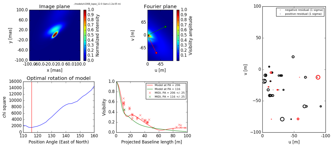
Fig. D.4. NGC 1068. Same as Fig. D.1 for the Lopez-Gonzaga et al. (2014) NGC 1068 model. All three components are included. The third, extended component is barely visible in the left panel, but contributes to the visibilities at short baselines.
