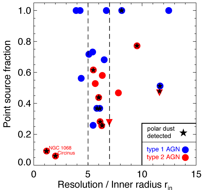
Fig. 17. Point source fraction for the MIR interferometric observations of Burtscher et al. (2013). Only objects around 6r_{\text{in}} should be compared to Fig. 18. Objects with detected extended dust emission are marked with a star. This emission is mostly in polar direction, i.e. the direction of the narrow line region, and was detected on 10 pc-scale (Lopez-Gonzaga et al. 2016 and references therein) and on 100 pc-scale (Asmus et al. 2016), but not for the same objects. Note that the detectability of polar dust emission depends on a number of observational parameters and non-detections do not mean that these AGNs are intrinsically different.
