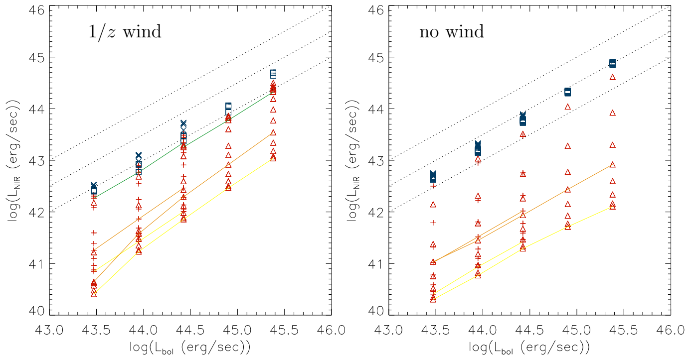
Fig. 10. Model NIR luminosities as a function of the bolometric luminosity. Blue: type 1, red: type 2. Circinus model: crosses/pluses; NGC 1068 model: squares/triangles. The inclination angles of type 2 objects are indicated: i = 50^\circ (green line), i = 70^\circ (orange line), i = 90^\circ (yellow line). Left panel: wind with 1/z density profile. Right panel: no wind component. The dotted lines correspond to L_{\text{NIR}} = \xi L_{\text{bol}} with \xi = 1, 1/3, 1/10 .
