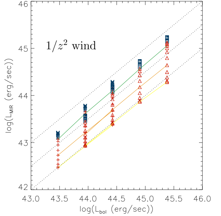
Fig. B.1. Model MIR luminosities as a function of the bolometric luminosity. Blue: type 1, red: type 2. Circinus model: crosses/pluses; NGC 1068 model: squares/triangles. The inclination angles of type 2 objects are indicated: i = 50^\circ (green line), i = 70^\circ (orange line), i = 90^\circ (yellow line).
