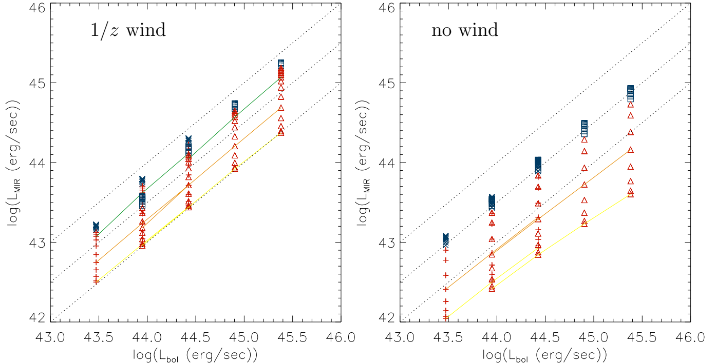
Fig. 9. Model MIR luminosities as a function of the bolometric luminosity. Blue: type 1, red: type 2. Circinus model: crosses/pluses; NGC 1068 model: squares/triangles. The inclination angles of type 2 objects are indicated: i = 50^\circ (green line), i = 70^\circ (orange line), i = 90^\circ (yellow line). Left panel: wind with 1/z density profile. Right panel: no wind component. The dotted lines correspond to L_{\text{MIR}} = \xi L_{\text{bol}} with \xi = 1, 1/3, 1/10 .
