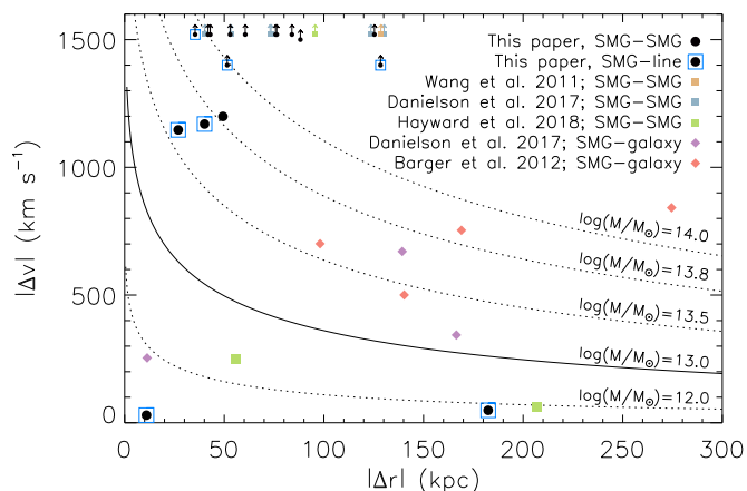
Figure 3. Radial and velocity separations between the multiple 870\text{-}\mu\text{m} selected SMGs (SMG–SMG) as well as serendipitously-detected line emitters (SMG–CO) in each ALMA field. The abscissa is truncated such that galaxy pairs with velocity separations (or lower limits) > 1500\text{ km s}^{-1} are shown as limits at 1500\text{ km s}^{-1} . The curves show the expected profiles for NFW halos of different masses (see Section 4.1 for details). Clustering measurements suggest that 870\text{-}\mu\text{m} selected SMGs reside in halos of mass \sim 10^{13}\text{ M}_{\odot} at z \gtrsim 2 , and simulations suggest that at z \sim 2.5 virialised halos with mass \gtrsim 10^{14}\text{ M}_{\odot} are rare. Therefore, the lower limits on the velocity offsets between blended SMG–SMGs pairs suggest that they are unlikely to reside in the same bound environments. For comparison we also show SMG pairs and SMG–galaxy pairs from blank-field surveys that have interferometric positions and spectroscopic redshifts. The majority of the associated SMG–CO sources, SMG–SMG and SMG–galaxy pairs have velocity offsets higher than expected if they occupy the same virialised \sim 10^{13}\text{ M}_{\odot} halo, and may instead indicate that they trace different proto-cluster substructure. Measurement uncertainties are not shown because they are typically smaller than the data points.
