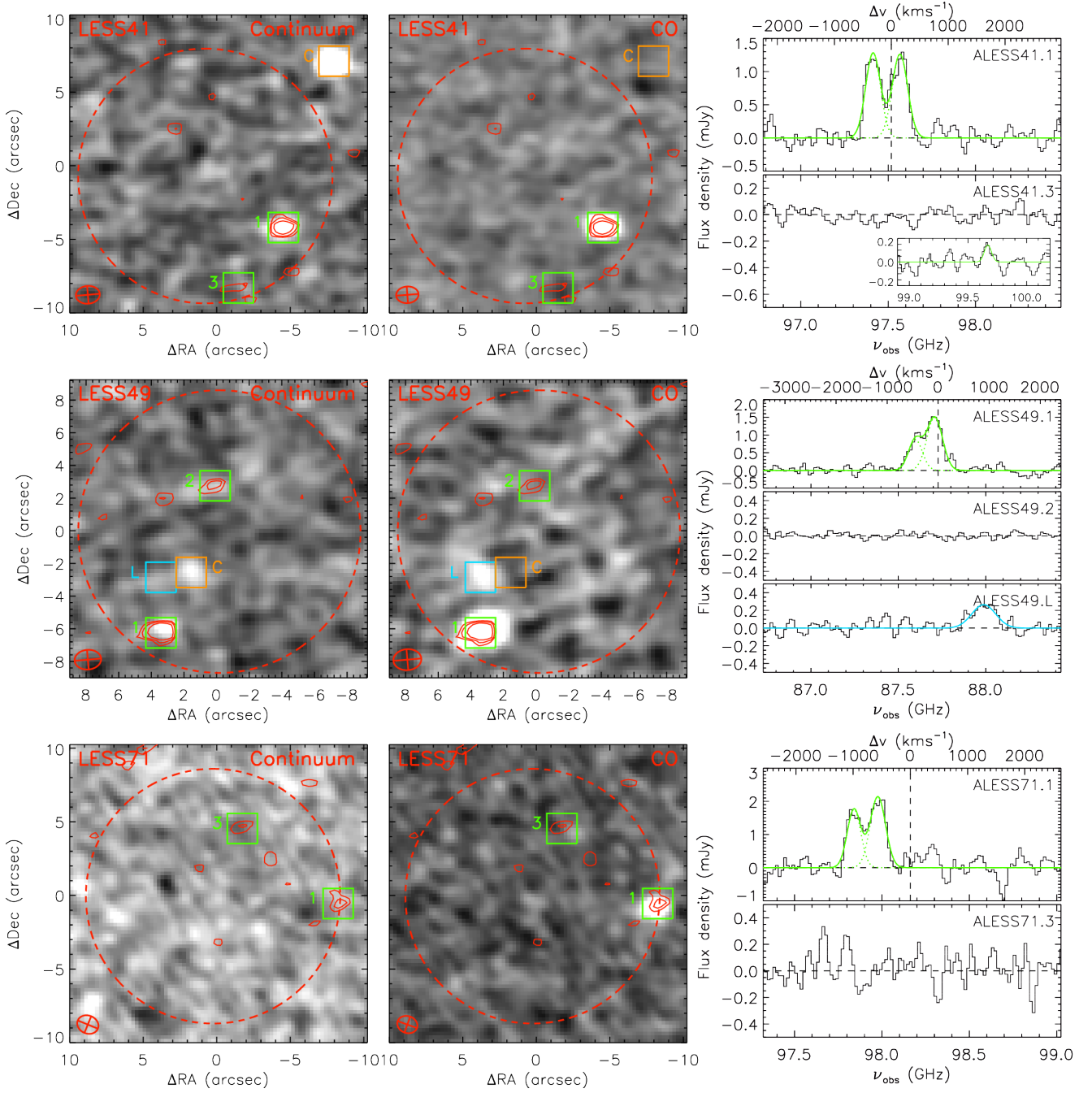
Figure 1. An overview of the ALMA data in each field, demonstrating the quality of the data, the strength of the detections and the correspondence between the 870\text{-}\mu\text{m} selected SMGs and sources in our 3.3-mm data. Left column: The naturally-weighted 870\text{-}\mu\text{m} continuum data (greyscale), with 870\text{-}\mu\text{m} continuum contours (at 2.5, 3.5, 5, 10, 20\sigma ) overlaid from Hodge et al. (2013) or Simpson et al. (2015b) . The dashed circle shows the 870\text{-}\mu\text{m} primary beam and the ellipse in the lower-left corner represents the 3.3 mm restored beam. At \sim 55'' the 3.3 mm primary beam is larger than the areas shown, but there are no significant sources outside of the areas shown. 870\text{-}\mu\text{m} selected SMGs are highlighted and labelled with green boxes, 3.3-mm selected continuum sources (Section 3.4) are marked in orange, and serendipitously-identified emission line sources (Section 3.2) are in cyan. Labels are the sub-IDs of the sources (Table 1), so source ‘1’ in the LESS 41 panels is ALESS 41.1 etc. Centre column: Collapsed, continuum-subtracted, naturally-weighted images covering the frequencies of the emission lines (i.e. moment-0 maps of the line emission). Annotations and labels are the same as in the left-hand panel. Right column: Continuum-subtracted spectrum for each SMG and serendipitously-detected emission line source; labels in the top-right of each panel show the name of the source. Dashed vertical lines mark the expected frequency of CO emission based on spectroscopic optical/near-infrared redshifts, where they exist (Table 1), and the top axis shows the velocity offset from this frequency. Best-fit single or double Gaussian profile are overlaid for sources with detected emission lines (Section 3.1 and 3.2). ALESS 41.3 includes an inset showing the possible weak line in the other sideband at \sim 99.7 GHz (Section 3.1).
