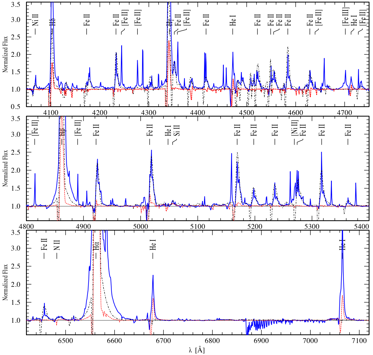
Fig. F.1. 2016 \eta Car’s FEROS spectrum (blue-solid line). The image displays our best-fit CMFGEN model (red-dashed line) and the model described in Groh et al. (2012a; black-dashed line). The Balmer lines of the FEROS spectrum are too strong. They include large contributions of the circumstellar emission as a result of the bad seeing of \sim 2'' at the time of the observation. The black synthetic spectrum matches the Fe II and Si II lines. The absorption component of the P-Cygni profiles are filled in and the He I emission lines are not reproduced by the model, which has been already observed and discussed in detail by Hillier et al. (2001). The hotter red model can hardly fit the spectral lines observed at FEROS’ wavelengths.
