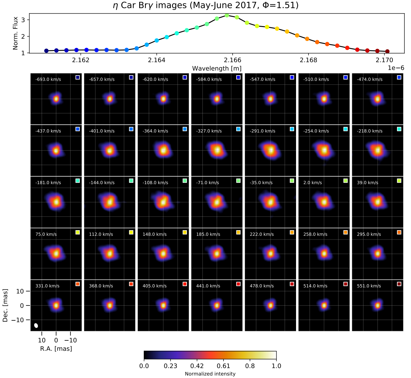
Fig. D.1. Br \gamma interferometric aperture synthesis images from the May-June 2017 data. The Doppler velocity of each frame is labeled in the images. For all the panels, east is to the left and north to the top and the displayed FOV corresponds to 36 \times 36 mas. The small white ellipse shown in the lowermost-left panel corresponds to the synthesized beam (the detailed PSF is shown in Fig. D.1). Above all the images, the GRAVITY spectrum is shown and the different positions where the images are reconstructed across the line are labeled with a colored square, which is also plotted in the images for an easy identification. Due to the sparseness of the u-v coverage, the quality of these reconstructed images is limited, creating a clumpy fine structure and a cross-like shape superimposed on the source's brightness distribution. Therefore, they cannot be properly compared with the GRAVITY 2016 data presented in this work.
