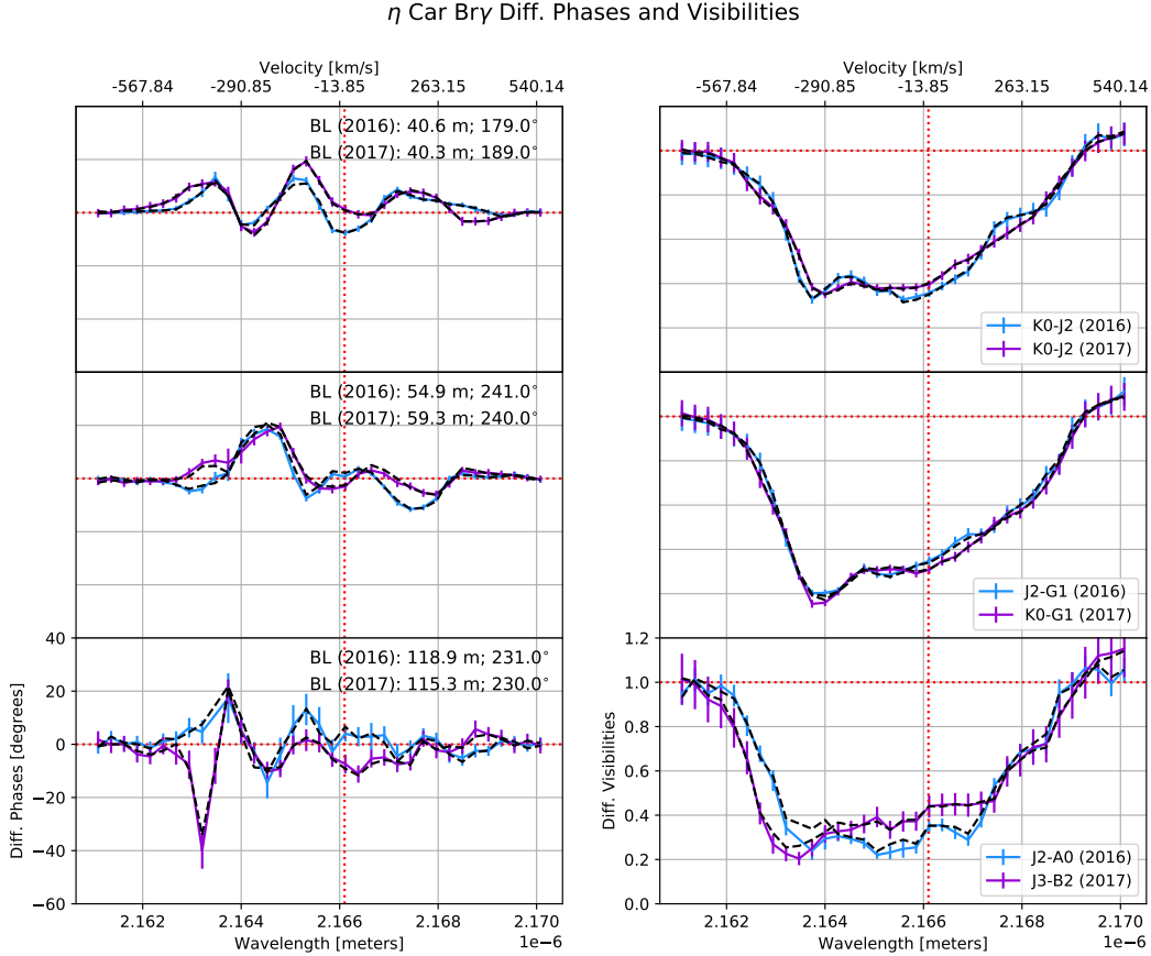
Fig. 8. Differential phases ( left panels ) and differential visibilities ( right panels ) between the continuum and the line emission for the 2016 (blue line) and 2017 data (purple line). The (reference) continuum phase and visibility were estimated using the first and last five channels in the imaged bandpass. Each one of the rows corresponds to a similar baseline in both epochs, tracing large ( top ), intermediate ( middle ) and small ( bottom ) spatial scales. The baseline lengths and position angles are labeled on the left panels , while the baseline stations are labeled on the right ones. The black-dashed lines correspond to the differential quantities extracted from the unconvolved reconstructed images. The vertical red-dotted line marks the systemic velocity of Bry. The horizontal red-dotted lines show the continuum baselines.
