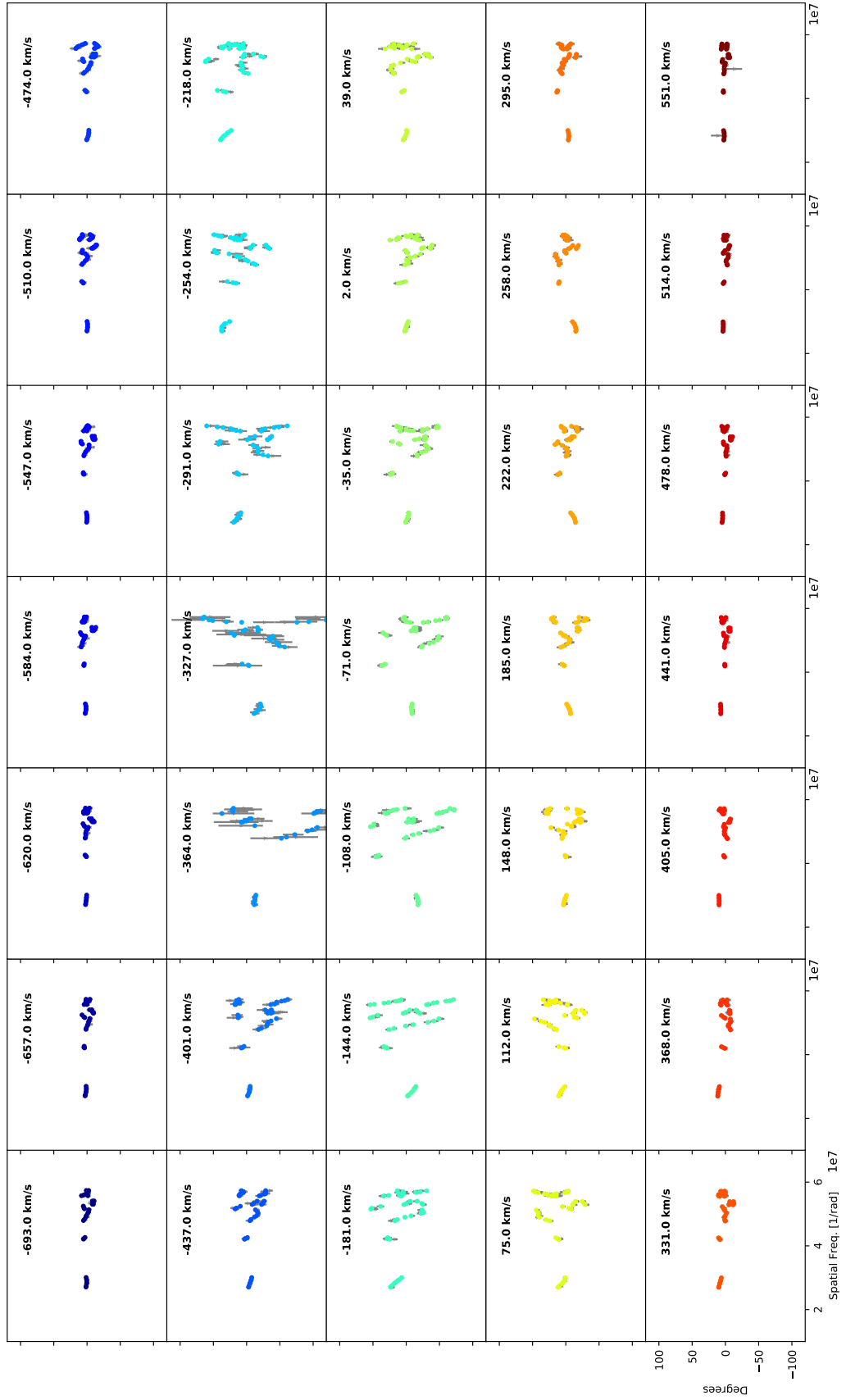
Fig. E.4. Fit to the observed closure phases from the interferometric aperture synthesis images across the Bry line (2017). The panels are as described in Fig. E.1.
