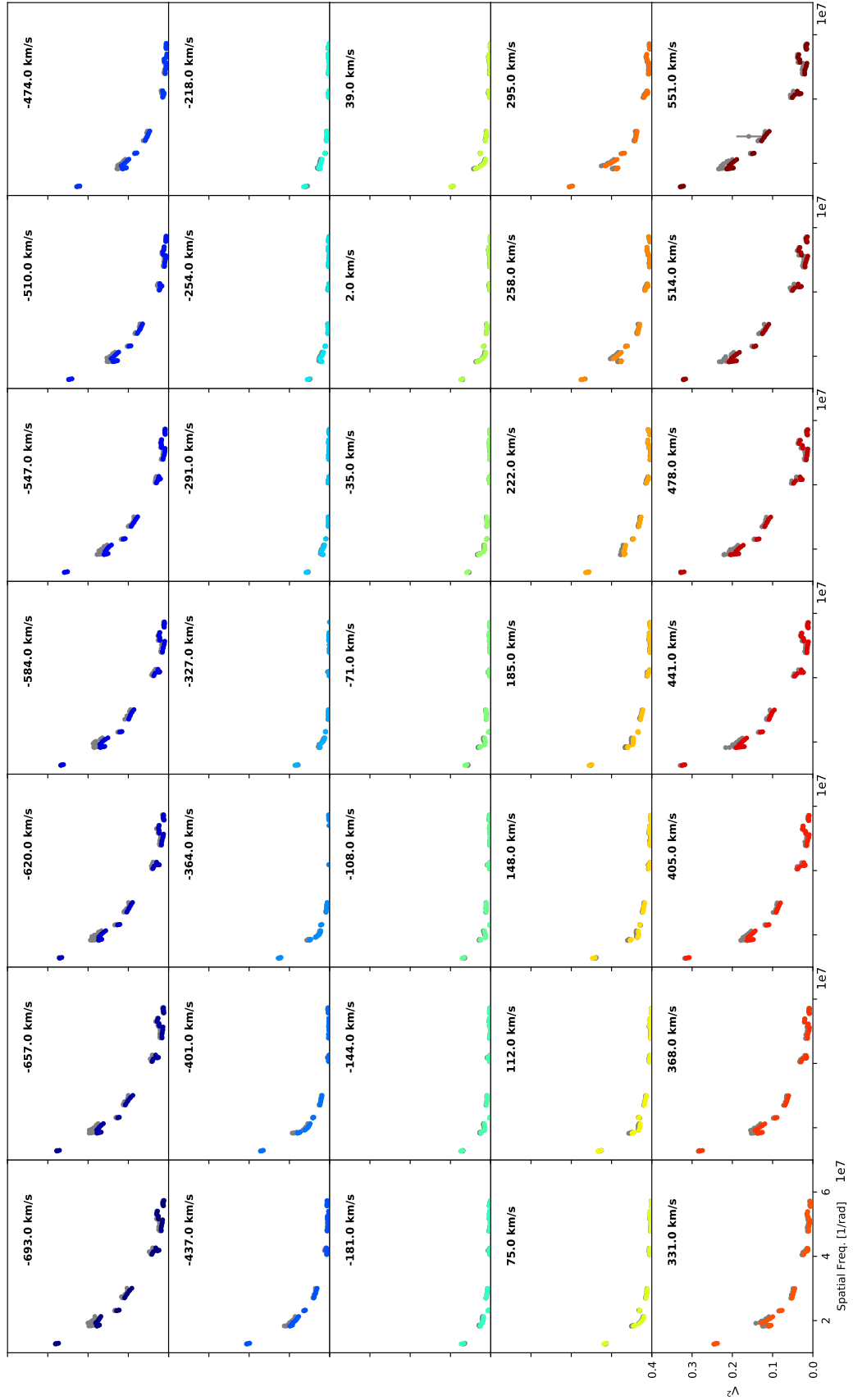
Fig. E.3. Fit to the observed V^2 from the interferometric aperture synthesis images across the Bry line (2017). The panels are as described in Fig. E.1.
