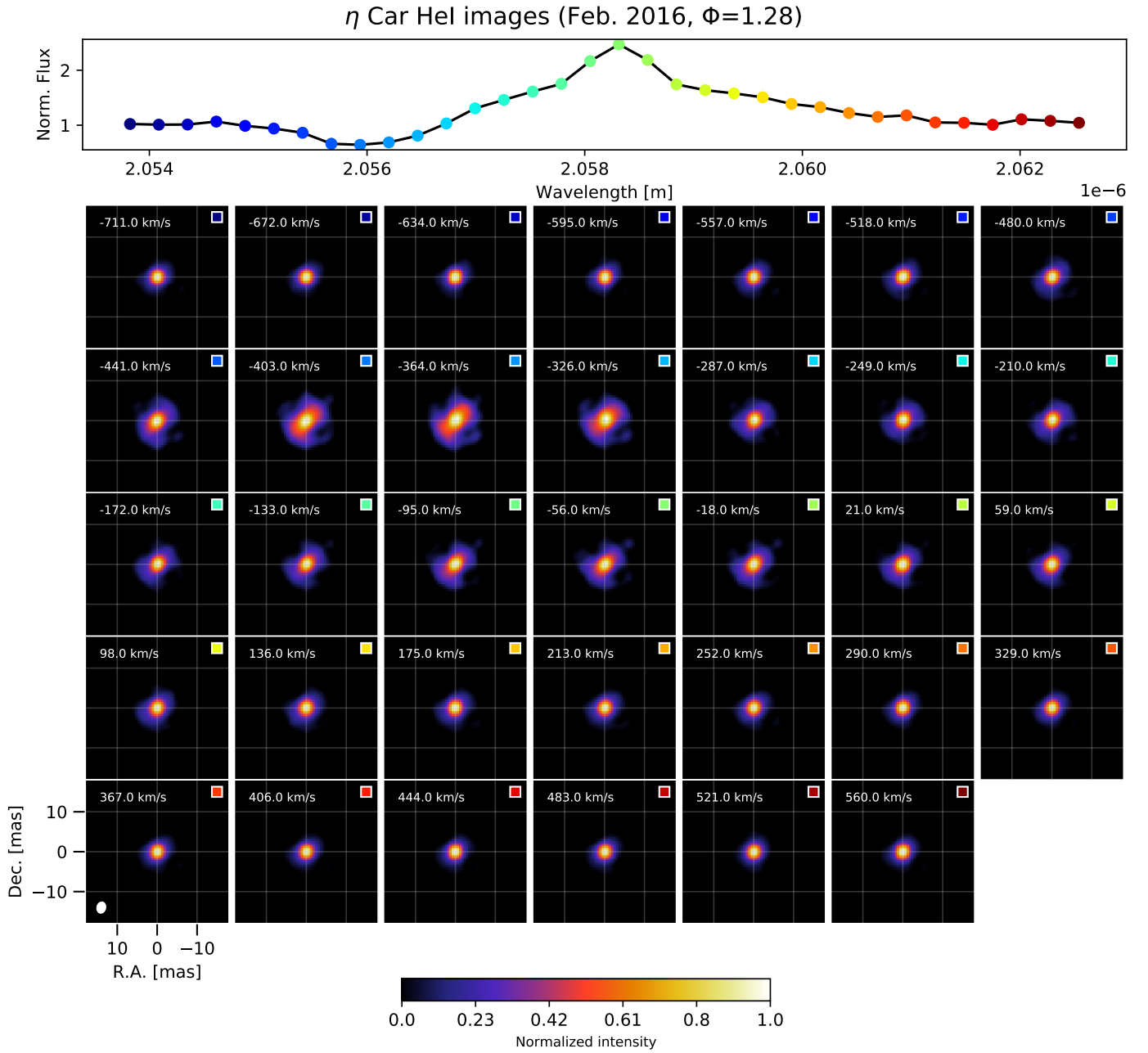
Fig. 7. He I interferometric aperture synthesis images from the Feb. 2016 data. The maps are as described in Fig. 6.
