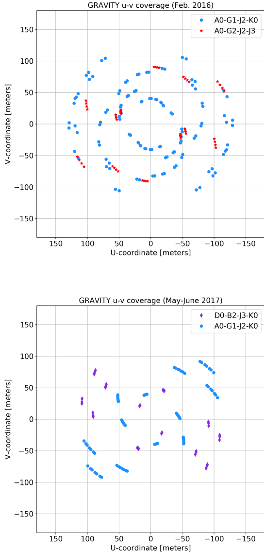
Fig. 2. \eta Car’s u – v coverages obtained during the GRAVITY runs in February 2016 ( top panel ) and May–June 2017 ( bottom panel ). Different quadruplets are indicated with different colors.
