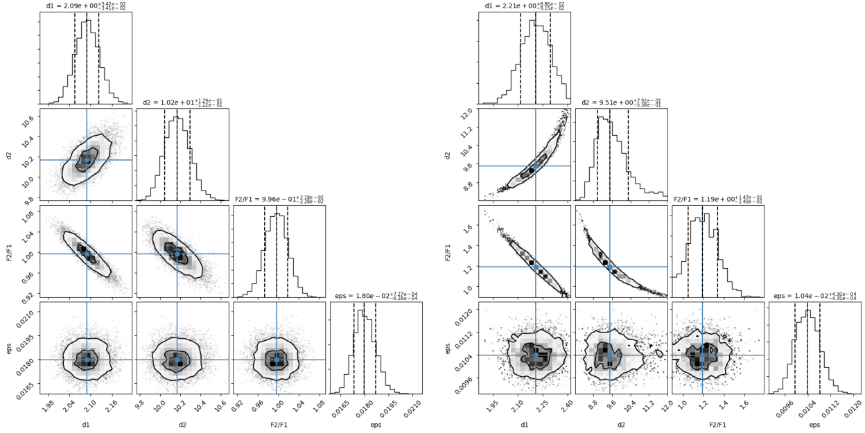
Fig. B.1. Posterior distributions of the best-fit parameters of the geometrical model presented in Sect. 3.1. Left panel: posterior distributions for the model applied to the V^2 data at PA_{\perp} = 40^{\circ} \pm 20^{\circ} , while the right panel displays the posterior distributions for the model at PA_{\parallel} = 130^{\circ} \pm 20^{\circ} . The 2D distributions show 1 and 2 standard deviations encircled with a black contour. The mean of each distribution is displayed with a blue square. The 1D histograms show the expected value (mean) and \pm 1\sigma with vertical dashed lines, together with their corresponding values at the top.
