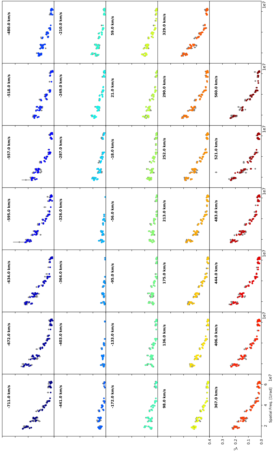
Fig. E.5. Fit to the observed V^2 from the interferometric aperture synthesis images across the He I line (2016). The panels are as described in Fig. E.1.
