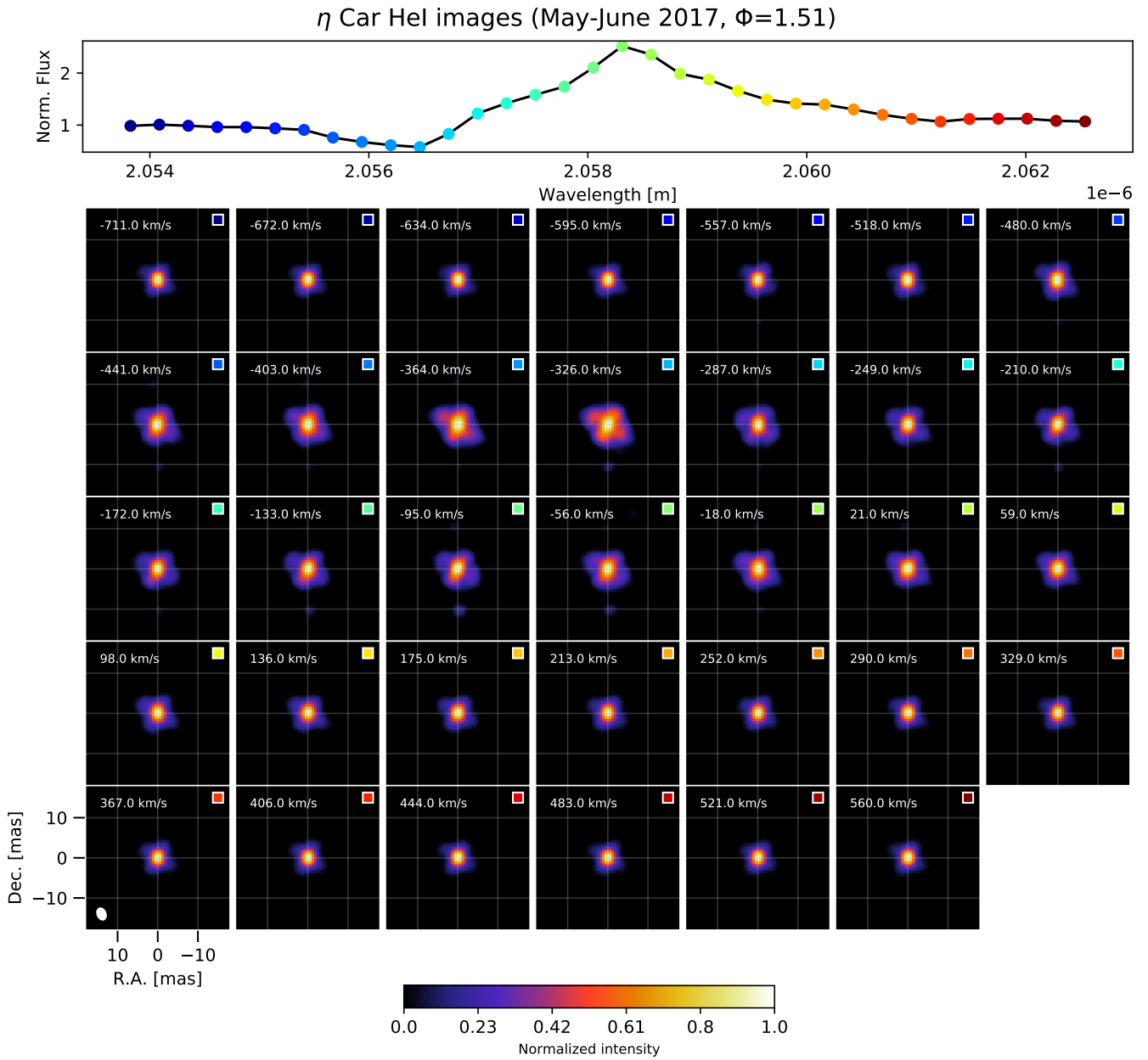
Fig. D.2. He I interferometric aperture synthesis images from the May–June 2017 data. The maps are as described in Fig. D.1.
