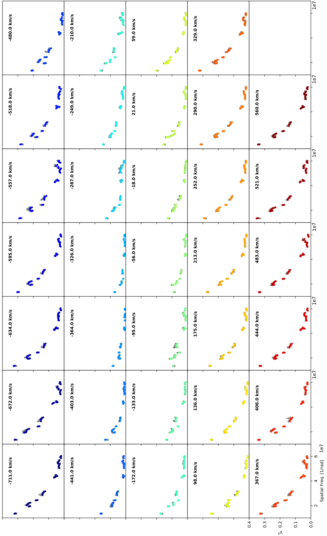
Fig. E.7. Fit to the observed V^2 from the interferometric aperture synthesis images across the He I line (2017). The panels are as described in Fig. E.1.
