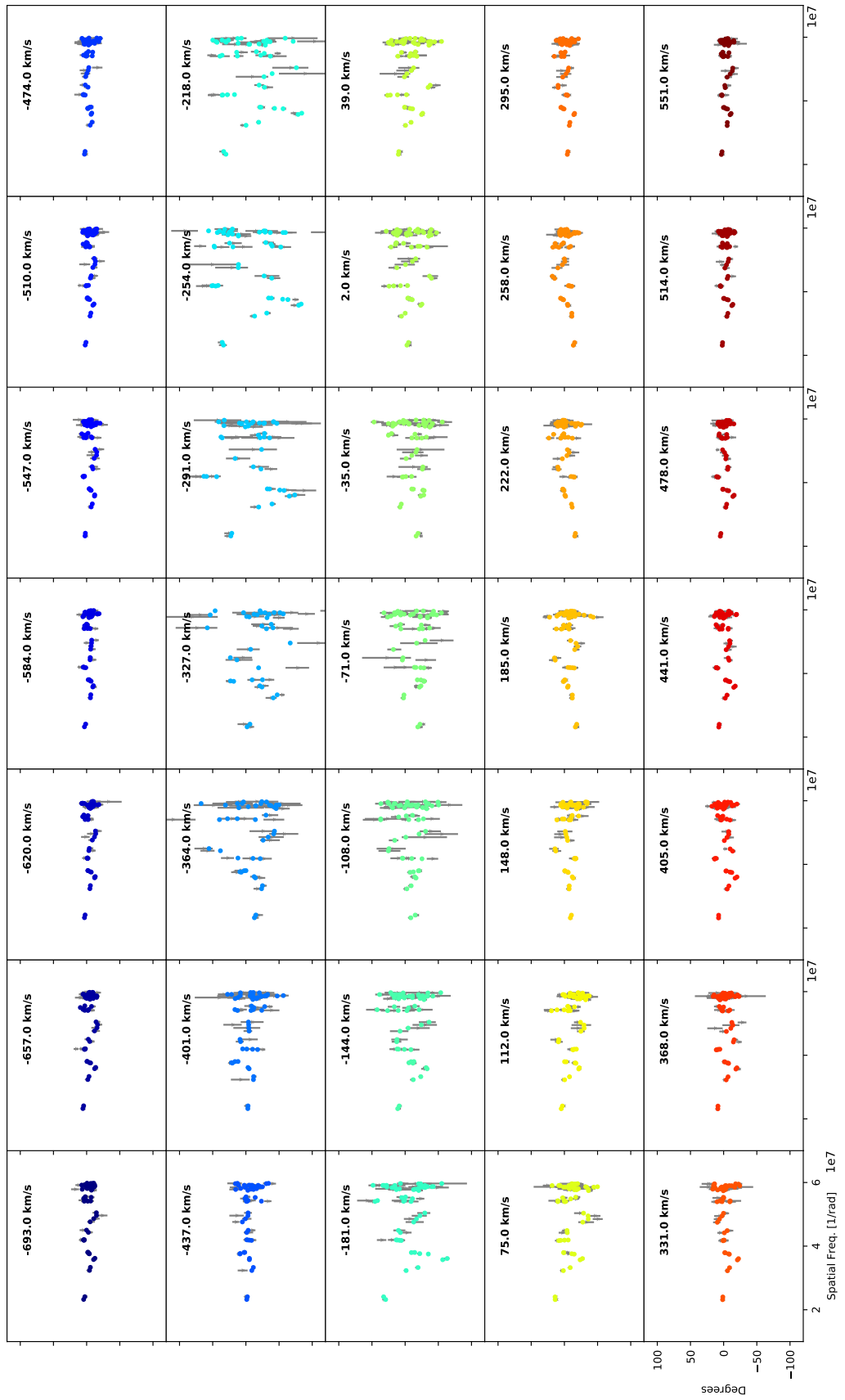
Fig. E.2. Fit to the observed closure phases from the interferometric aperture synthesis images across the Bry line (2016). The panels are as described in Fig. E.1.
