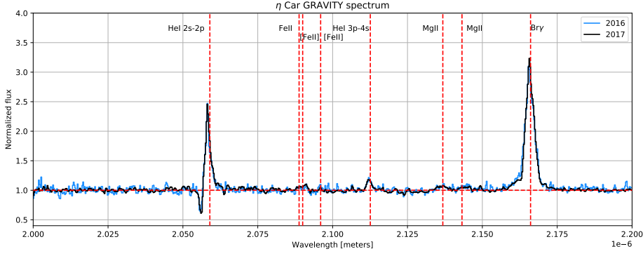
Fig. 3. 2016 (blue straight line) and 2017 (black straight line) \eta Car normalized spectra in the 2.0–2.2 \mu\text{m} bandpass. The vertical red-dashed lines indicate the spectral features identified in the spectrum.
