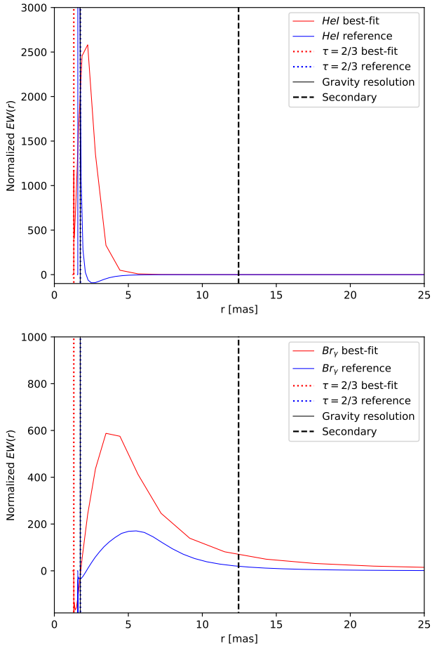
Fig. 10. CMFGEN normalized line equivalent width (EW) as a function of radius for our best-fit model and the reference one. Top and bottom panels: line-forming region as a function of radius for He I 2s-2p and Br \gamma , respectively. The red/blue dotted line corresponds the location of the \eta_A 's photosphere. The black-solid line indicates the spatial resolution limit of GRAVITY and the black-dashed line shows the projected position of \eta_B at apastron, according with the mean orbital solution presented by Teodoro et al. (2016).
