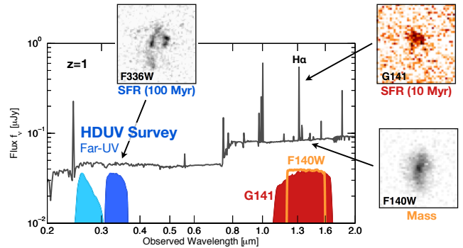
FIG. 11.— Template spectrum and images of a galaxy at z \sim 1 highlighting the power of the multi-wavelength data at HST resolution available in the HDUV survey footprint. The HDUV samples the far-UV which is sensitive to star-formation on \sim 100 Myr timescales, while the WFC3/IR grism provides resolved H \alpha images and the star-formation on \sim 10 Myr timescales. Finally, the broadband imaging in the NIR samples the rest-frame optical of galaxies out to z \sim 3 and is sensitive to the underlying mass distribution. The HDUV thus provides key insights into the internal build-up of galaxies at a spatial resolution of \sim 700 - 800 \text{ pc} out to z \sim 1 - 3 .
