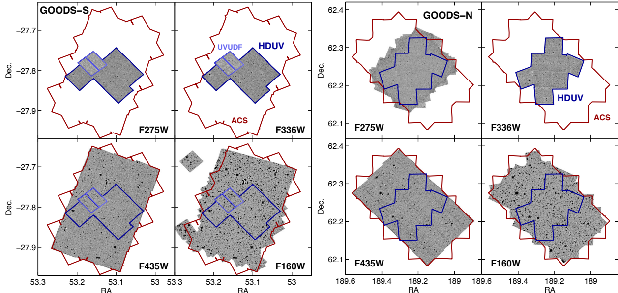
FIG. 6.— The HDUV images and their relative location to previous HST data in the GOODS-S (left) and GOODS-N (right) fields. The top panels show the WFC3/UVIS filter data in F275W and F336W of the HDUV processed images. The lower left shows the ACS F435W data from the GOODS survey and the lower right panels show the existing WFC3/IR F160W data. The dark blue outline shows the HDUV footprint. In GOODS-S the HDUV release includes the UVUDF data (pale blue outline). In GOODS-N, the HDUV survey added 4 orbits to the pre-existing F275W imaging data from the CANDELS observations. The latter are also processed and released as part of the HDUV data. Hence the F275W image in GOODS-N extends over the HDUV survey footprint. The red outline shows the full GOODS ACS coverage.
