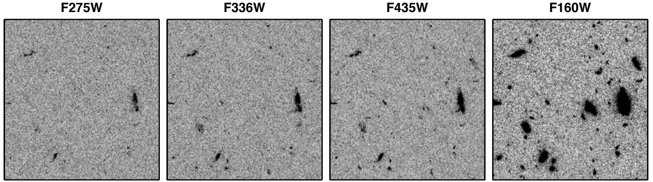
FIG. 5.— Examples of images from the HDUV (left two panels; F275W and F336W) and ancillary data (right two panels; F435W and F160W) in the GOODS-South field. The images are 0.5 arcmin on a side. Note the flat background in the WFC3/UVIS data, which was only achieved after subtraction of the sky dark. Clearly, the surface density of sources decreases to shorter wavelengths as the average galaxy exhibits a relatively red color, and sources at z \gtrsim 1.7 start to disappear from the UV imaging due to the Lyman break (see Fig 1). The low number density of UV-bright sources and the very high incidence of cosmic rays make it particularly challenging to align such UV imaging data (see §4.5).
