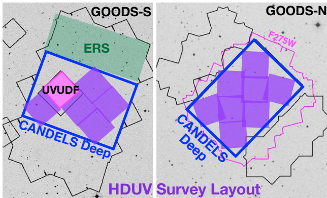
FIG. 2.— Layout of the HDUV Survey with respect to previous datasets in the GOODS-South (left) and -North (right) fields. The HDUV was designed to optimally build on and extend the pre-existing data to provide deep F275W and F336W imaging over most of the CANDELS-Deep area (blue outline). In GOODS-S, the HDUV covers 5 pointings around the UVUDF (pink). A larger area (8 pointings) could be covered in GOODS-N making use of the CVZ and building on the limited, pre-existing F275W imaging from the CANDELS survey. When combined with the UVUDF, the total area of WFC3/UVIS imaging in these two fields spans \sim 100 arcmin 2 to a depth of 10 and 8 orbits or deeper in the two filters, respectively, reaching 27.5–28.0 mag at 5\sigma . The data release described here includes the F275W images from the CANDELS survey in GOODS-N.
