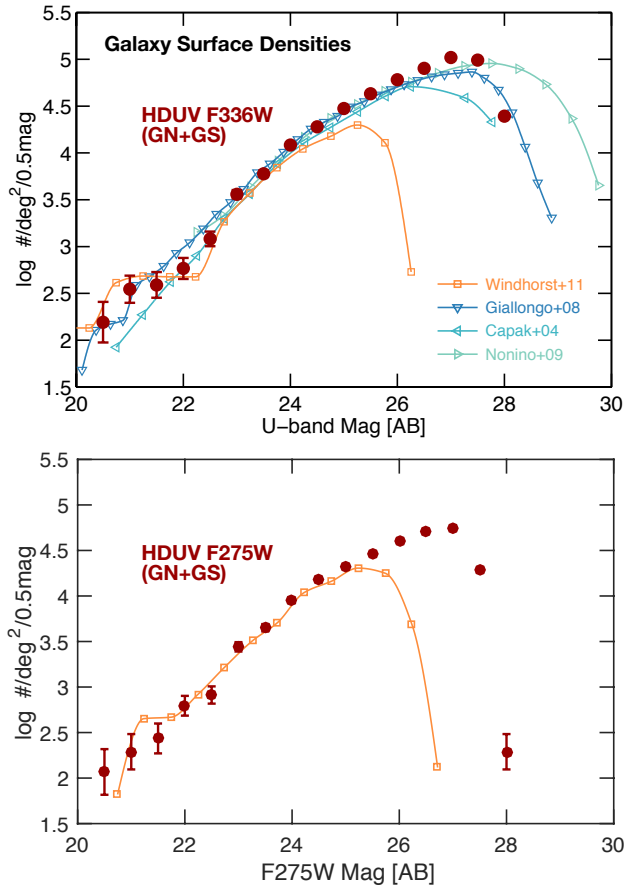
FIG. 10.— Comparison of the U/F336W-band (top) and F275W (bottom) surface densities of sources measured with different surveys. The surface densities based on the HDUV F336W and F275W filter imaging are shown as dark red dots (with Poisson errorbars). The orange squares and lines represent the F336W/F275W surface density measured in the ERS data (Windhorst et al. 2011), while all the other lines correspond to ground-based U-band imaging surveys covering larger areas (Nonino et al. 2009; Giallongo et al. 2008; Capak et al. 2004). The latter cover slightly longer central wavelengths ( \lambda_c \sim 3600 - 3800 \text{ \AA} ) compared to \lambda_c = 3350 \text{ \AA} of F336W, and they all have a much wider PSF ( > 8\times ). The curves turn over at faint magnitudes since no completeness corrections have been applied. Magnitudes correspond to total fluxes.
