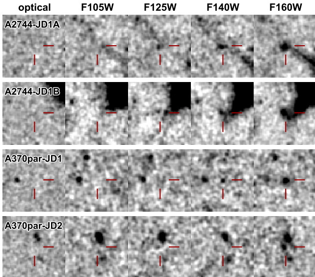
FIG. 1.— Stamps of the only four z \sim 10 galaxy candidates with S/N > 6 in the twelve HFF cluster+parallel fields. From left to right these show a stack of all the available optical ACS images, and the WFC3/IR Y_{105} , J_{125} , JH_{140} , and H_{160} images. The images are oriented North up and they span 3'' on a side. z \sim 10 candidates are identified based on J_{125} - H_{160} > 1.2 colors and non-detections at shorter wavelengths.
