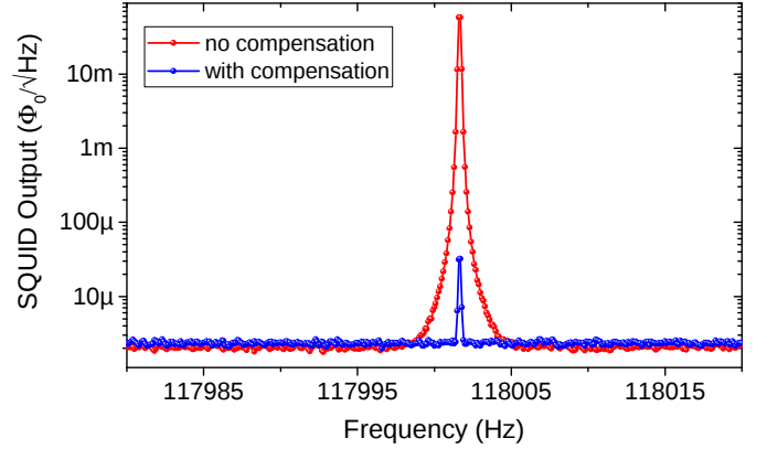
Figure 5: Demonstration of the reduction of crosstalk by compensating the RF pulse. The measured flux crosstalk has been reduced from 26 \text{ m}\Phi_0 without compensation to less than 15 \text{ }\mu\Phi_0 with compensation.
