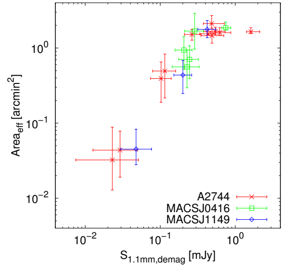
Fig. 9. Median effective area as a function of demagnified integrated flux density for A2744 (red crosses), MACSJ0416 (green squares), and MACSJ1149 (blue diamonds). Median values are obtained combining all models for each cluster field. Error bars correspond to the 16th and 84th percentiles. For comparing uncertainty values, both axes cover the same interval in order of magnitude. Within the errors, both demagnified flux densities and effective areas span around 2.5 orders of magnitude.
