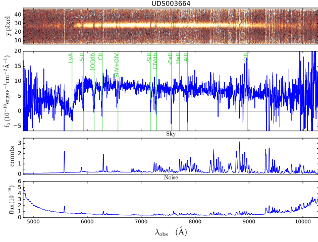
Fig. 12. From top to bottom, the 2-dimensional spectrum, 1-dimensional extracted spectrum, sky counts and rms noise of target VANDELS-UDS-003664. This object has an H-band magnitude of 23.1 and was selected in the category SFG. It was assigned a z_{spec} = 3.703 and Flag 4. The main spectral features identified (the Ly \alpha absorption and several interstellar absorption lines) are indicated in the 1-D spectrum.
