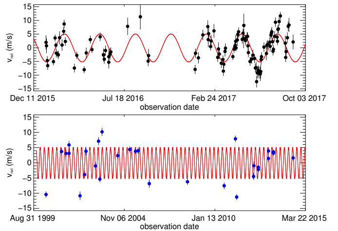
Fig. 1. Radial velocities obtained with CARMENES (upper panel) and HIRES/Keck (lower panel). The orbital motion according to the adopted solution is overplotted in red (see Sect. 4).
