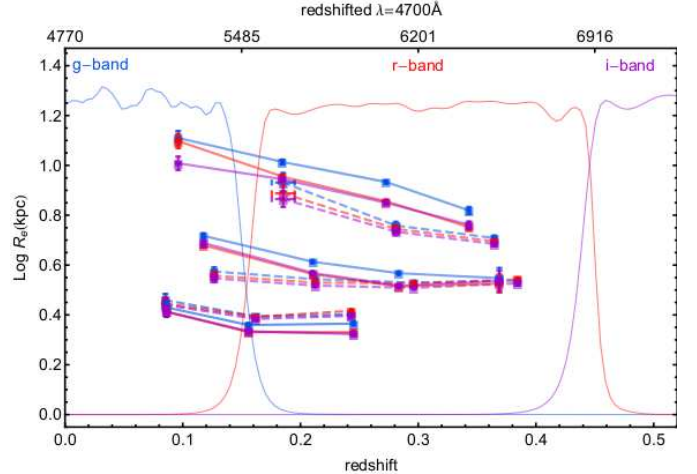
Figure D1. Size-redshift relation for the spheroids (solid lines) in the mass bins \text{Log } M_*/M_\odot = 10.4, 10.8, 11.2 and disc dominated galaxies in the mass bins \text{Log } M_*/M_\odot = 10.0, 10.4, 10.8 (dashed lines) in g (blue), r (red) and i (purple) bands.
