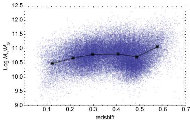
Figure 17. Mass vs. redshift plot for the spheroids sample. Overplotted to the individual galaxy values, we show the mean and standard deviation of the mean of the sample (error bars are comparable to the size of the boxes). Note that the steepening of the z \sim 0.6 bin is due to the mass incompleteness of this bin. In the lowest z bin ( z \sim 0.1 ), the sample suffers some volume incompleteness (see discussion in Sect. 2), which produces the mean mass in the bin to be biased toward less massive systems.
