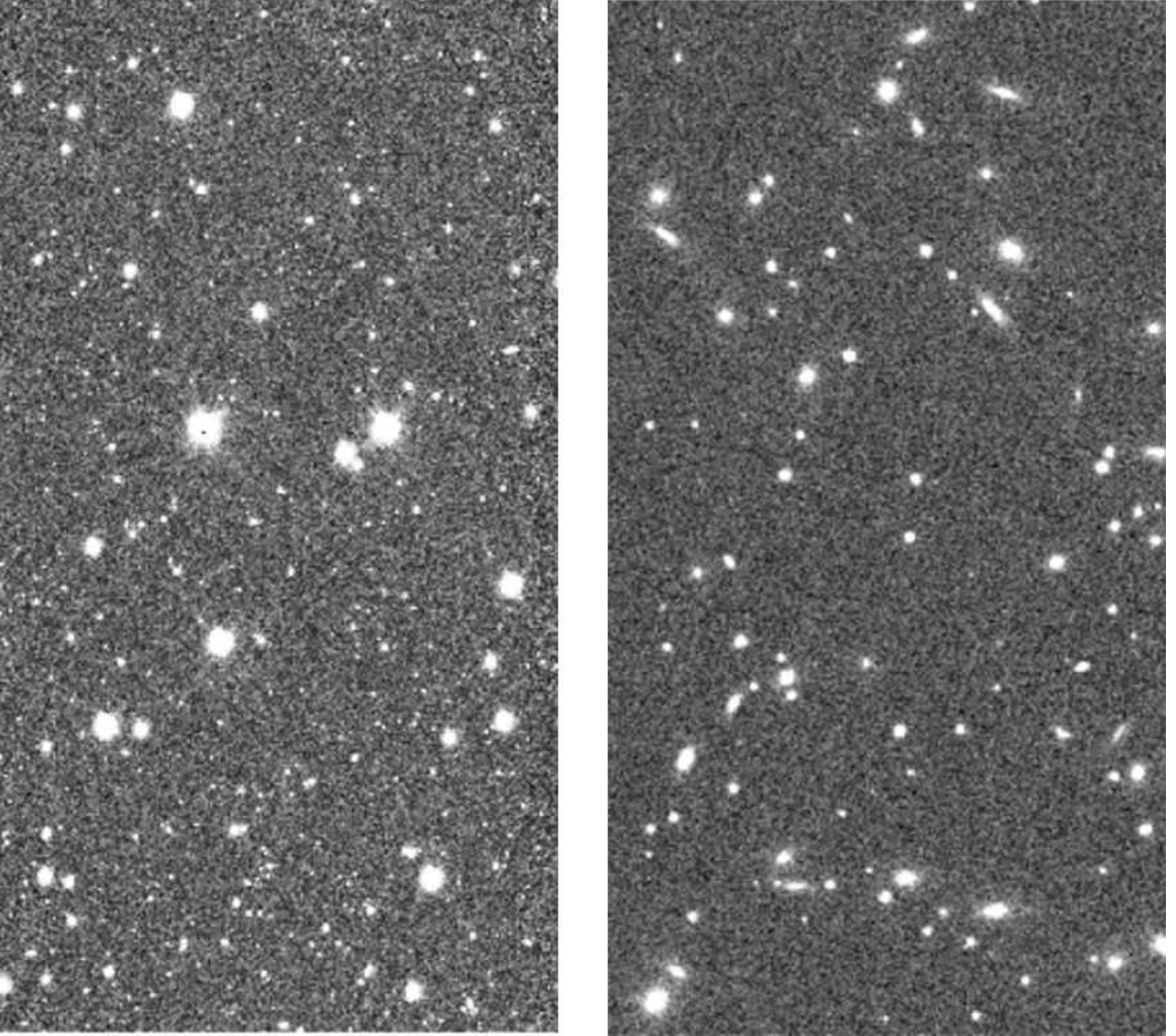
Figure 11. A real KiDS image (left) vs. a mock image with simulated galaxies (right). Seeing FWHM are 0.69 and 0.66 for real and mock images respectively.
