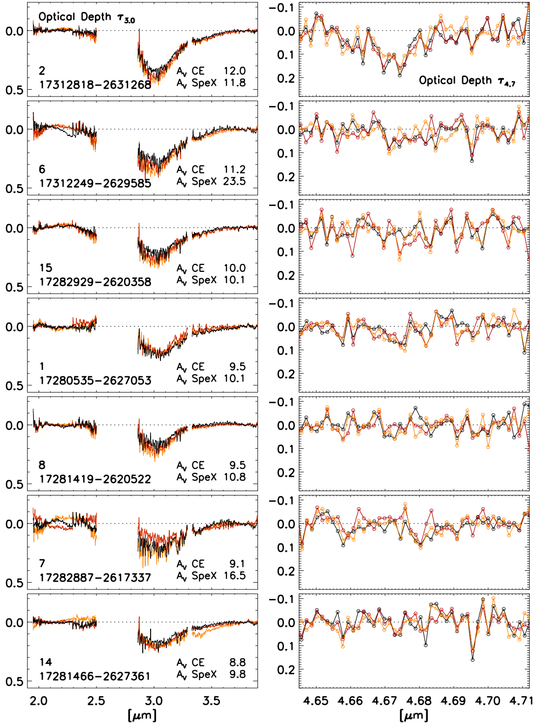
Fig. 2. Optical depth spectra of water ( 3.0\mu\text{m} ; left column) and CO ice ( 4.672\mu\text{m} ; right column) toward the seven sources where water ice was positively detected in the observations by SpeX spectrograph at the IRTF. The numbering of the sources in Fig. 1 and Table 1 is shown at the bottom left of the water-ice panels with the 2MASS IDs. The CO ice spectra were obtained by NIRSPEC spectrograph at Keck II. The whole SpeX spectra including negative detections are compiled in Fig. A.1 in Appendix A. Black, red, and orange plots, are the spectra in which photospheric features are removed by referring to the best, the second best, and the third best matching M -type template stars. The visual extinctions based on the color excess ( A_V CE; Román-Zúñiga et al. 2010) and on the template matching with the IRTF Spectral Library ( A_V SpeX; Rayner et al. 2009) are shown at the bottom right of the water ice spectra.
