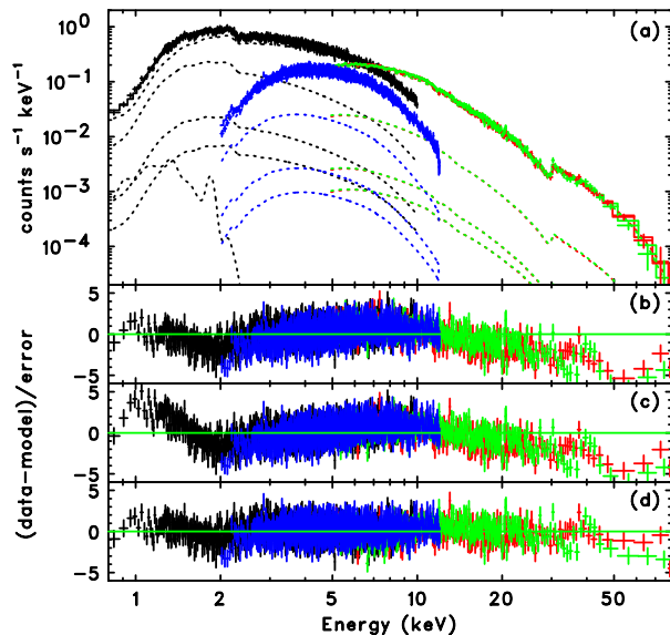
Fig. 2. Wide-band spectra of G21.5–0.9 obtained with the SXI (black; 0.8–10.0 keV), HX11 (red; 5.0–80.0 keV), HX12 (green; 5.0–80.0 keV) and the SXS (blue; 2.0–12.0 keV). The data is rebinned only for plotting purposes. The best-fit model (composite+Broken PL; see text and table 2) is overlaid with the solid lines in panel (a). The dotted lines indicate all the additive components in the model. Panels (b), (c), and (d) show residuals from the single PL, composite+PL and composite+Broken PL models, respectively.
