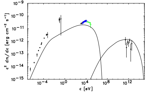
Fig. 5. Same as figure 4 but with the Case 2 model curves.
