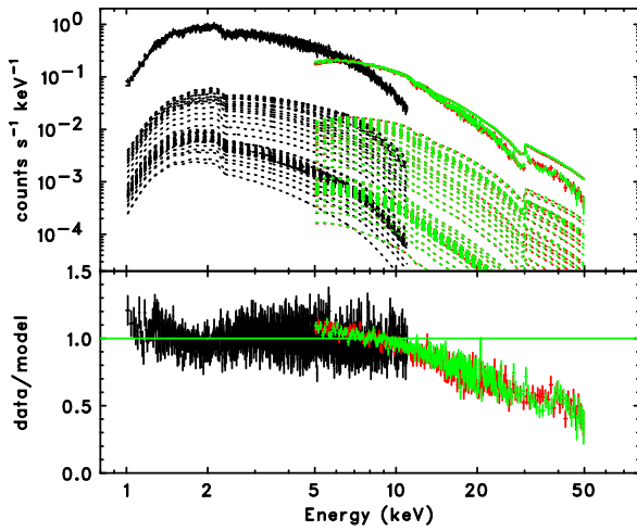
Fig. 3. The SXI (black) and HXI1/2 data (red and green) fitted with the composite+PL model accounting for the spatially resolved spectroscopic study of the SNR with Chandra (Guest & Safi-Harb 2018; see also Matheson & Safi-Harb 2005). The individual components contributing to the fitted spectrum are shown as dashed lines. The bottom panel shows the data-to-model ratios and illustrates that this model does not reproduce the spectral shape obtained with the HXI.
